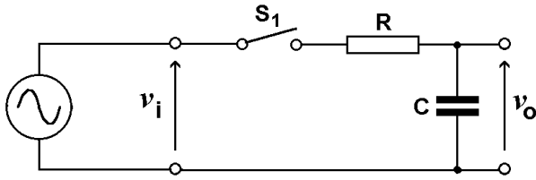
Figure 1, Gated Integrator
