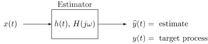
FIGURE 11.5 CT LTI filter for linear MMSE estimation.
