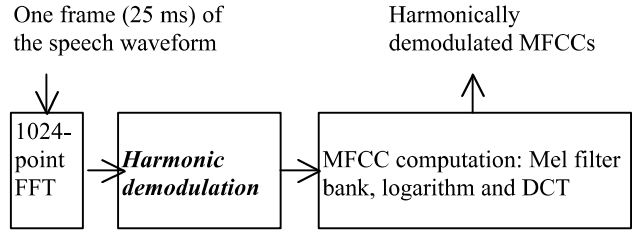
Figure 6: Block diagram of the harmonically demodulated MFCCs.
