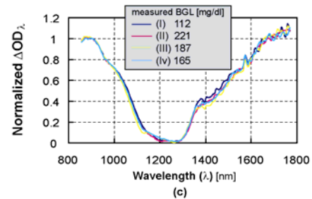
Fig. 5: (a) An example of the time course of the measured and predicted BGL values before and after oral administration of glucose solution indicated by the arrow, (b) averaged spectrum of optical density ( \Delta OD_\lambda ) obtained from 4 consecutive cardiac beats at a point (I) in (a) calculated from the light intensities ( I_\lambda and \Delta I_\lambda ), and (c) \Delta OD_\lambda spectra which was normalised using the value of the \Delta OD_\lambda at 900 nm as 1.0 together with the minimum value of \Delta OD_\lambda as 0 in each calculated spectrum obtained at the points (I), (II), (III) and (IV) in (a). The time course was obtained from the analysis based on method (B).
