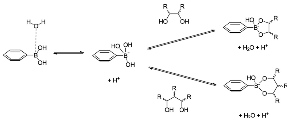
Scheme 5 – Interaction of phenylboronic with 1,2- and 1,3-diols to form cyclic boronate esters [46].
