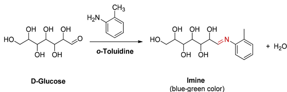
Scheme 1 – Reaction of D-glucose and o-toluidine.
