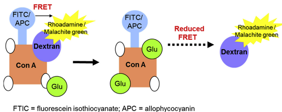
Fig. 4 – Principle of fluorescence resonance energy transfer (FRET) from Concanavalin A (Con A) to dextran by adding glucose [36].
