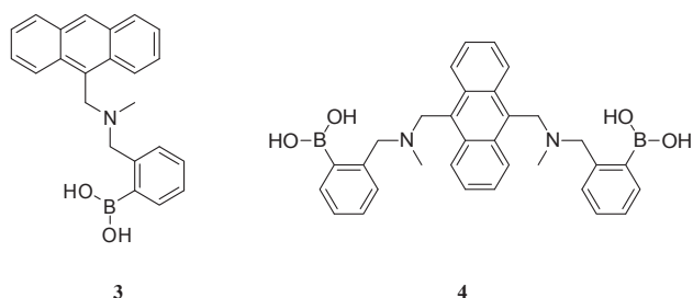
Fig. 6 – Structures of N-methyl-o-(aminomethyl)phenylboronic acid (3) and bis-boronic acid (4).
