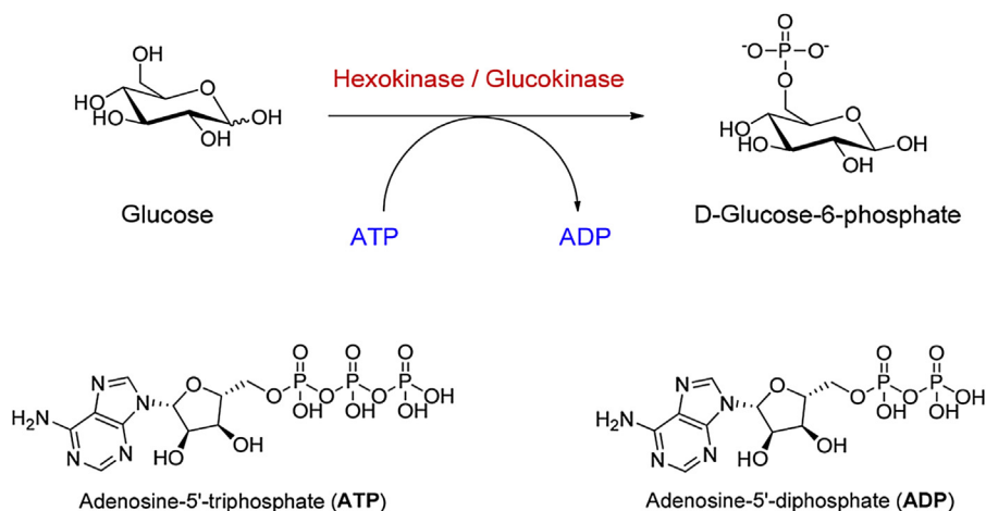
Scheme 4 – D-Glucose catalyzed by hexokinase forms D-glucose-6-phosphate.
