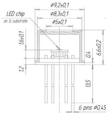
Infrared LED 16-TO-5
