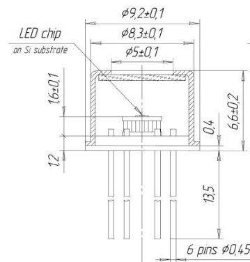
Infrared LED 13-TO-5
