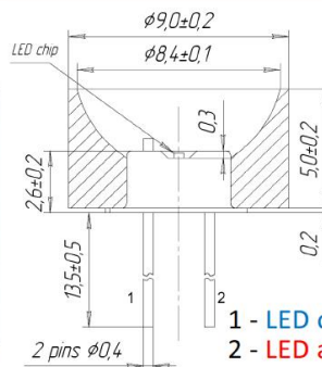
Infrared LED 10-TO-18R Infrared LED 10-TO-18RW
