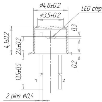
Infrared LED 19-TO-18
