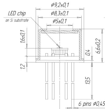
Infrared LED 19-TO-5
