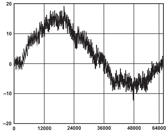
TPC 1. Typical INL Performance at 15 MSPS
