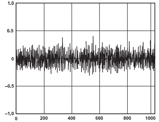
TPC 5. Typical DNL Performance at 30 MSPS
