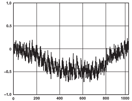
TPC 4. Typical INL Performance at 30 MSPS
