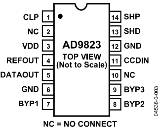
Figure 2. Pin Configurations
