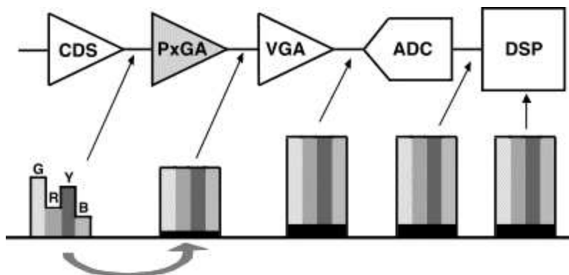
Figure 3: Signal path with PxGA^{TM}
