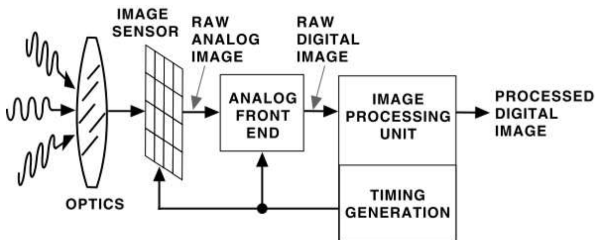
Figure 1: Block diagram of a typical imaging application
