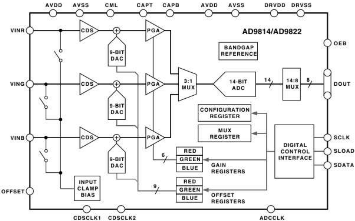
Figure 5: Block diagram of the AD9814/9822
