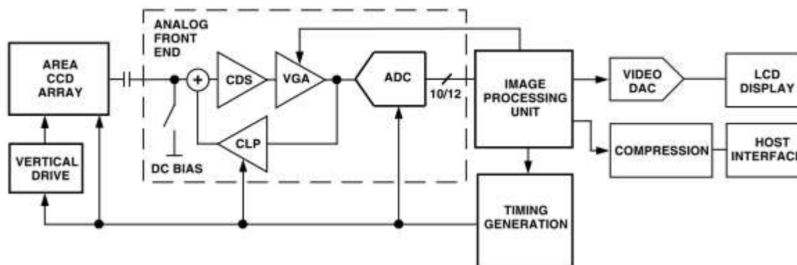
Figure 2: Simplified block diagram of a digital camera
