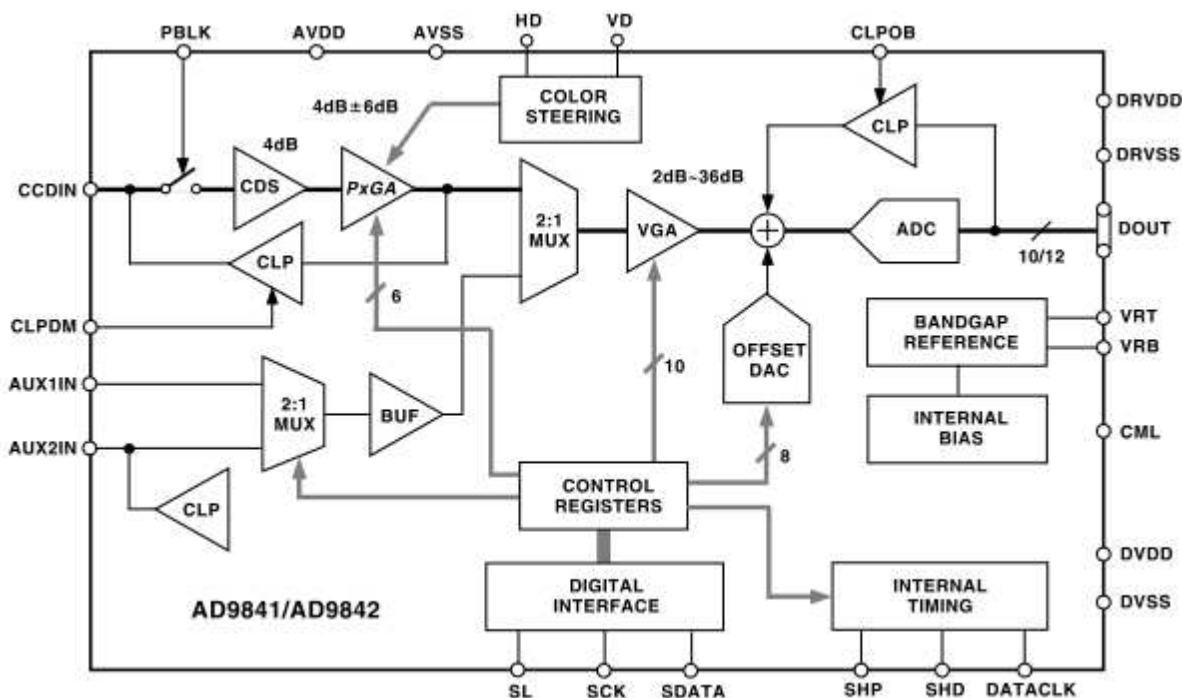
Figure 4: Block diagram of the AD9841/9842
