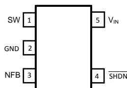
5-lead SOT-23 Package Top View
