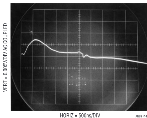
Figure 14. Time and Amplitude Expansion of Figure 13 More Clearly Shows Residual High Frequency Content with Slew Limiting Employed
