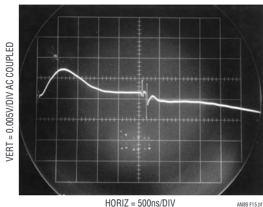
Figure 15. Same Test Conditions as Previous Figure, Except Slew Limiting Is Disabled. High Frequency Harmonic Content Rises \approx 10. Leave that Slew Limiting in There!
