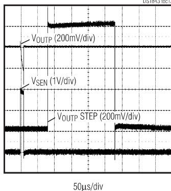
SINGLE-ENDED STEP RECOVERY, 1V OUTPUT STEP ( V_{INP} = 1\text{V} )
