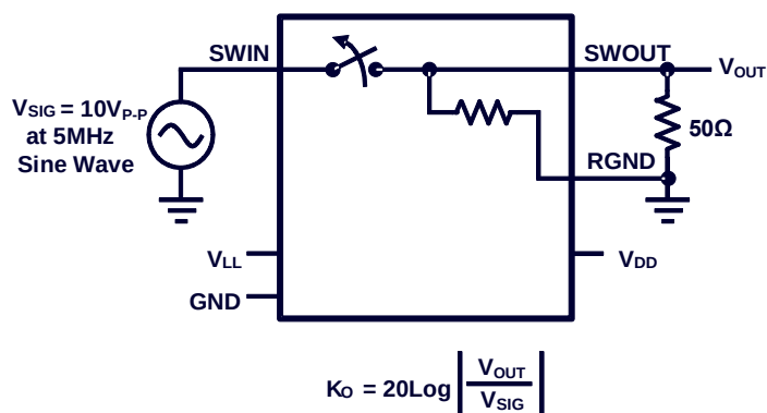
Figure 5: Test Circuit 4
