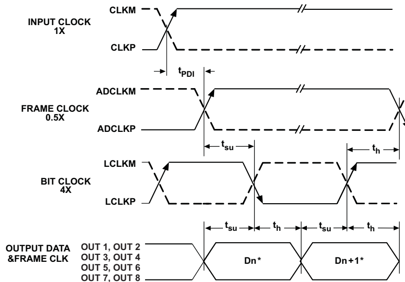
Figure 2. LVDS Timing
