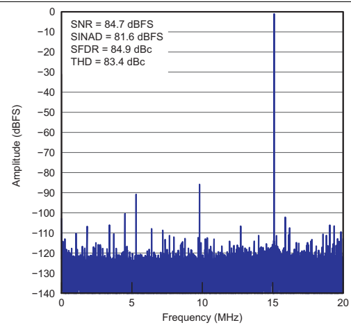
Figure 6. FFT for 15-MHz Input Signal, f_s = 40 \text{ MSPS}
