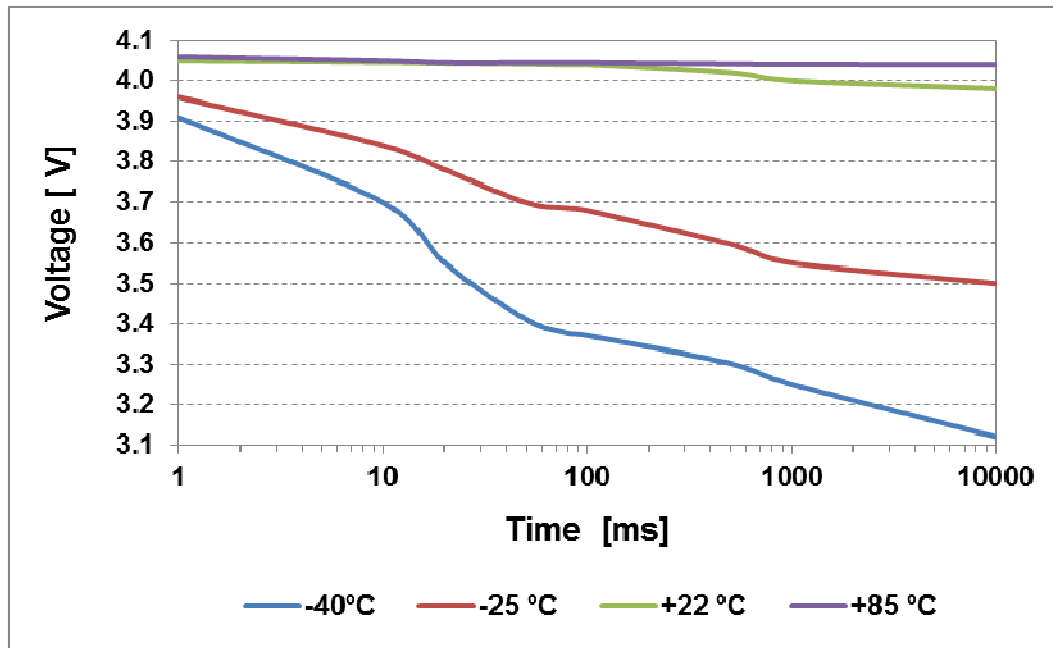
Voltage curves @ 750 mA, 10 sec pulse
