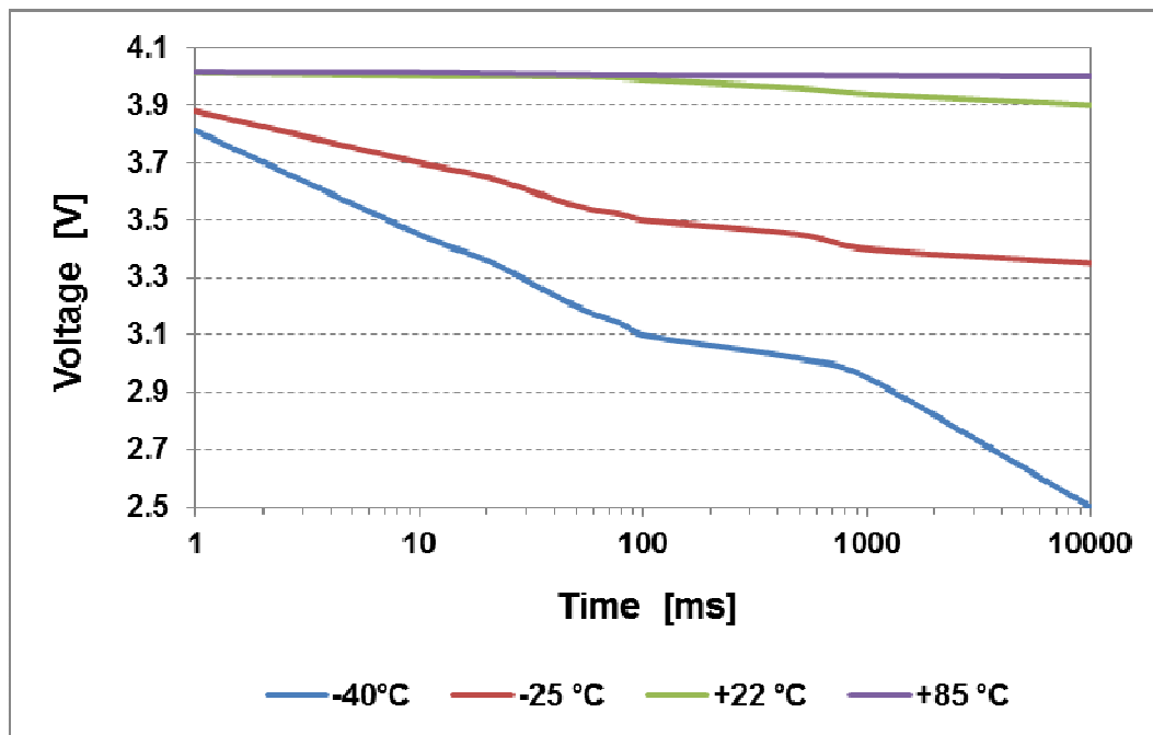
Voltage curves @ 1200 mA, 10 sec pulse
