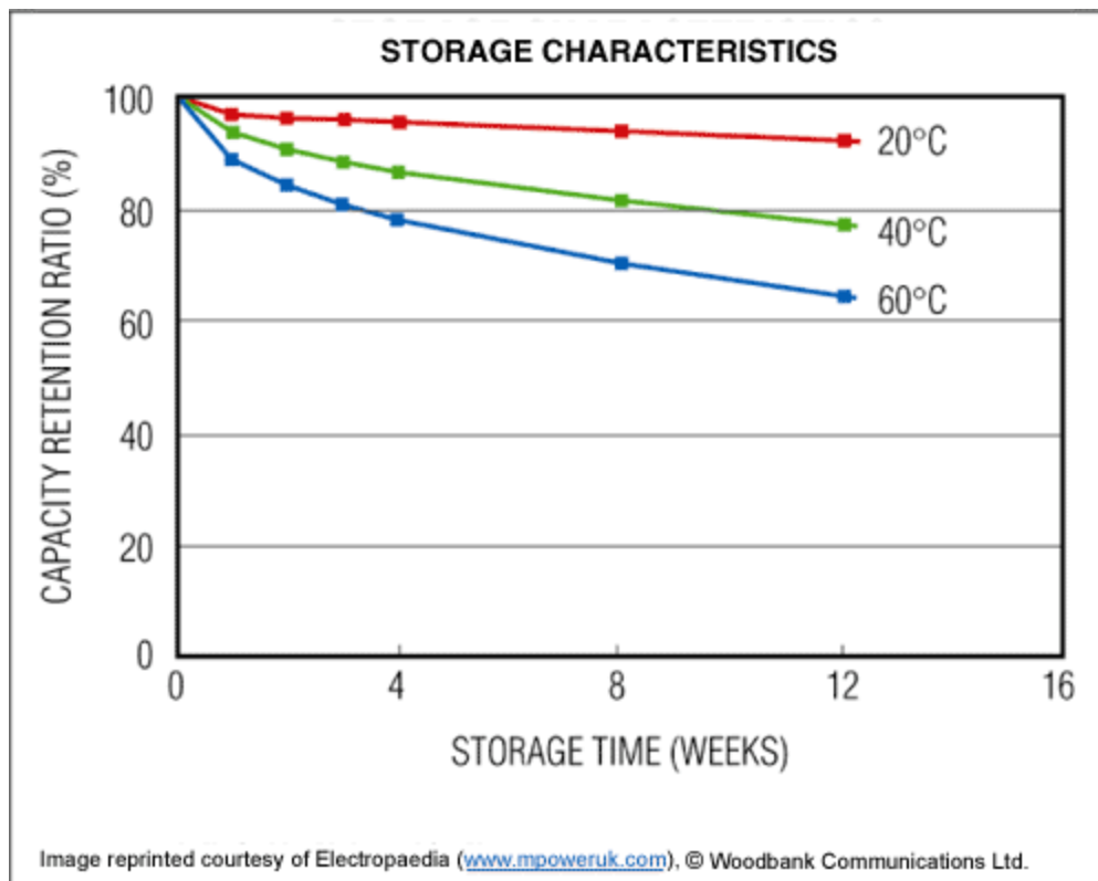
Figure 3. Self-discharge of Li-ion batteries.
