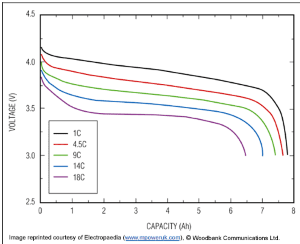
Figure 5. Battery-discharge curve.
