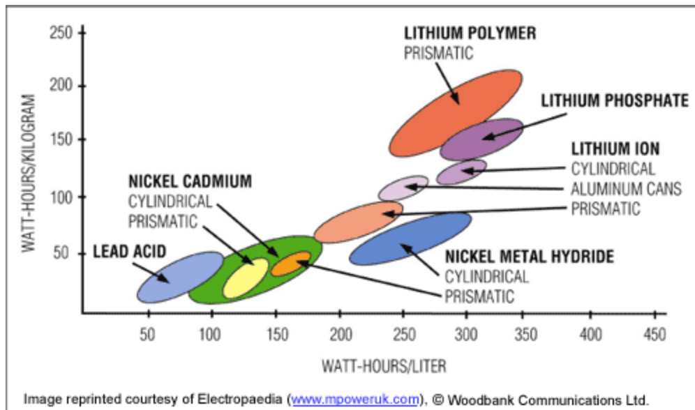
Figure 1. The energy densities of various battery types.
