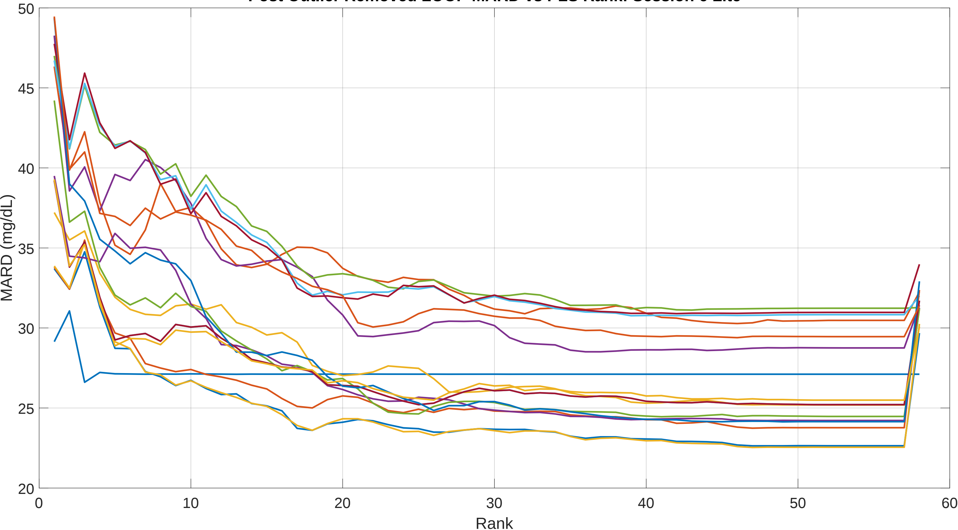
Post Outlier Removed LOOP MARD vs PLS Rank: Session 6 Lite
