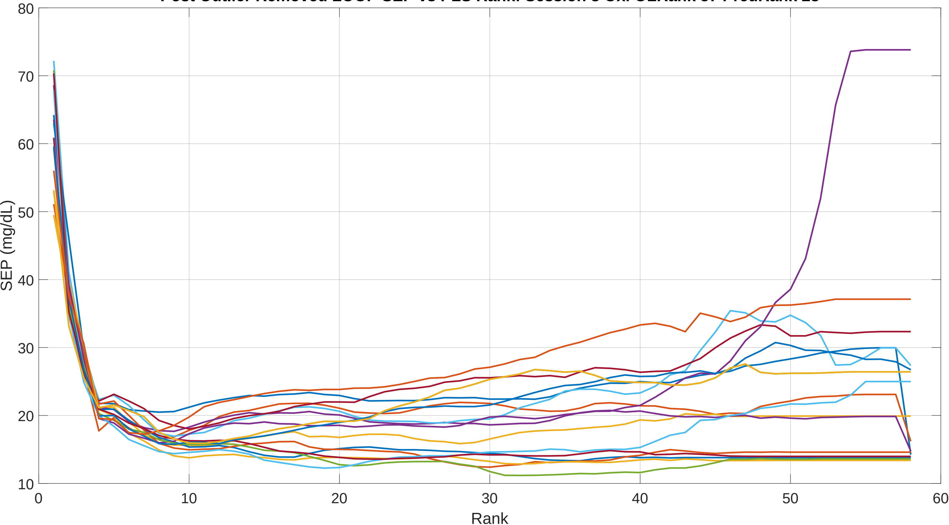
Post Outlier Removed LOOP SEP vs PLS Rank: Session 8 Oxi OLRank 57 PredRank 28
