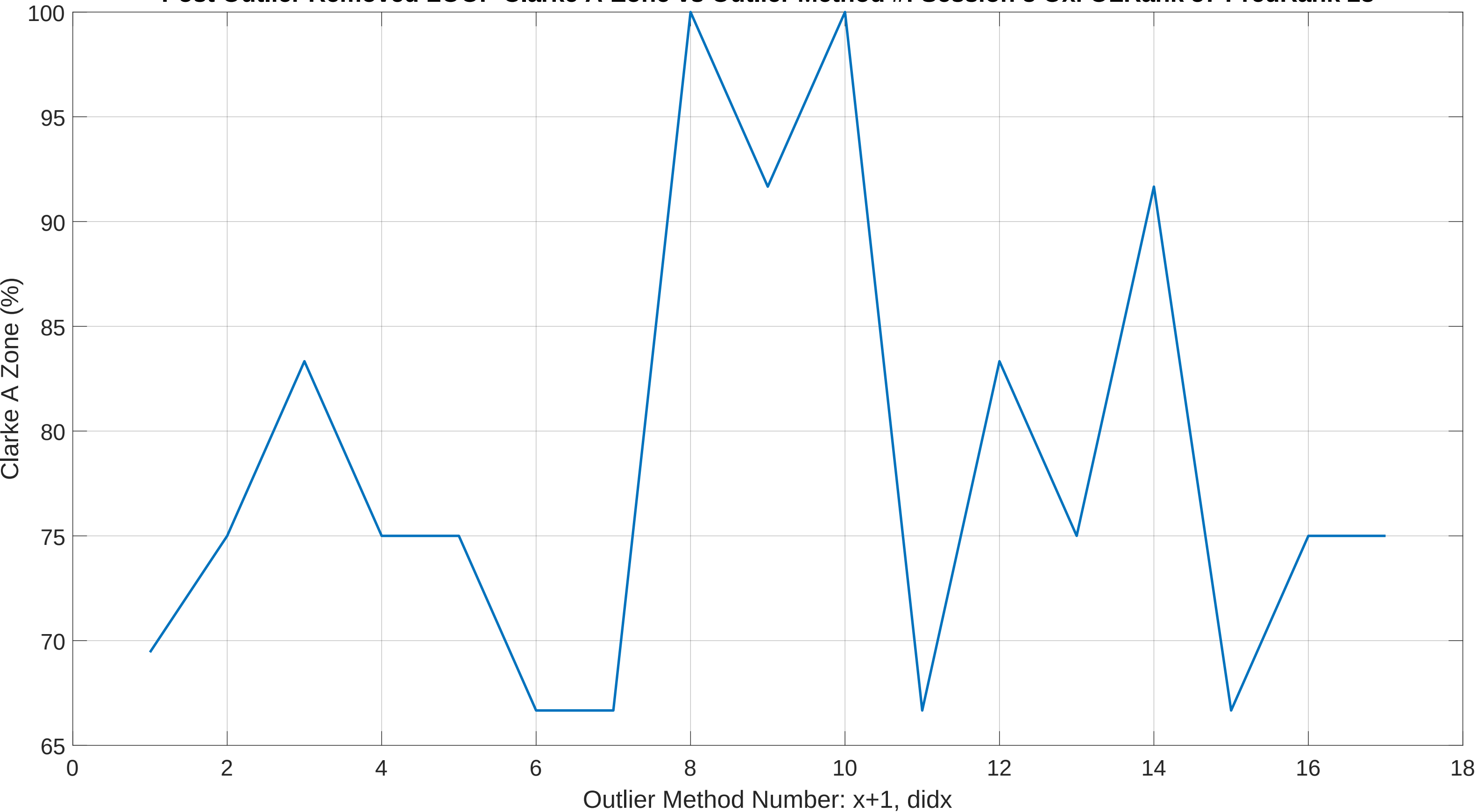
Post Outlier Removed LOOP Clarke A-Zone vs Outlier Method #: Session 8 Oxi OLRank 57 PredRank 28
