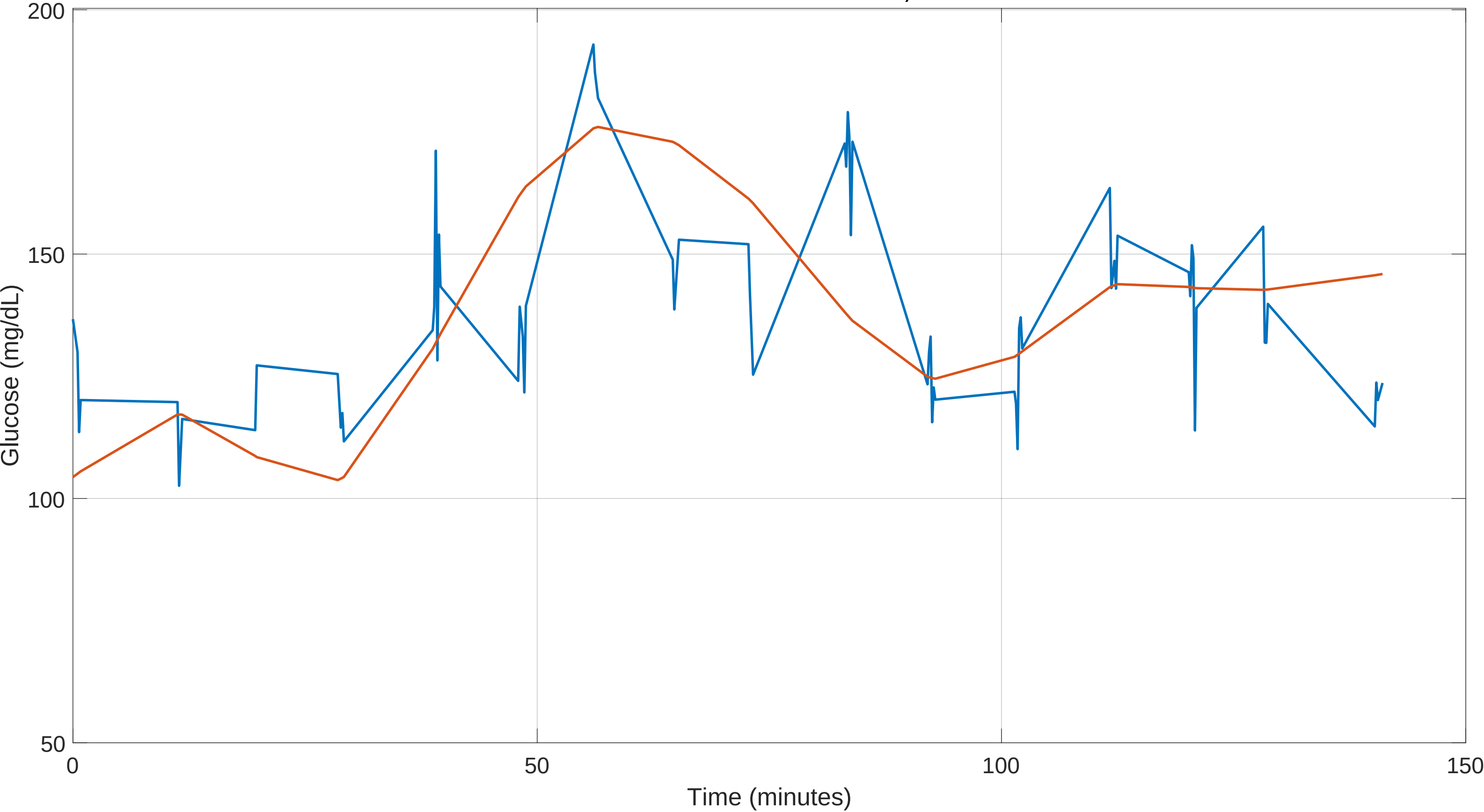
Post Outlier Removed LOOP vs Time: Outliers not in Predictions, Session 7 Verio OLRank 57 PredRank 28
