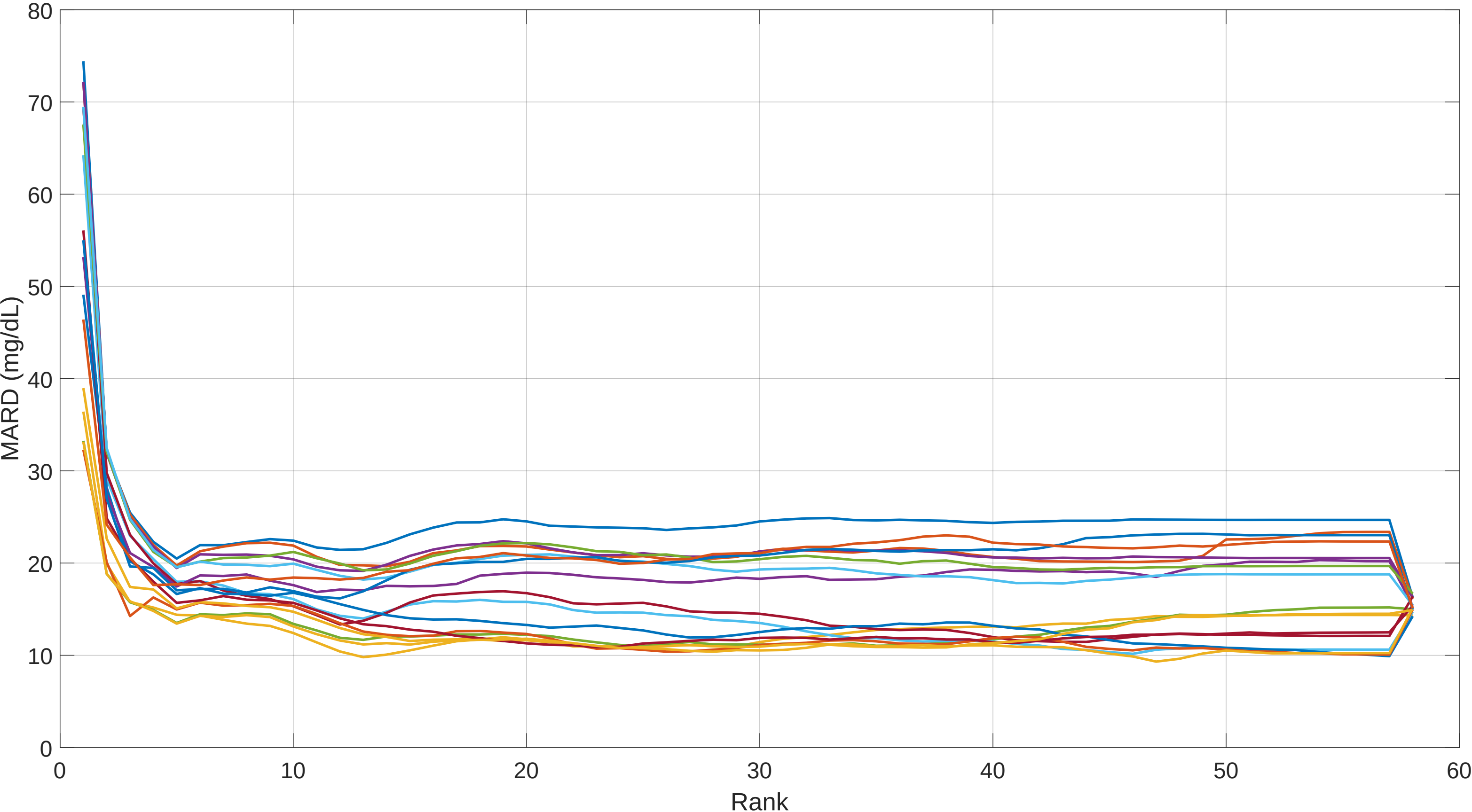
Post Outlier Removed LOOP MARD vs PLS Rank: Session 7 Verio OLRank 57 PredRank 28
