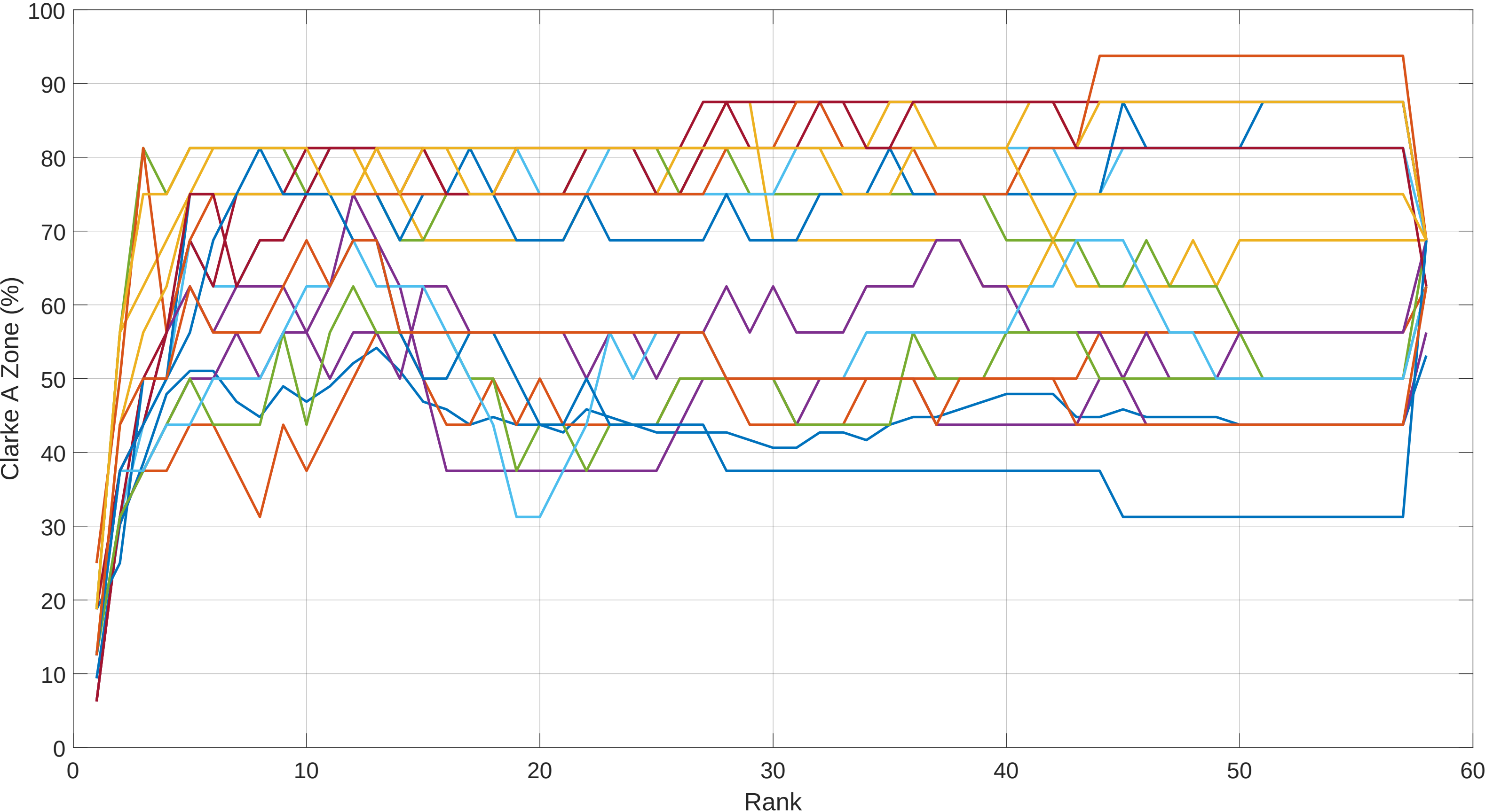
Post Outlier Removed LOOP Clarke A-Zone vs PLS Rank: Session 7 Verio OLRank 57 PredRank 28
