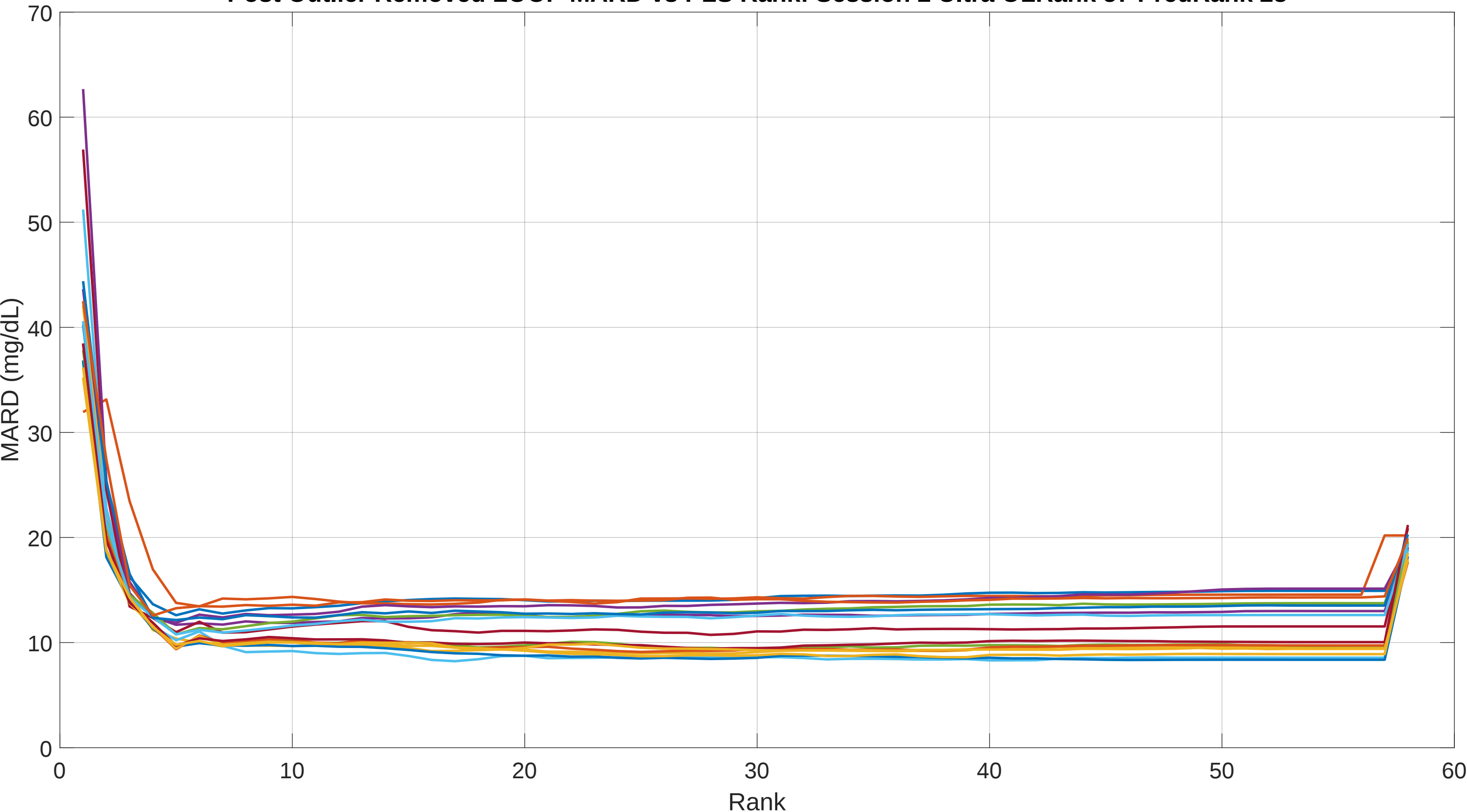
Post Outlier Removed LOOP MARD vs PLS Rank: Session 2 Ultra OLRank 57 PredRank 28
