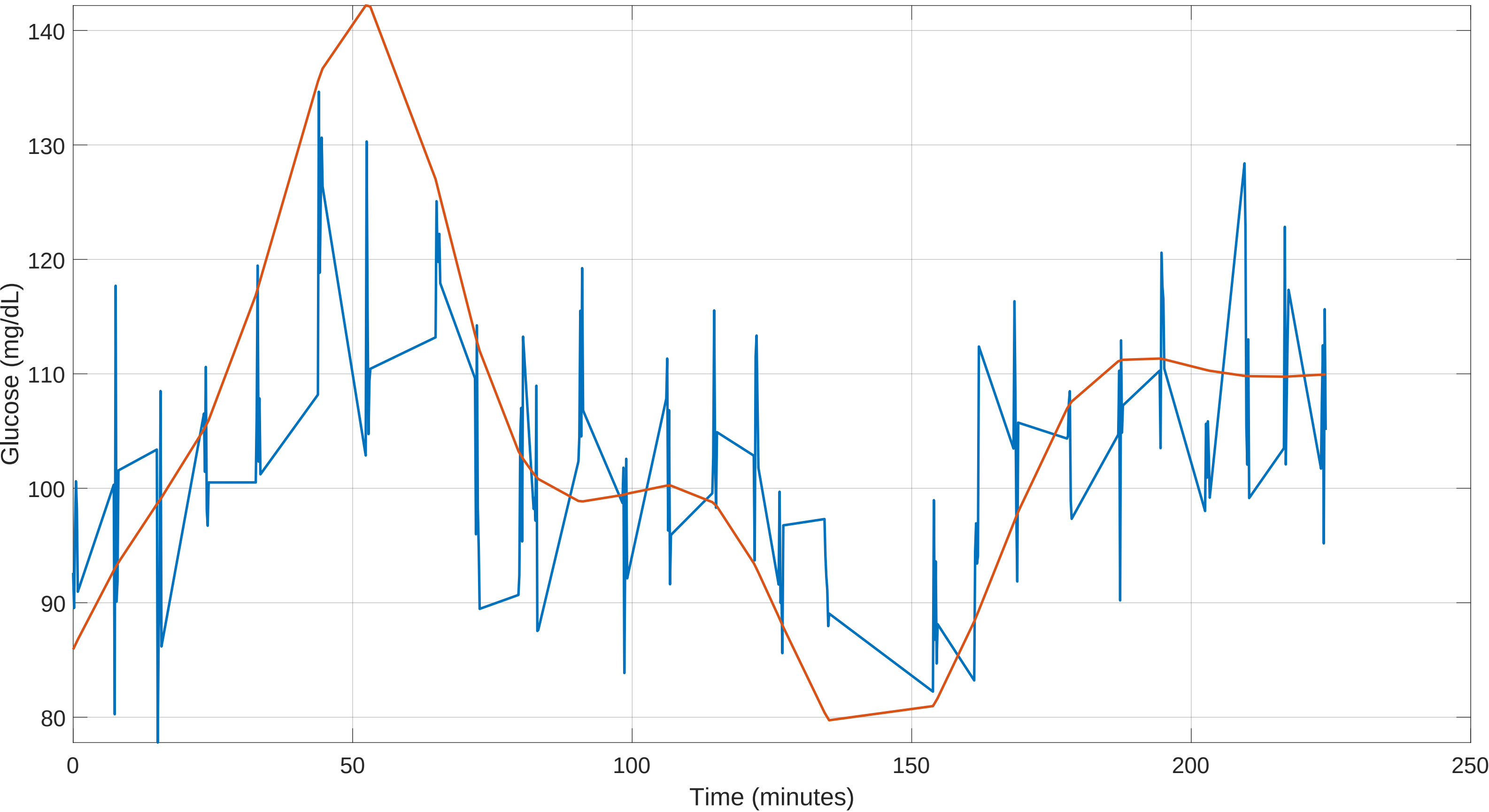
Post Outlier Removed LOOP vs Time: Outliers in Predictions, Session 1 Ultra OLRank 57 PredRank 28
