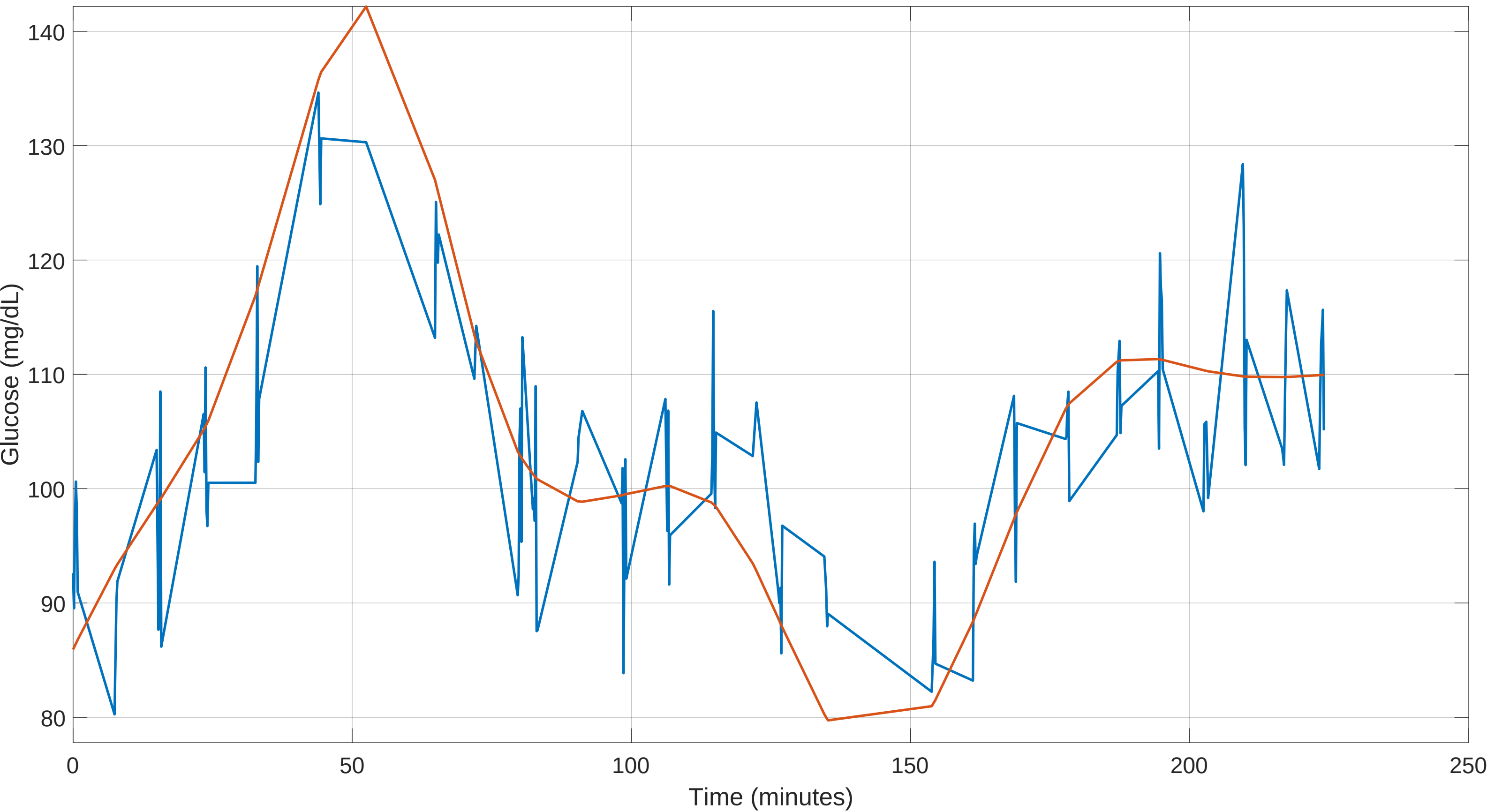
Post Outlier Removed LOOP vs Time: Outliers not in Predictions, Session 1 Ultra OLRank 57 PredRank 28
