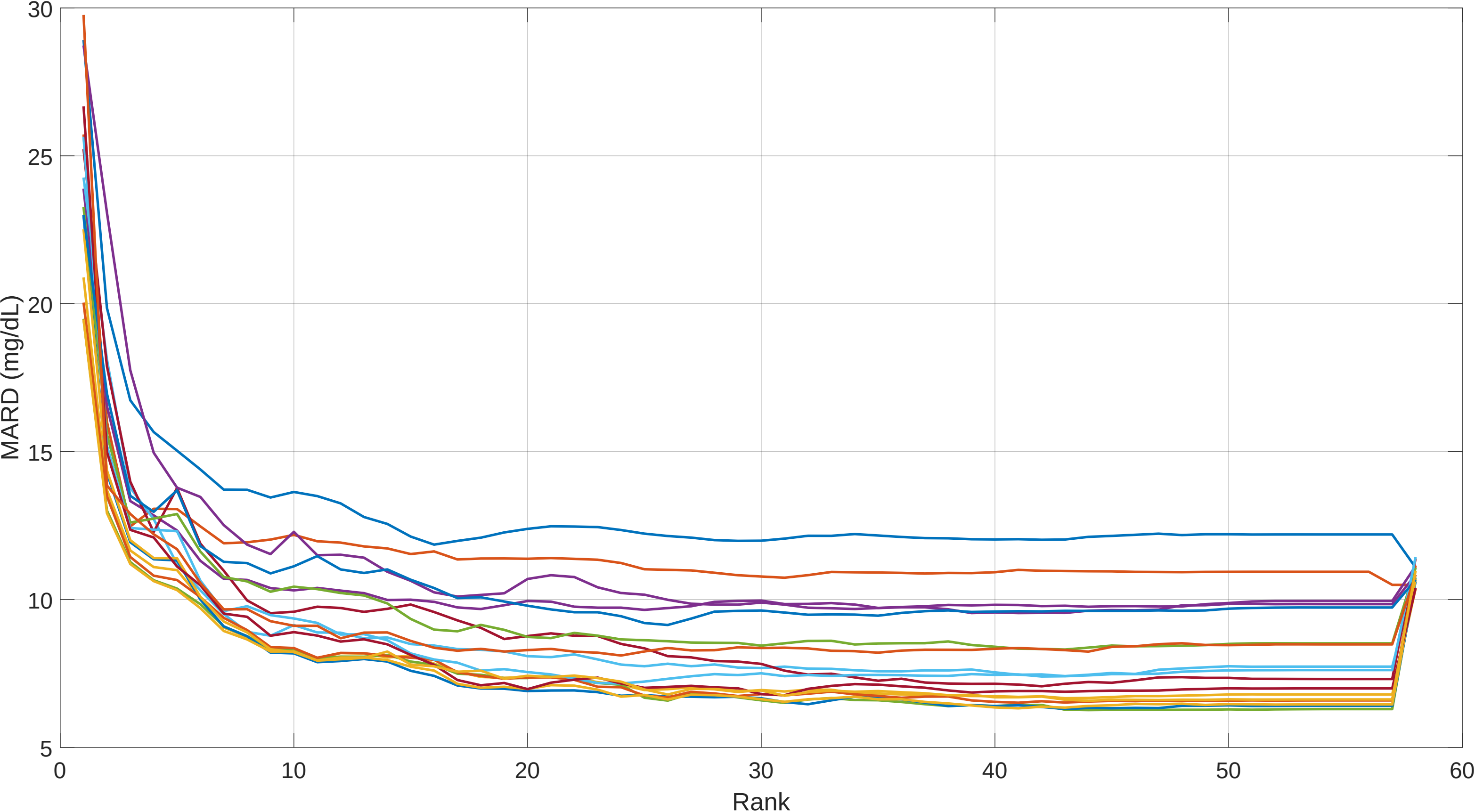
Post Outlier Removed LOOP MARD vs PLS Rank: Session 1 Ultra OLRank 57 PredRank 28
