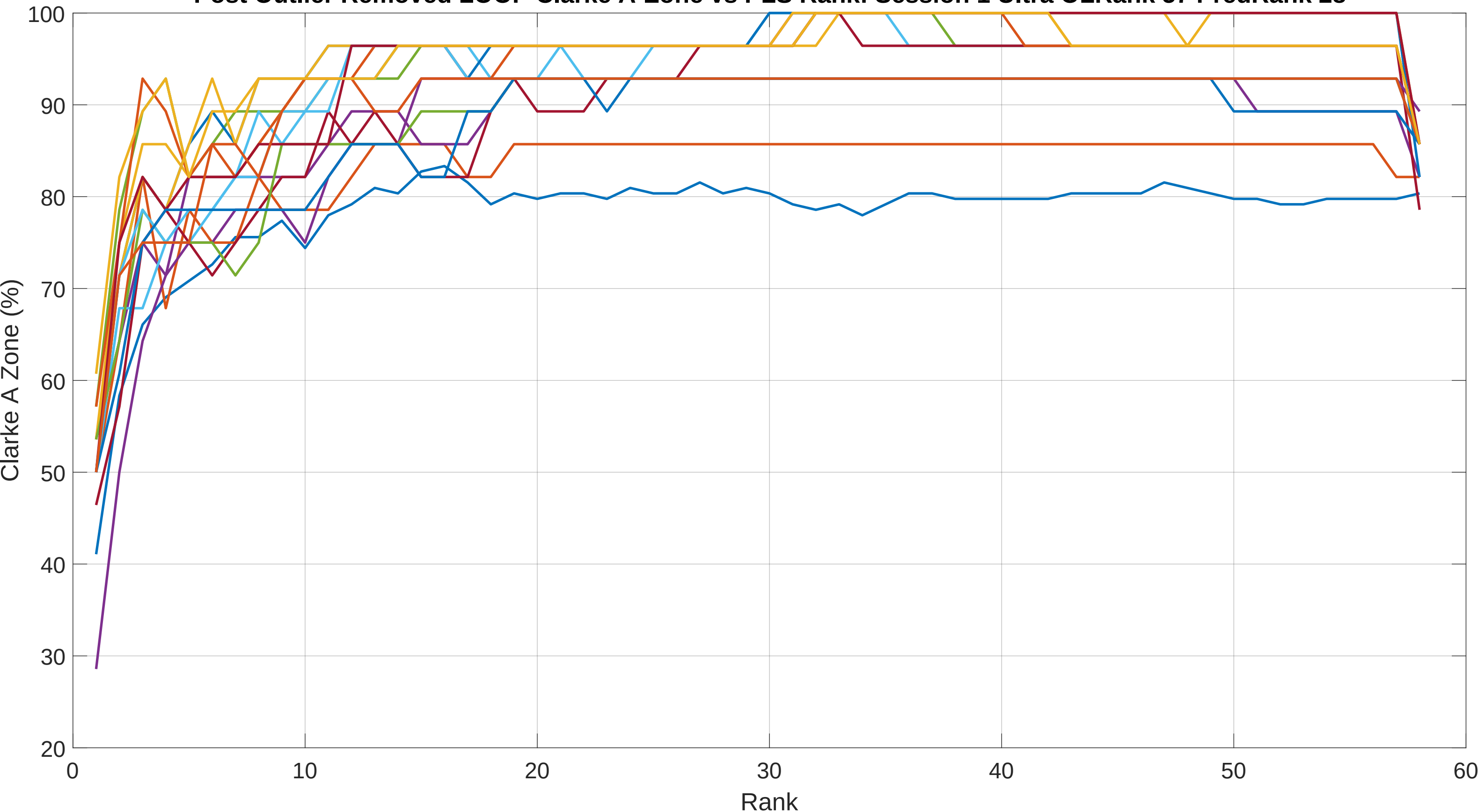
Post Outlier Removed LOOP Clarke A-Zone vs PLS Rank: Session 1 Ultra OLRank 57 PredRank 28
