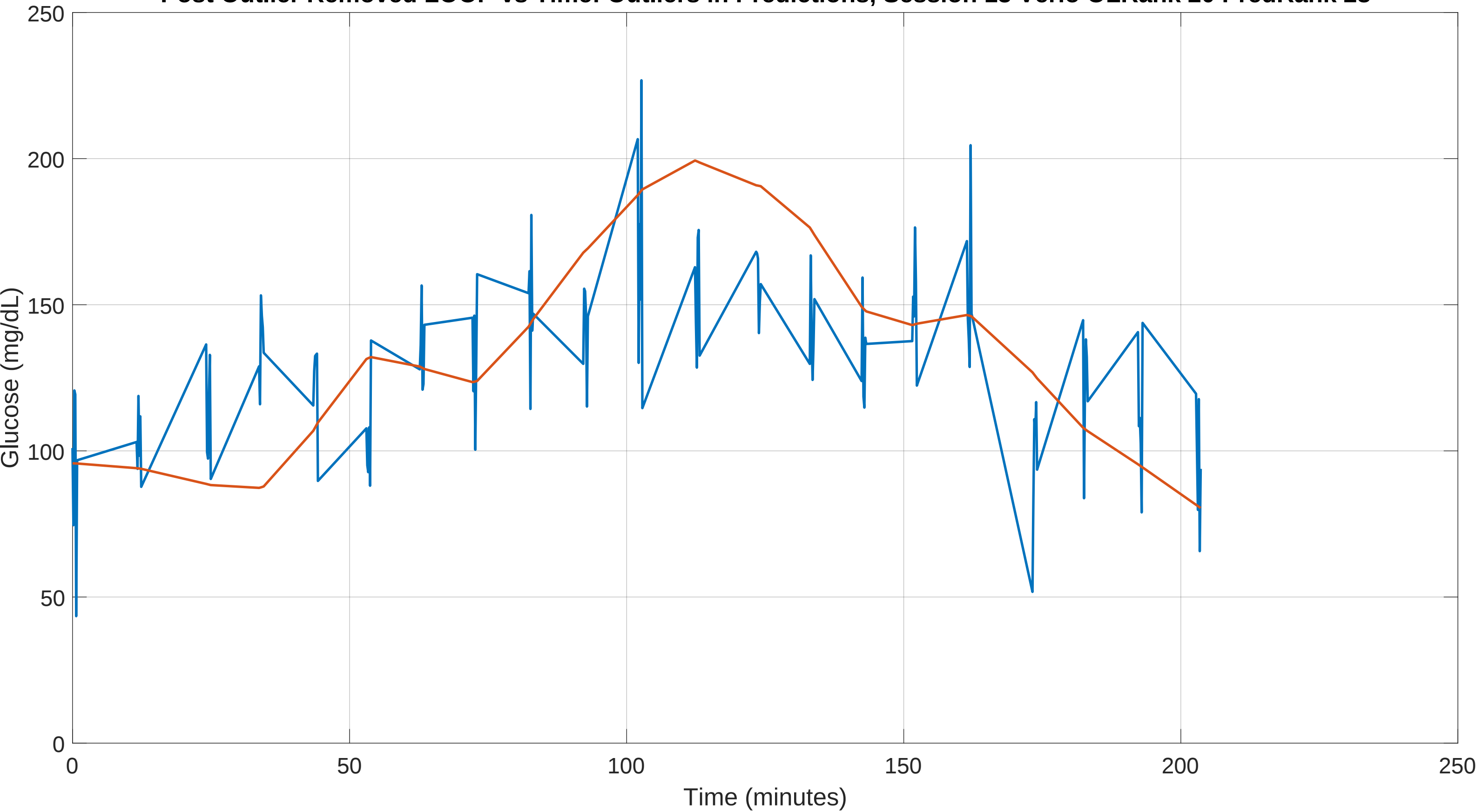
Post Outlier Removed LOOP vs Time: Outliers in Predictions, Session 13 Verio OLRank 20 PredRank 28
