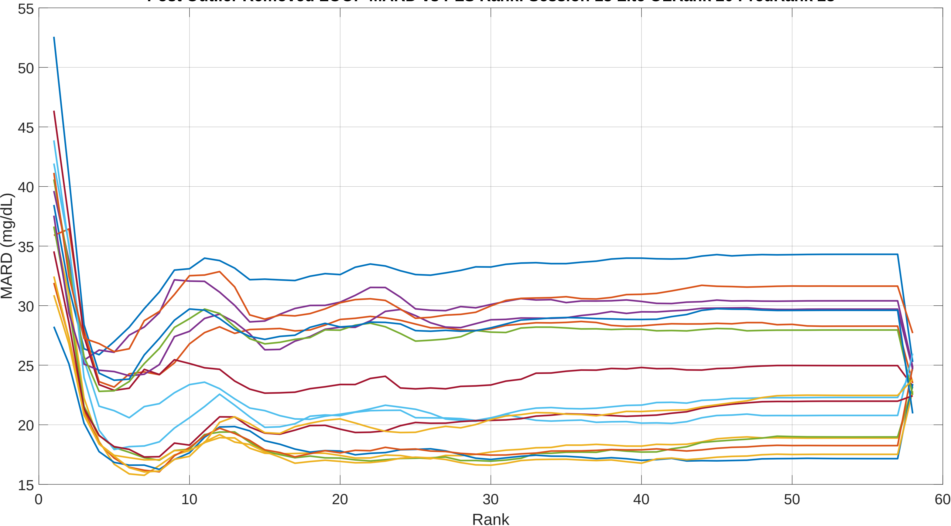
Post Outlier Removed LOOP MARD vs PLS Rank: Session 13 Lite OLRank 20 PredRank 28
