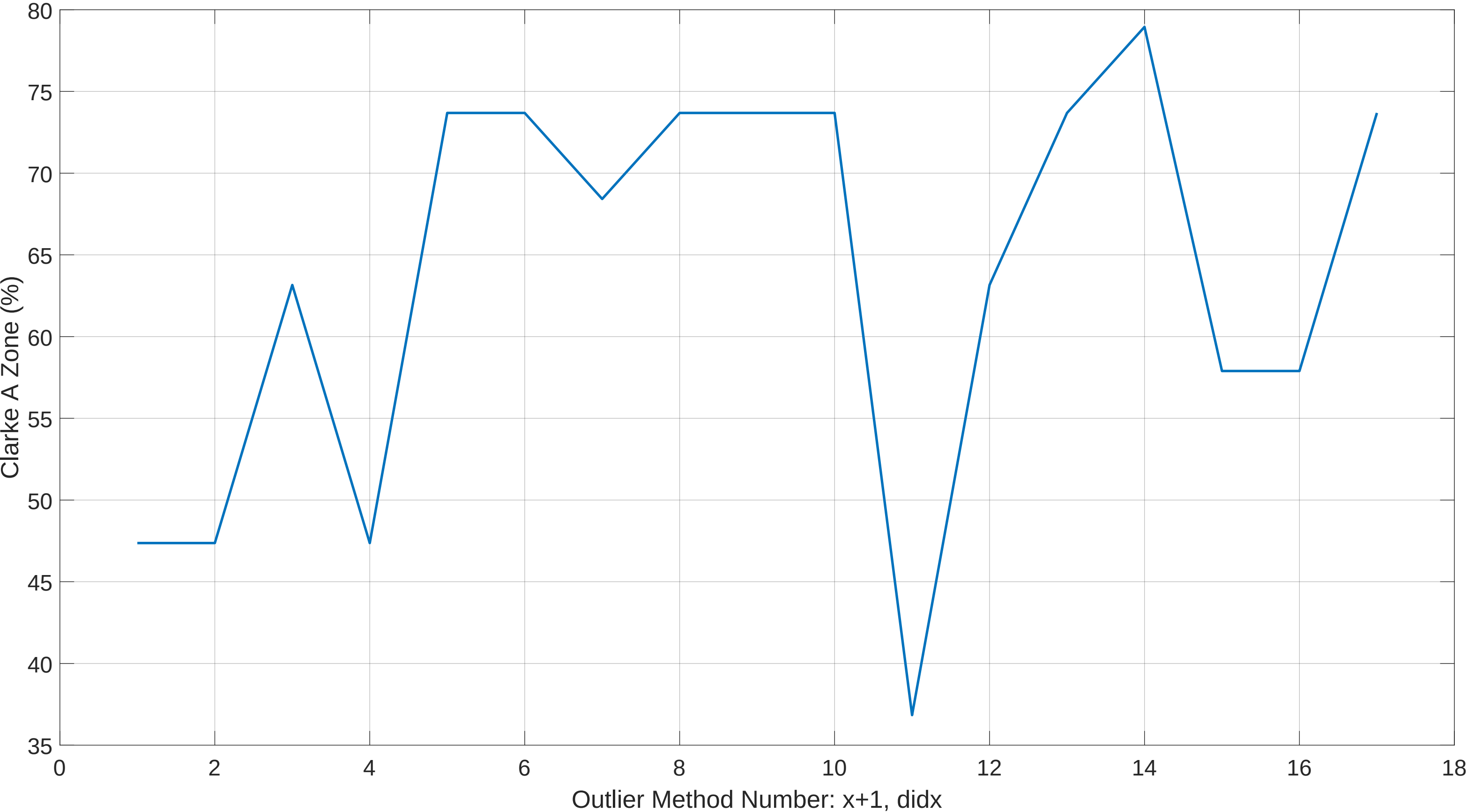
Post Outlier Removed LOOP Clarke A-Zone vs Outlier Method #: Session 12 Verio OLRank 20 PredRank 28
