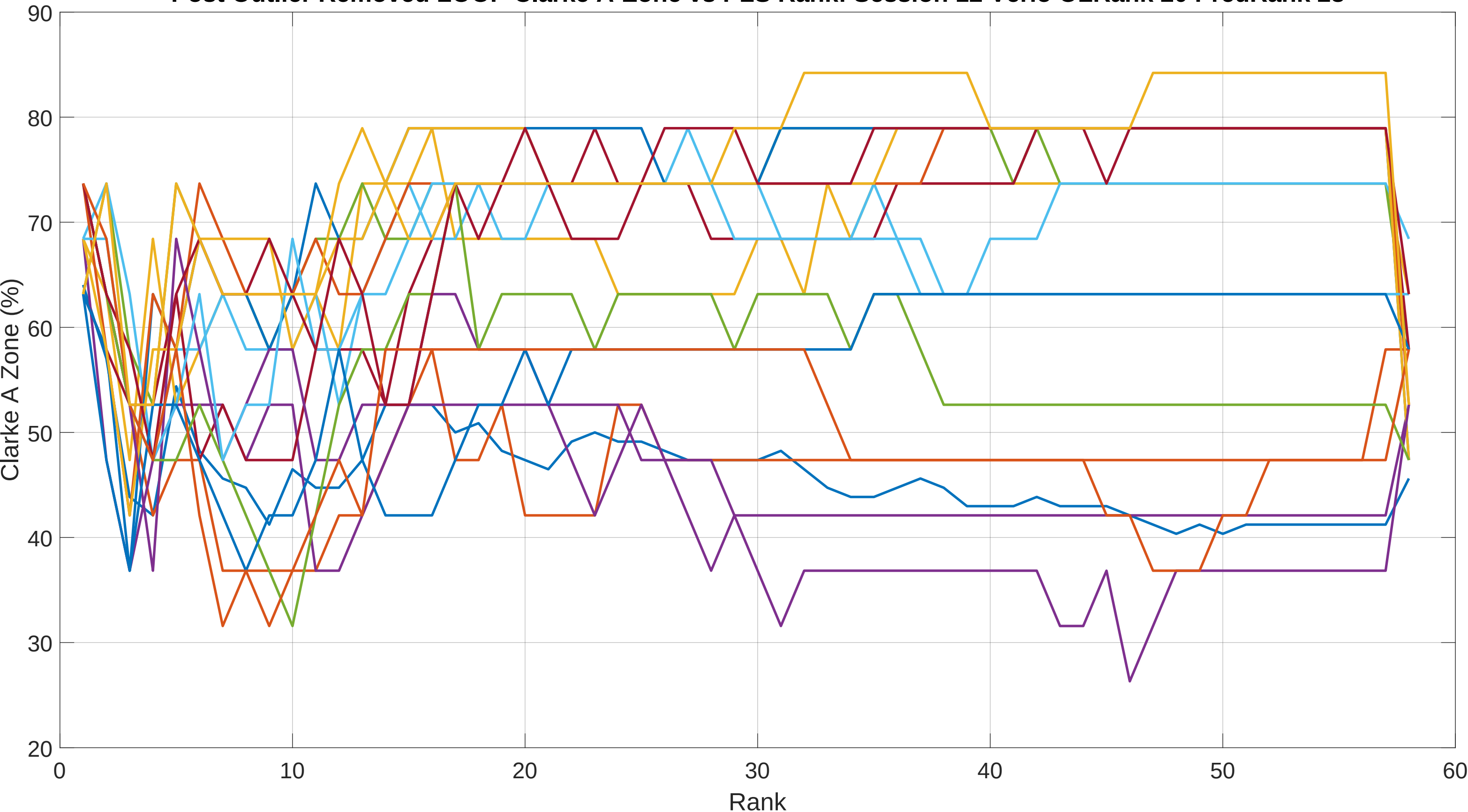
Post Outlier Removed LOOP Clarke A-Zone vs PLS Rank: Session 12 Verio OLRank 20 PredRank 28
