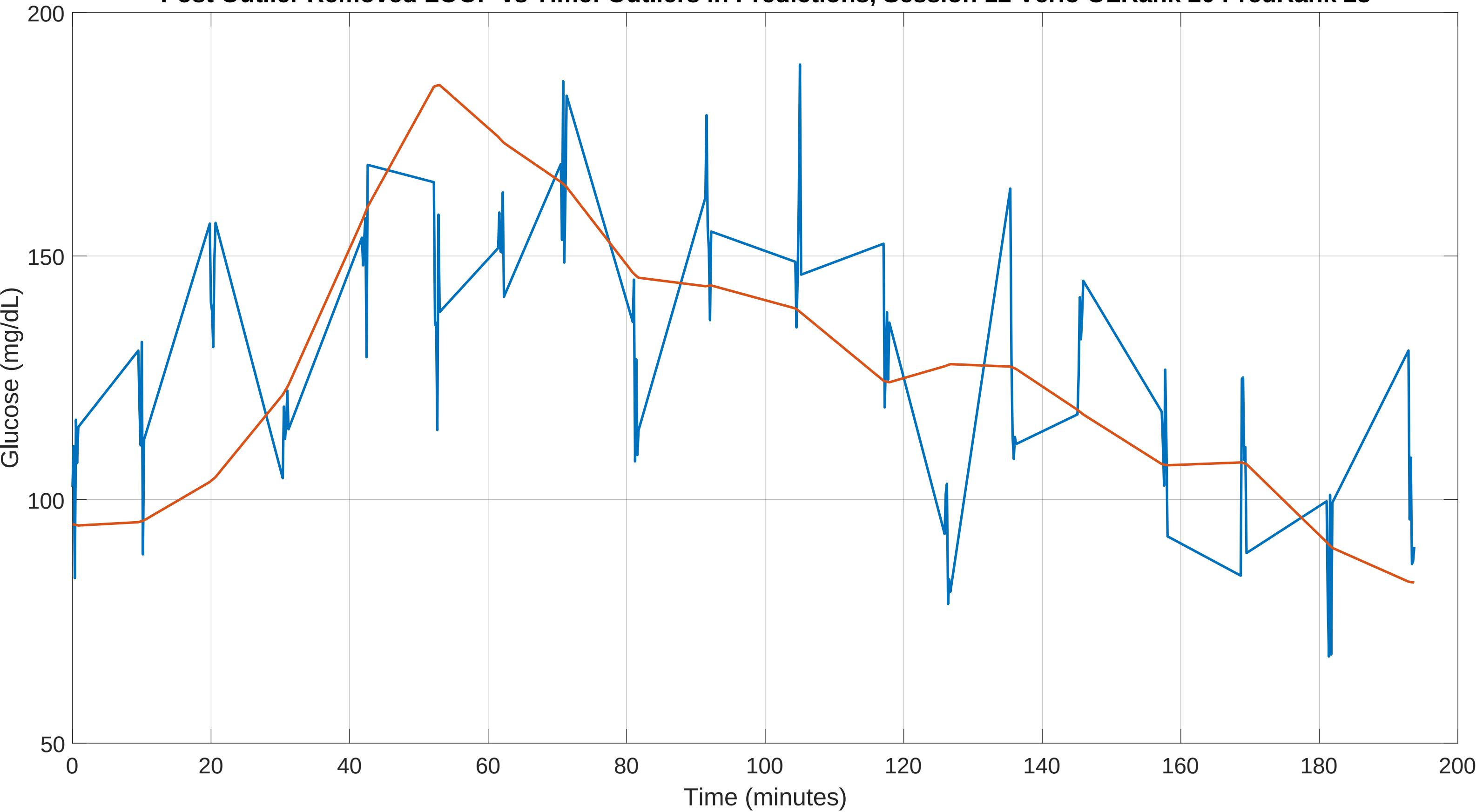
Post Outlier Removed LOOP vs Time: Outliers in Predictions, Session 12 Verio OLRank 20 PredRank 28
