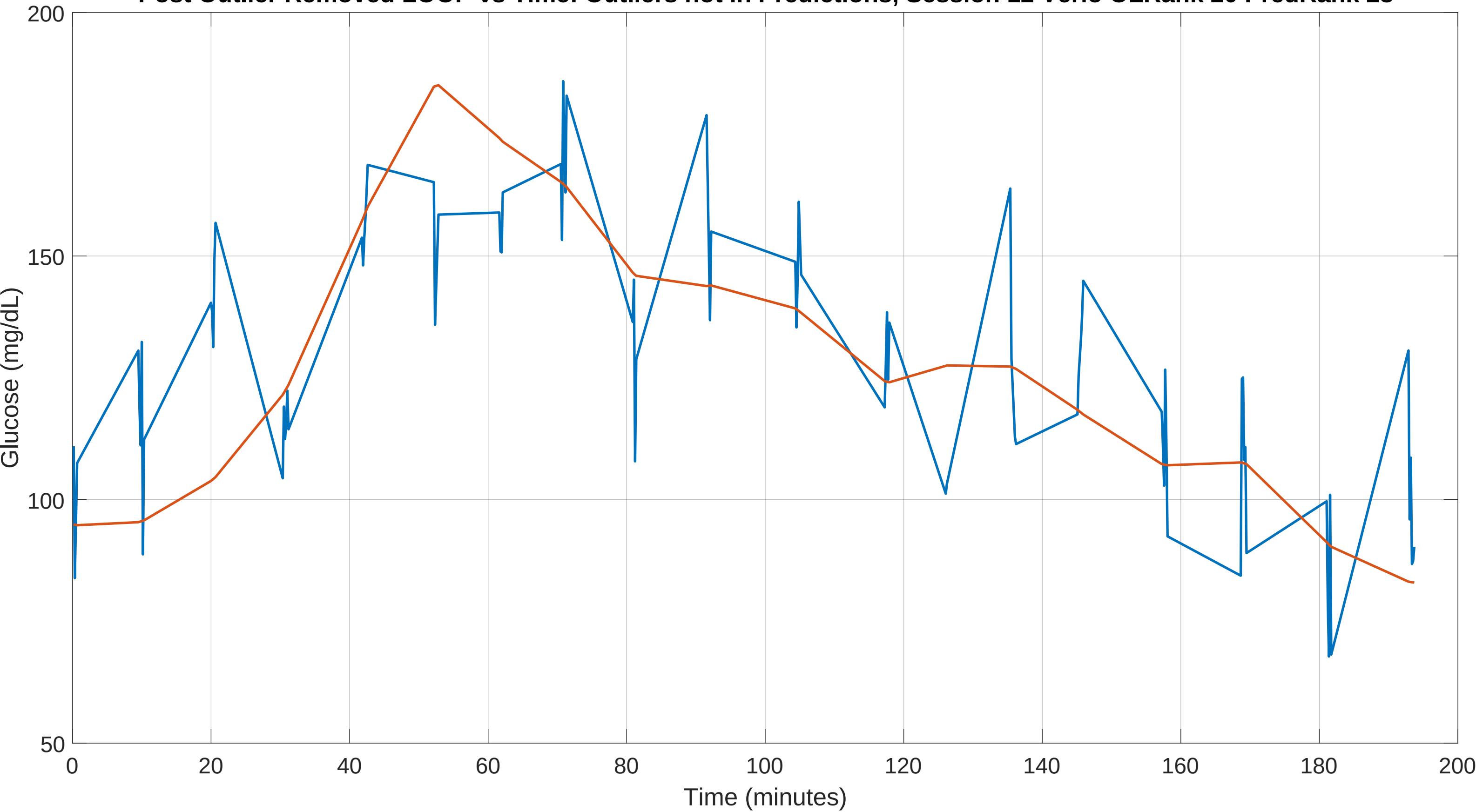
Post Outlier Removed LOOP vs Time: Outliers not in Predictions, Session 12 Verio OLRank 20 PredRank 28
