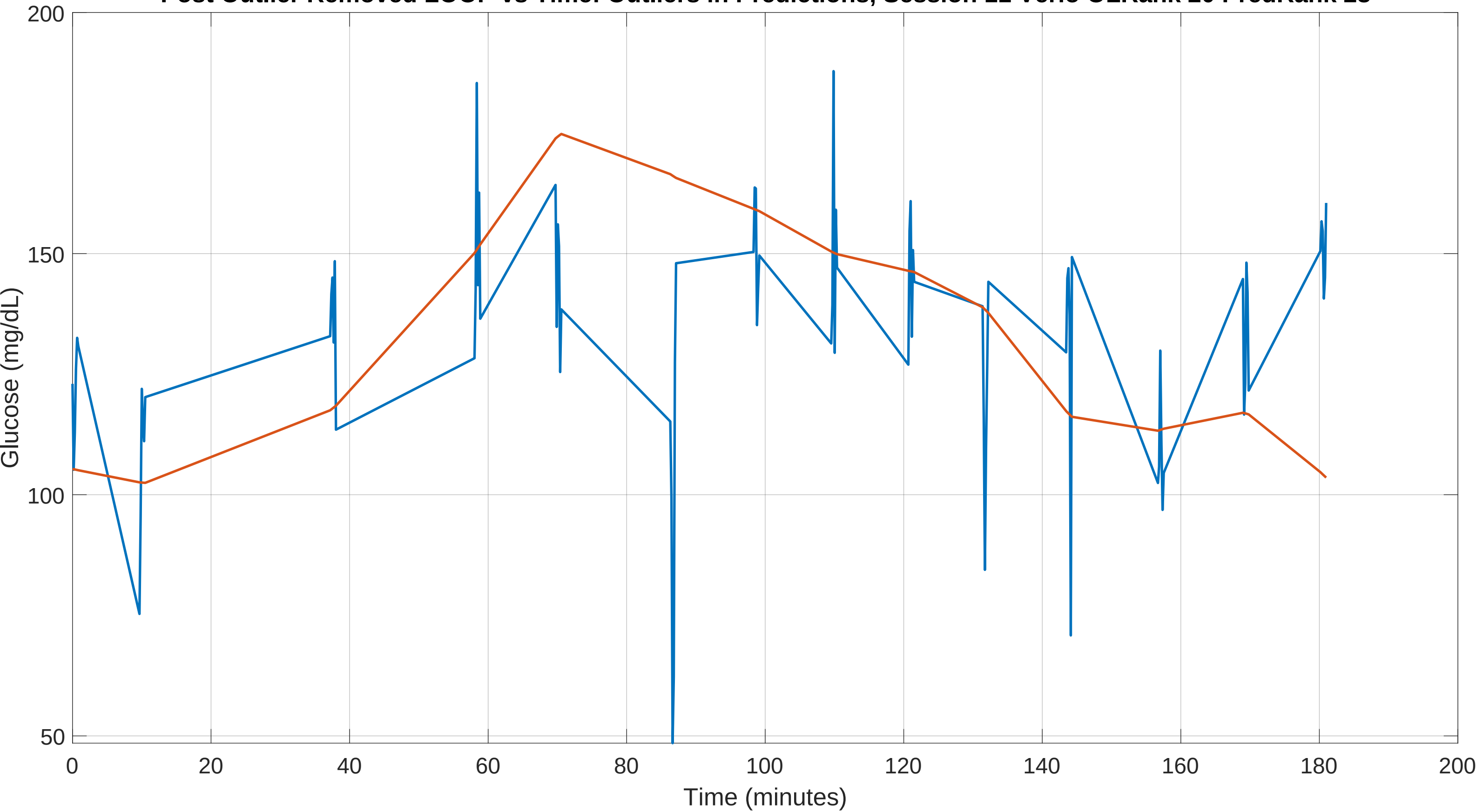
Post Outlier Removed LOOP vs Time: Outliers in Predictions, Session 11 Verio OLRank 20 PredRank 28
