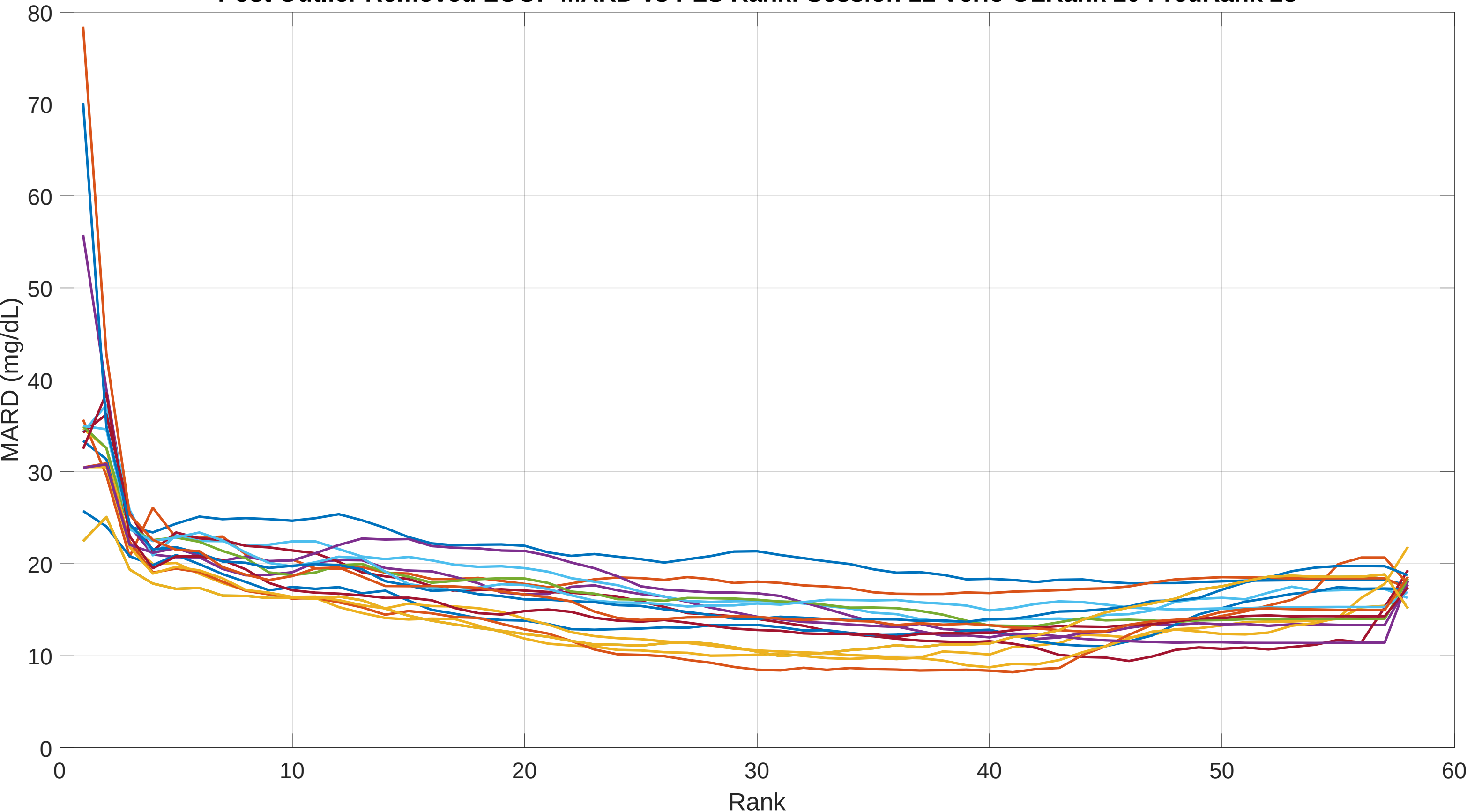
Post Outlier Removed LOOP MARD vs PLS Rank: Session 11 Verio OLRank 20 PredRank 28
