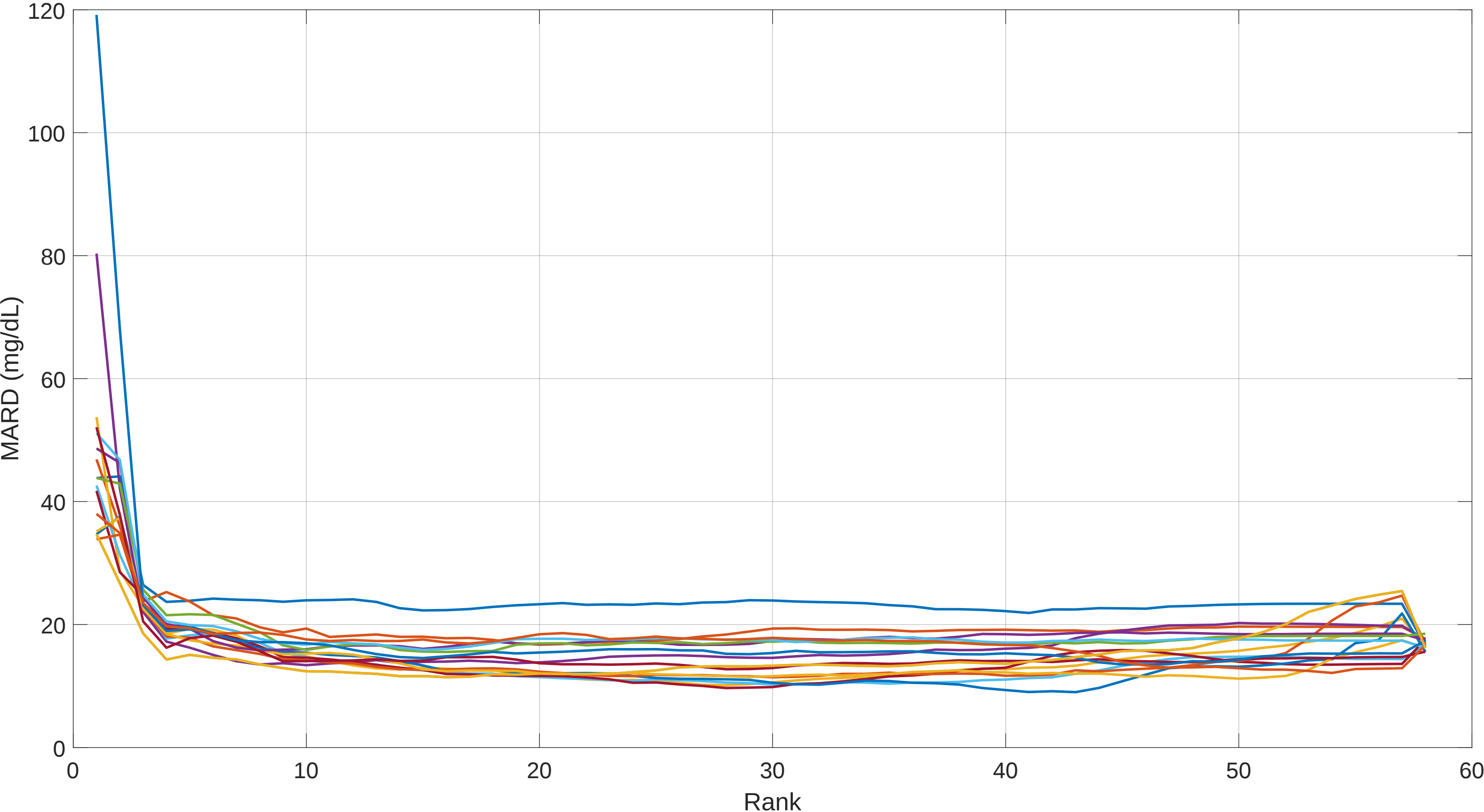
Post Outlier Removed LOOP MARD vs PLS Rank: Session 11 Oxi OLRank 20 PredRank 28
