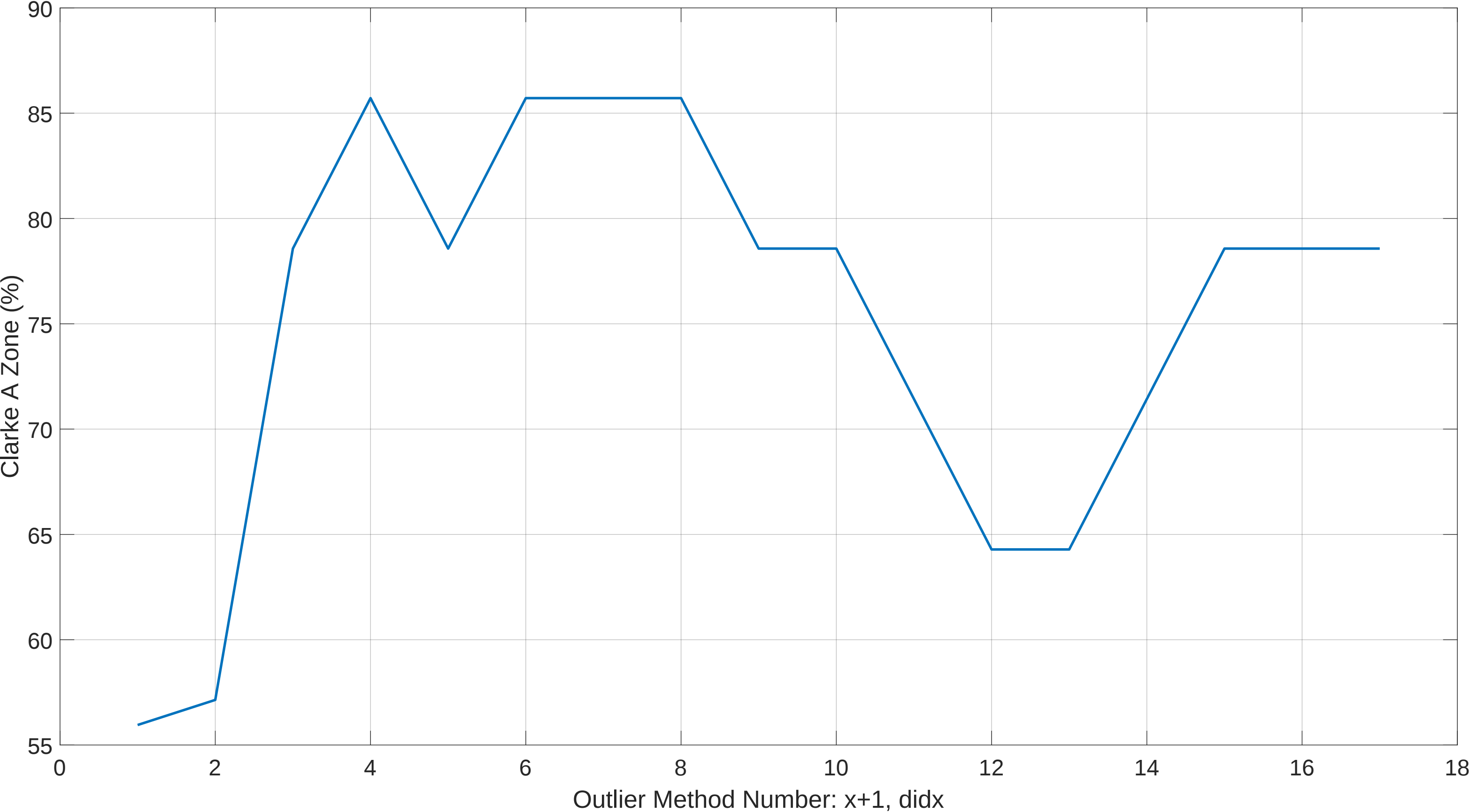
Post Outlier Removed LOOP Clarke A-Zone vs Outlier Method #: Session 11 Oxi OLRank 20 PredRank 28
