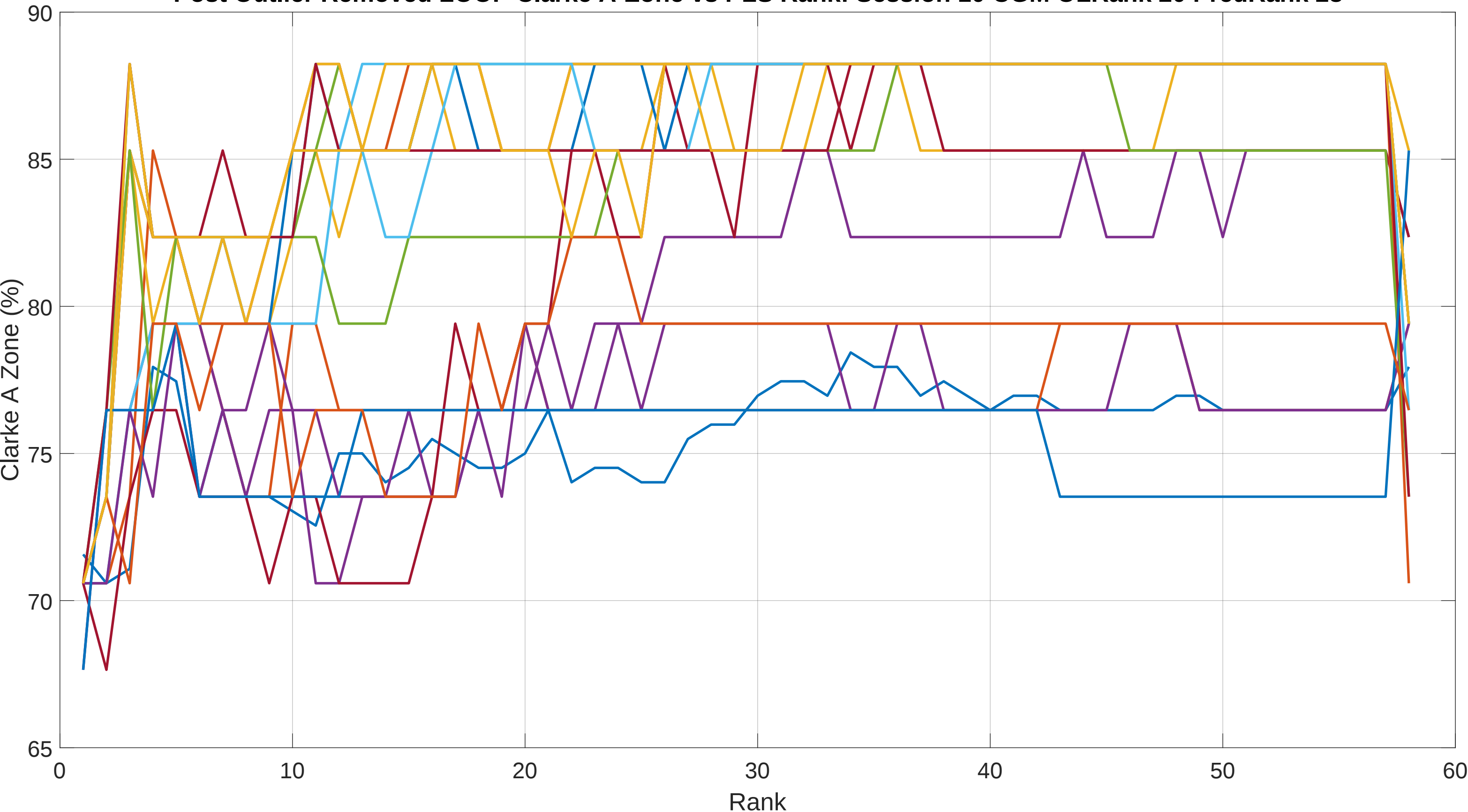
Post Outlier Removed LOOP Clarke A-Zone vs PLS Rank: Session 10 CGM OLRank 20 PredRank 28
