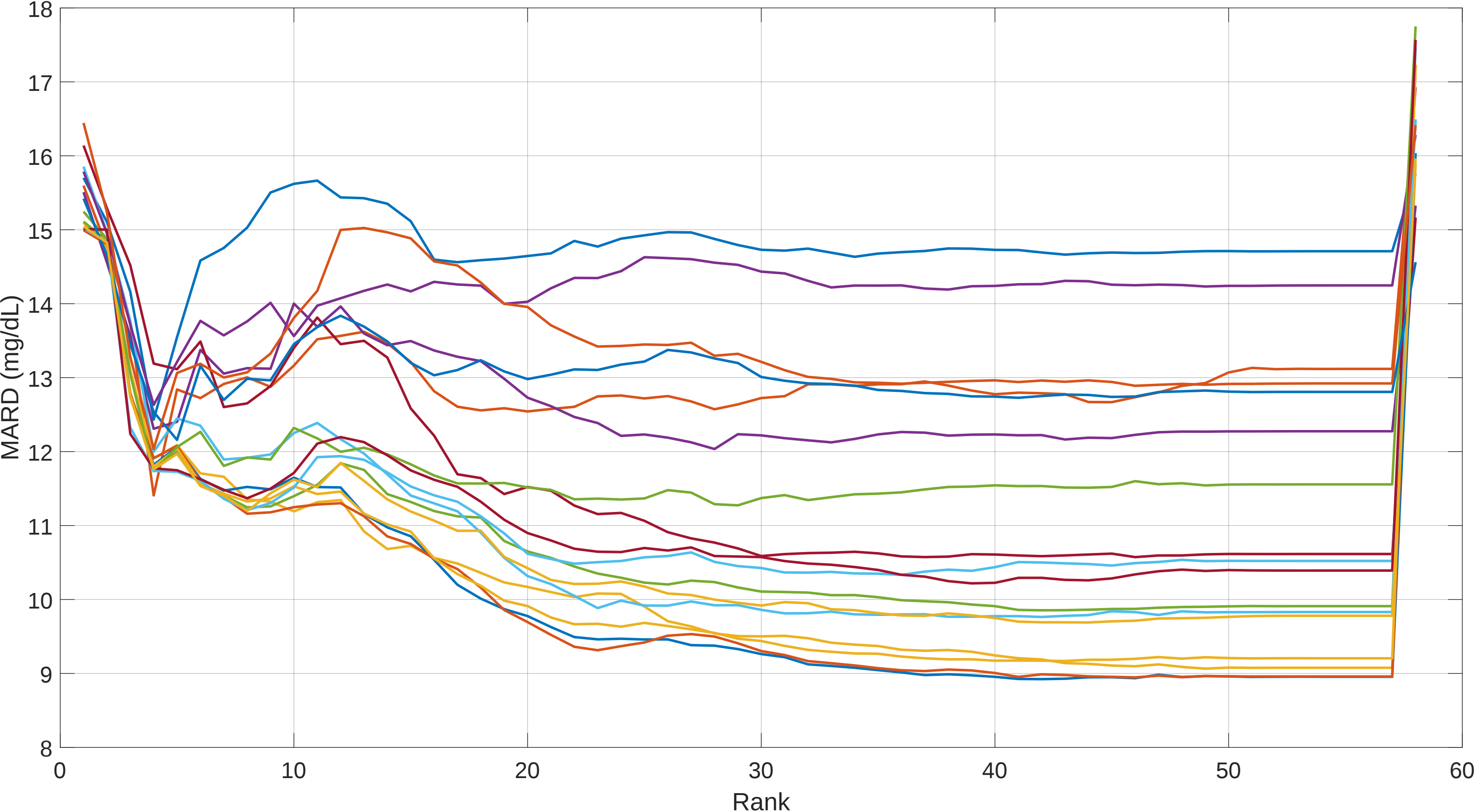
Post Outlier Removed LOOP MARD vs PLS Rank: Session 10 CGM OLRank 20 PredRank 28
