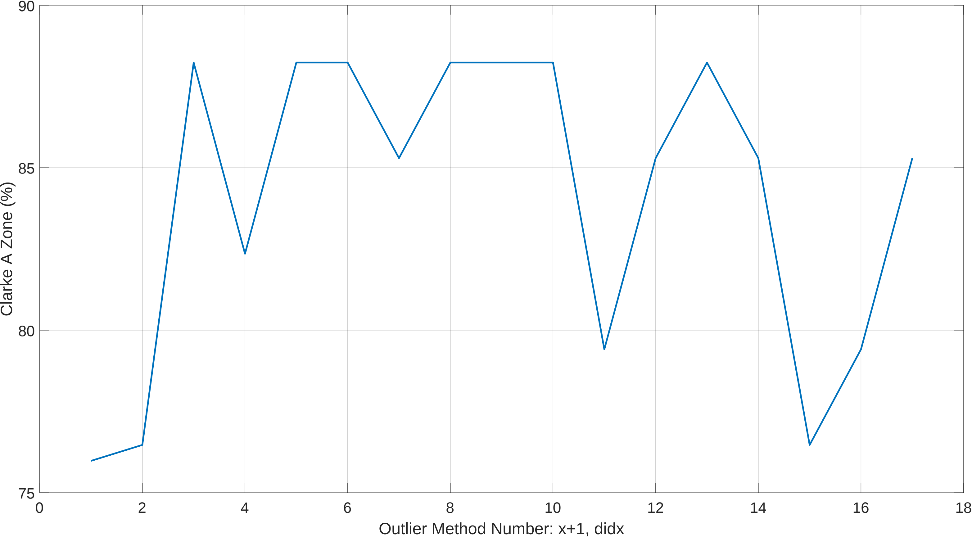
Post Outlier Removed LOOP Clarke A-Zone vs Outlier Method #: Session 10 CGM OLRank 20 PredRank 28
