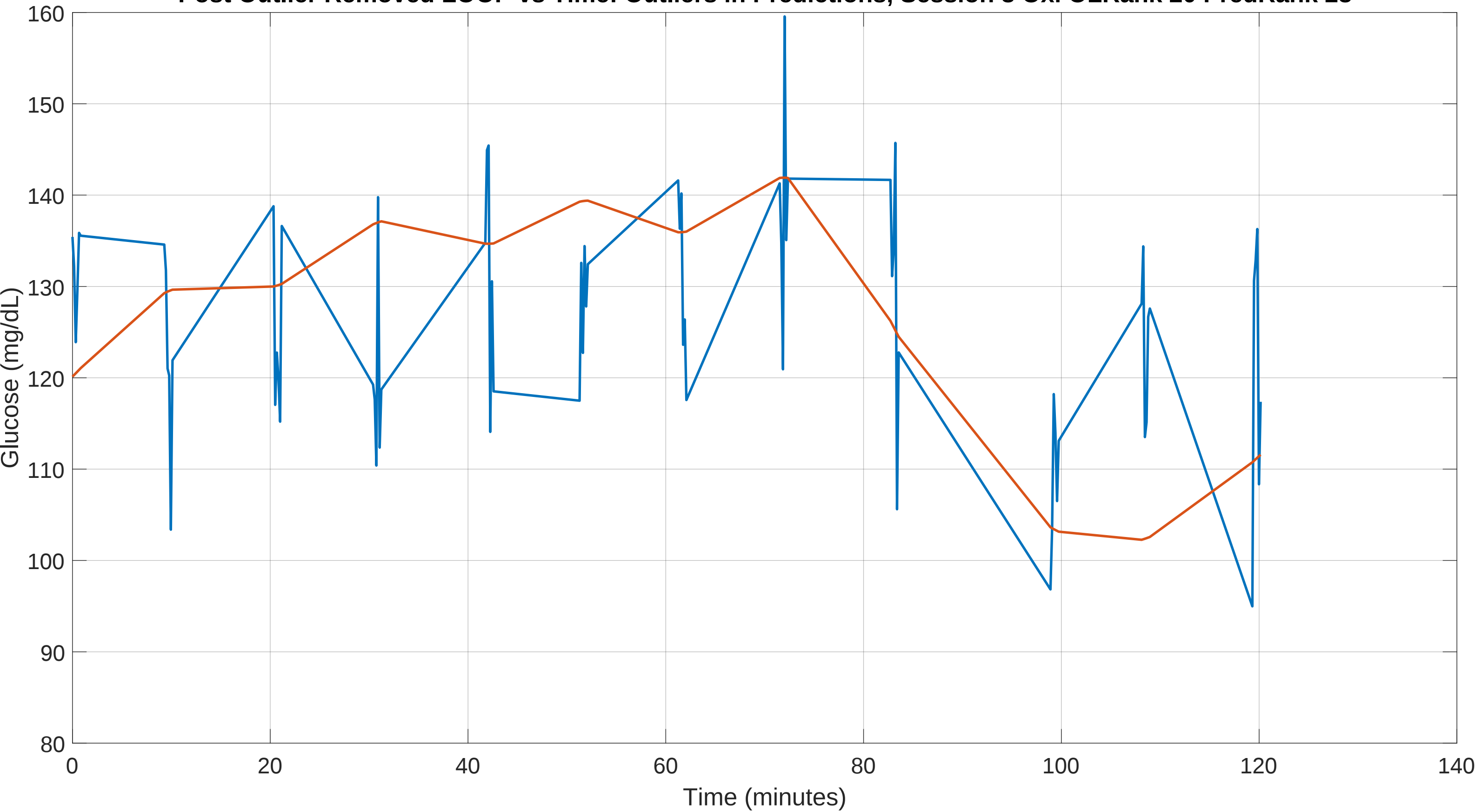
Post Outlier Removed LOOP vs Time: Outliers in Predictions, Session 8 Oxi OLRank 20 PredRank 28
