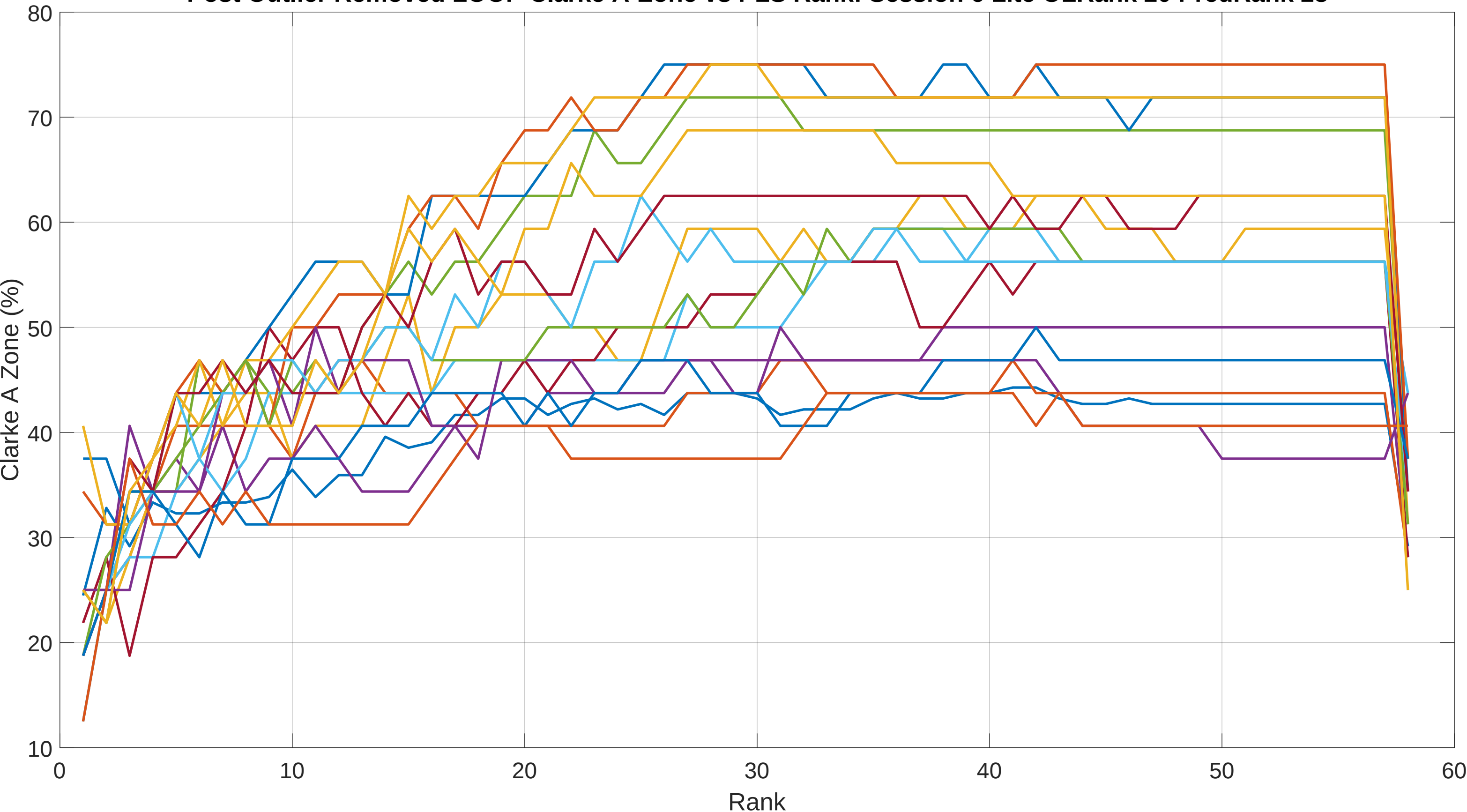
Post Outlier Removed LOOP Clarke A-Zone vs PLS Rank: Session 6 Lite OLRank 20 PredRank 28
