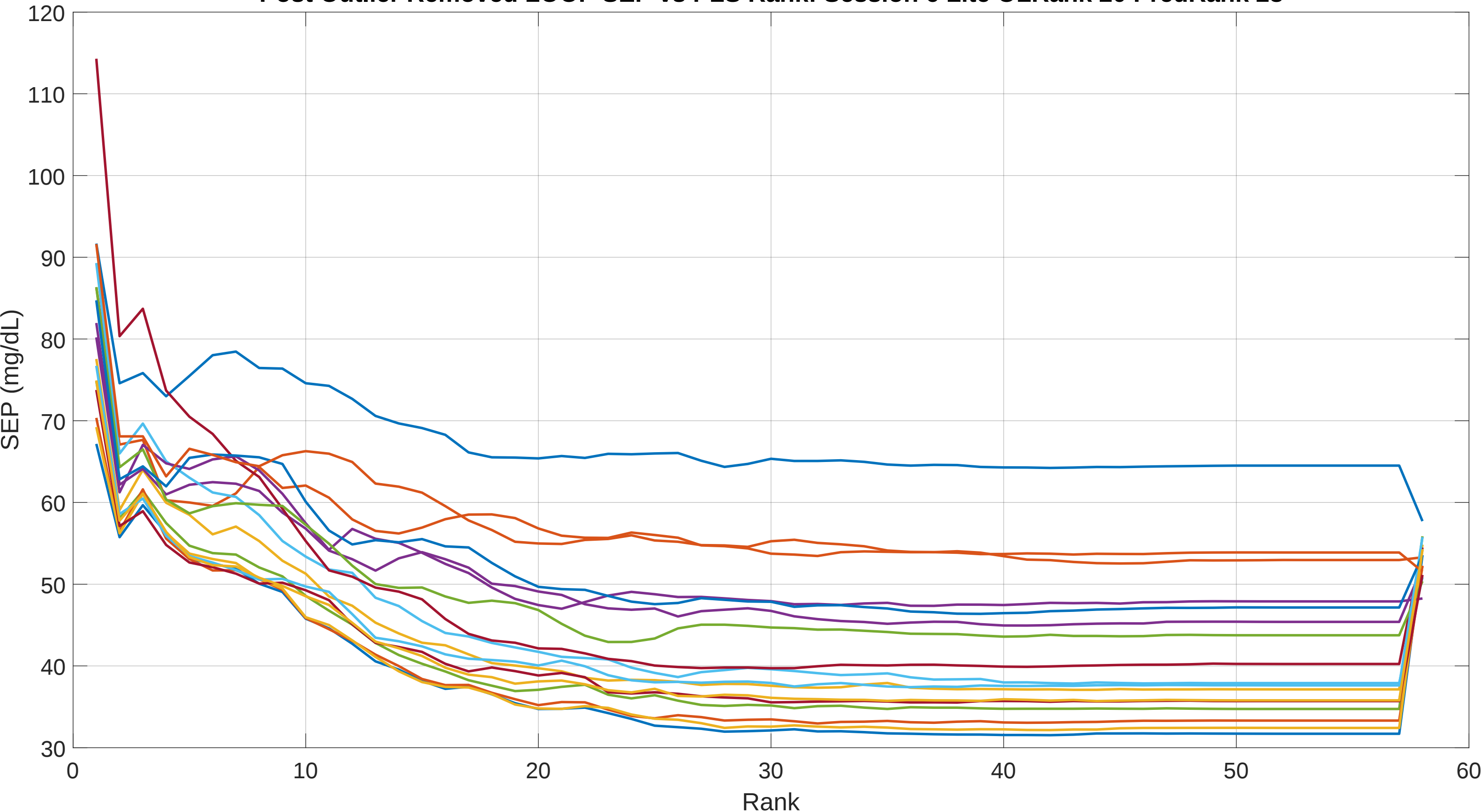
Post Outlier Removed LOOP SEP vs PLS Rank: Session 6 Lite OLRank 20 PredRank 28
