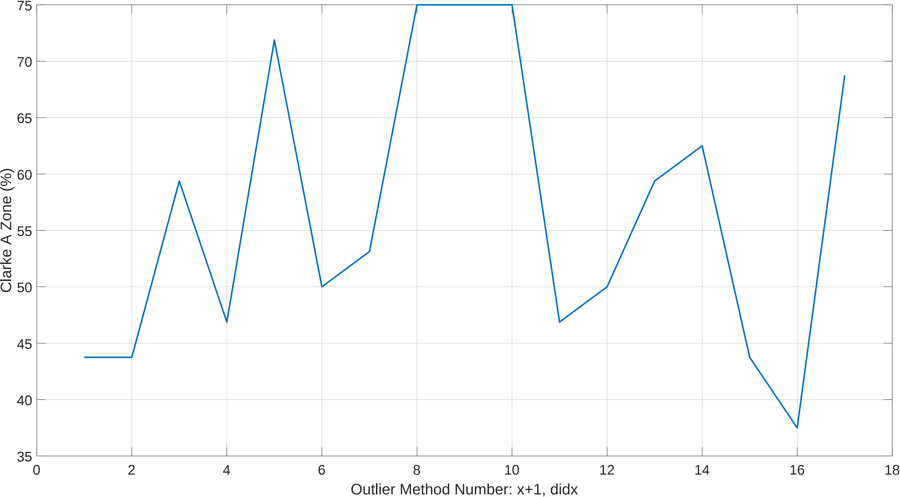
Post Outlier Removed LOOP Clarke A-Zone vs Outlier Method #: Session 6 Lite OLRank 20 PredRank 28
