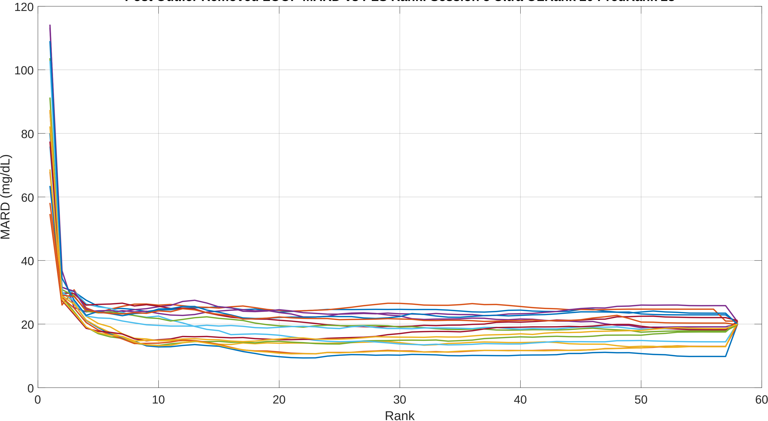
Post Outlier Removed LOOP MARD vs PLS Rank: Session 5 Ultra OLRank 20 PredRank 28
