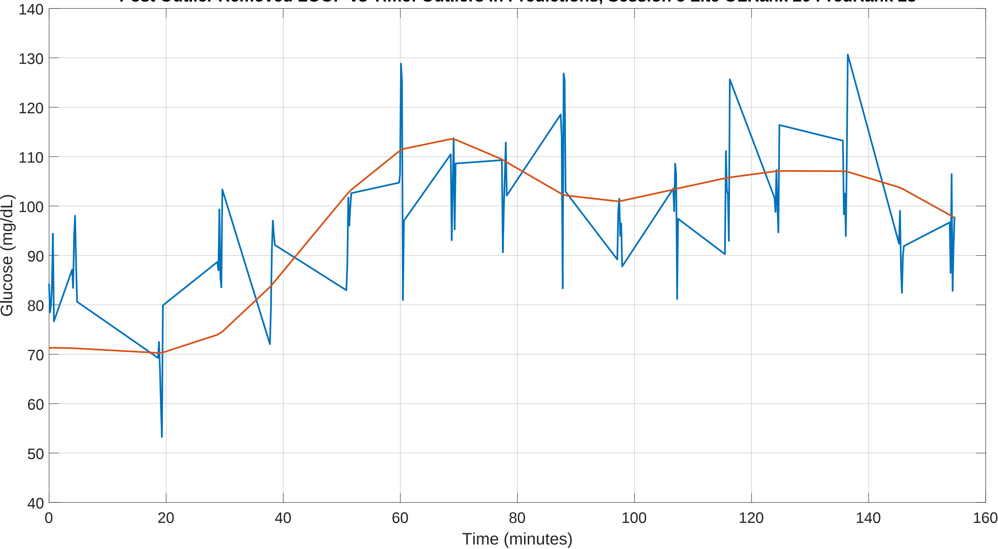
Post Outlier Removed LOOP vs Time: Outliers in Predictions, Session 5 Lite OLRank 20 PredRank 28
