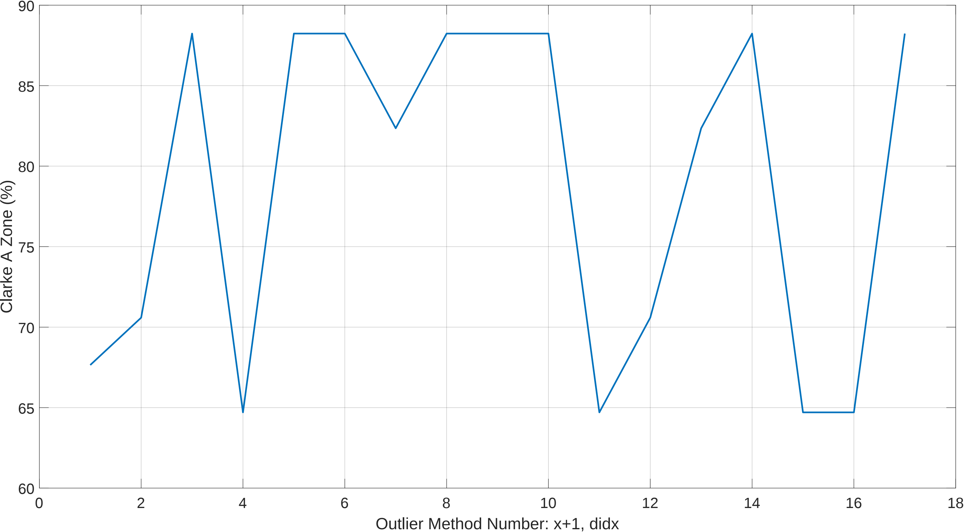
Post Outlier Removed LOOP Clarke A-Zone vs Outlier Method #: Session 5 Lite OLRank 20 PredRank 28
