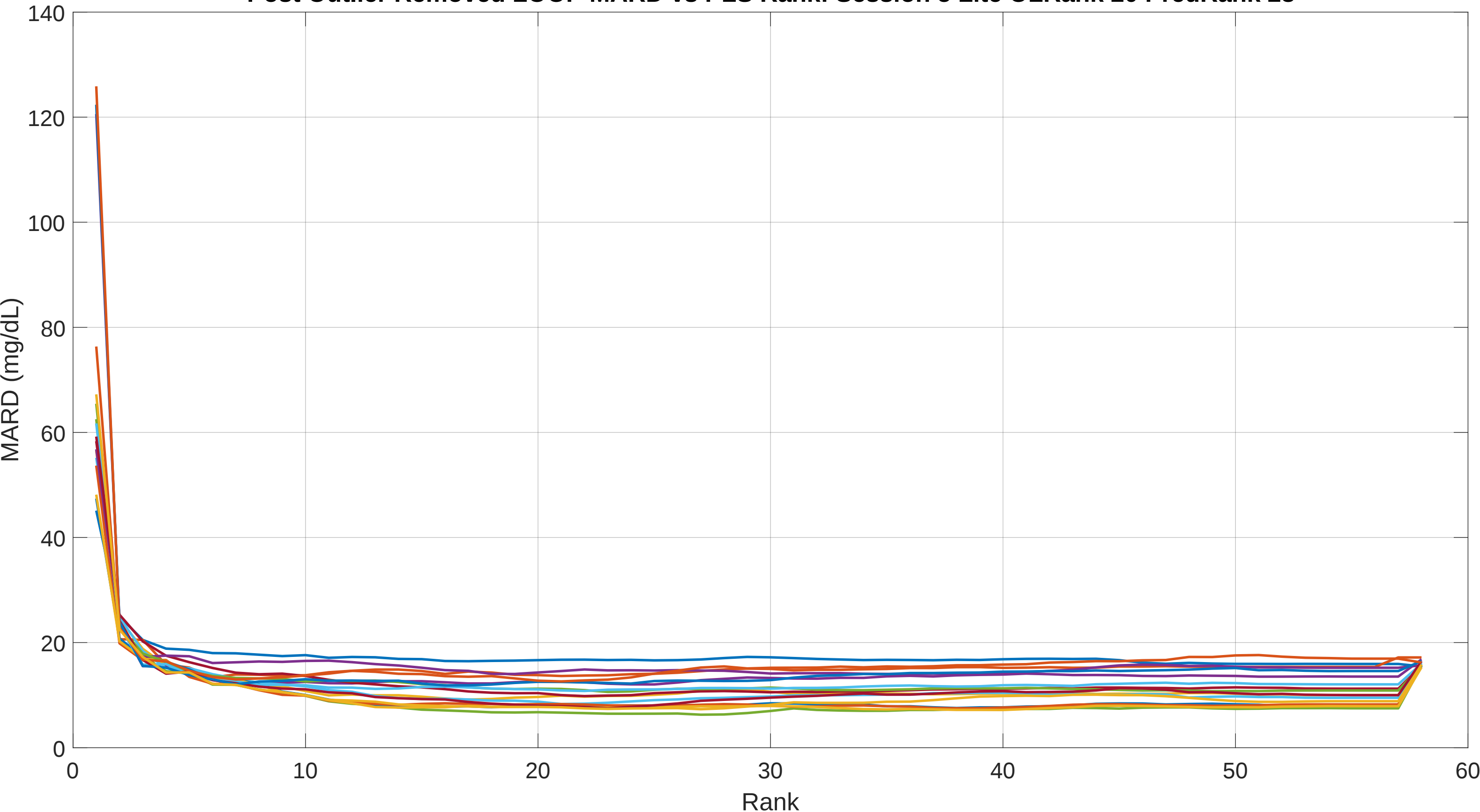
Post Outlier Removed LOOP MARD vs PLS Rank: Session 5 Lite OLRank 20 PredRank 28
