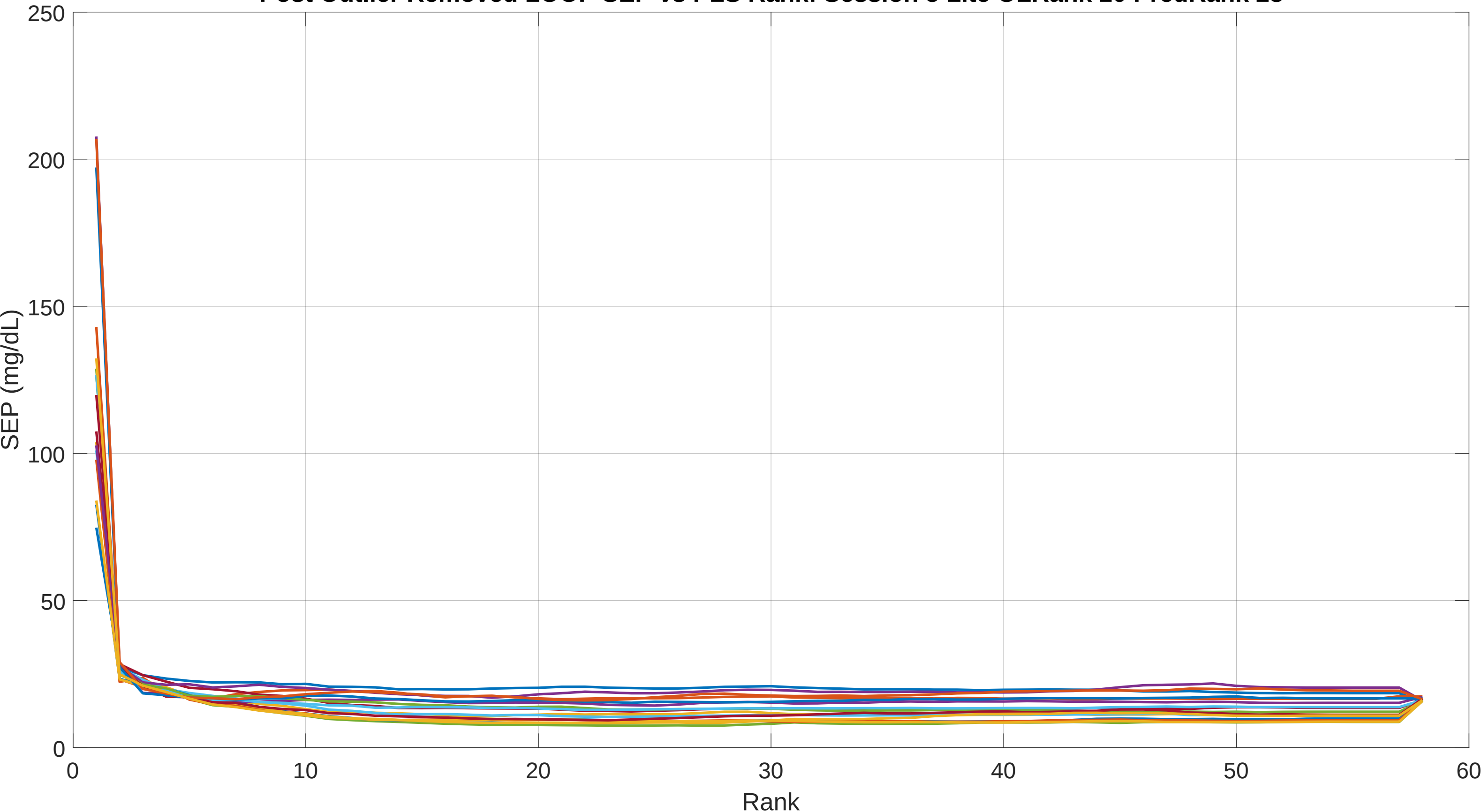
Post Outlier Removed LOOP SEP vs PLS Rank: Session 5 Lite OLRank 20 PredRank 28
