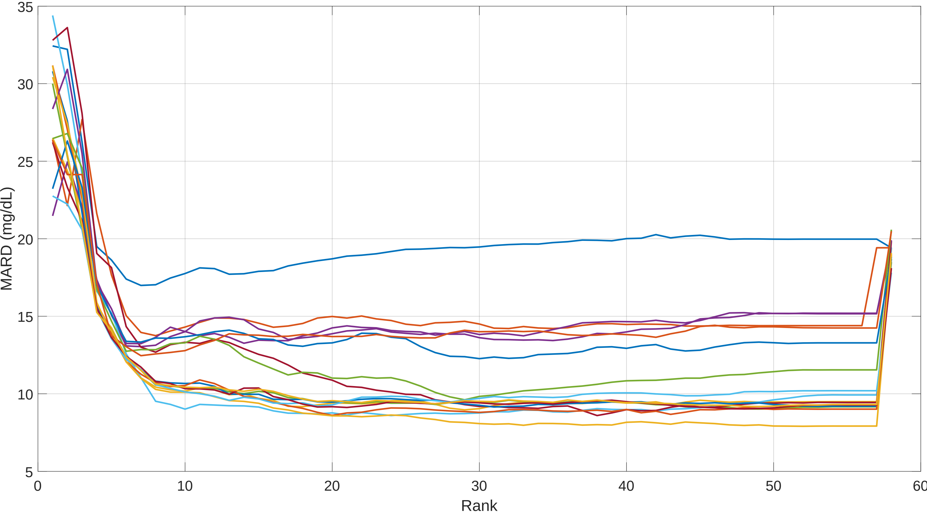
Post Outlier Removed LOOP MARD vs PLS Rank: Session 4 Ultra OLRank 20 PredRank 28
