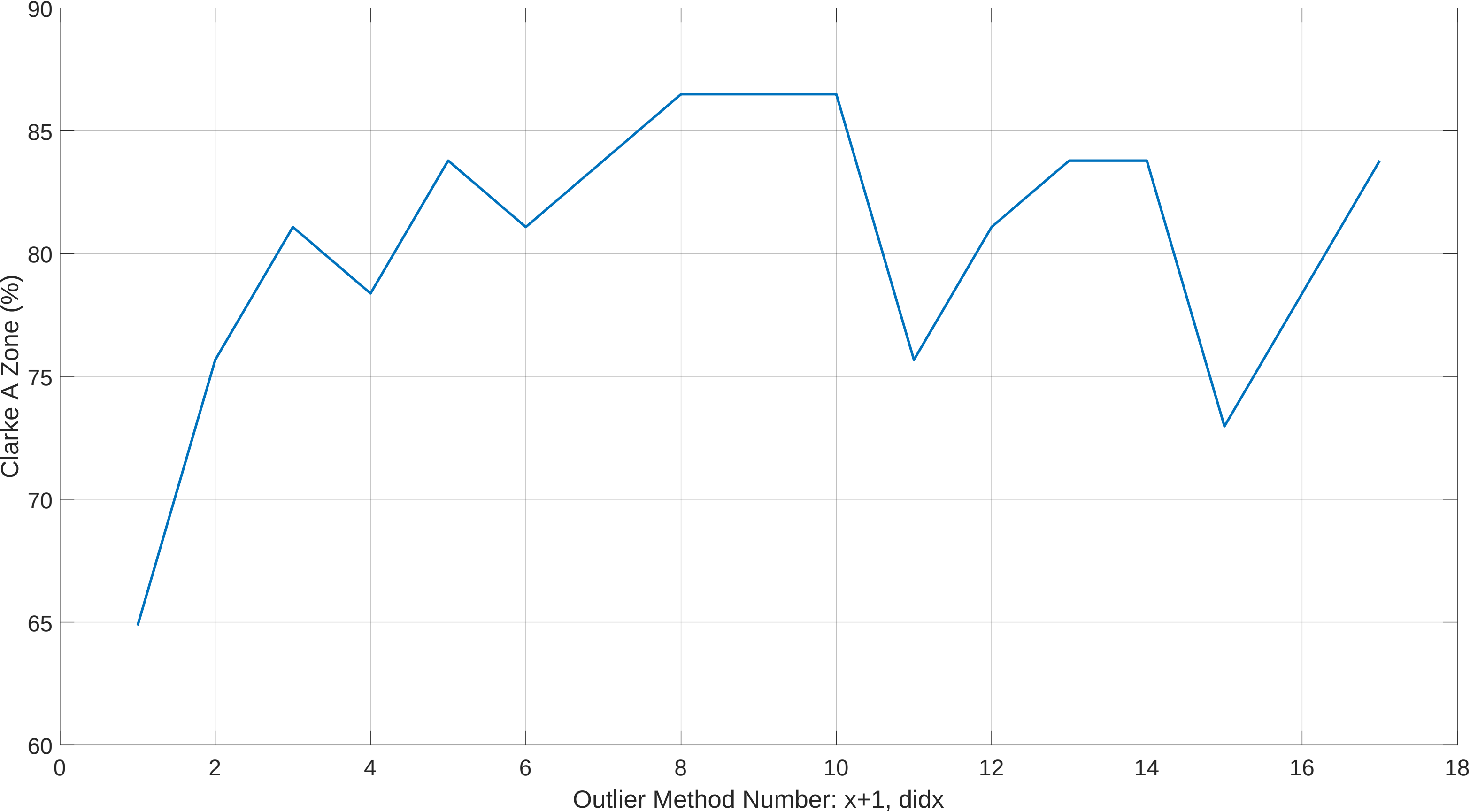
Post Outlier Removed LOOP Clarke A-Zone vs Outlier Method #: Session 3 CGM OLRank 20 PredRank 28
