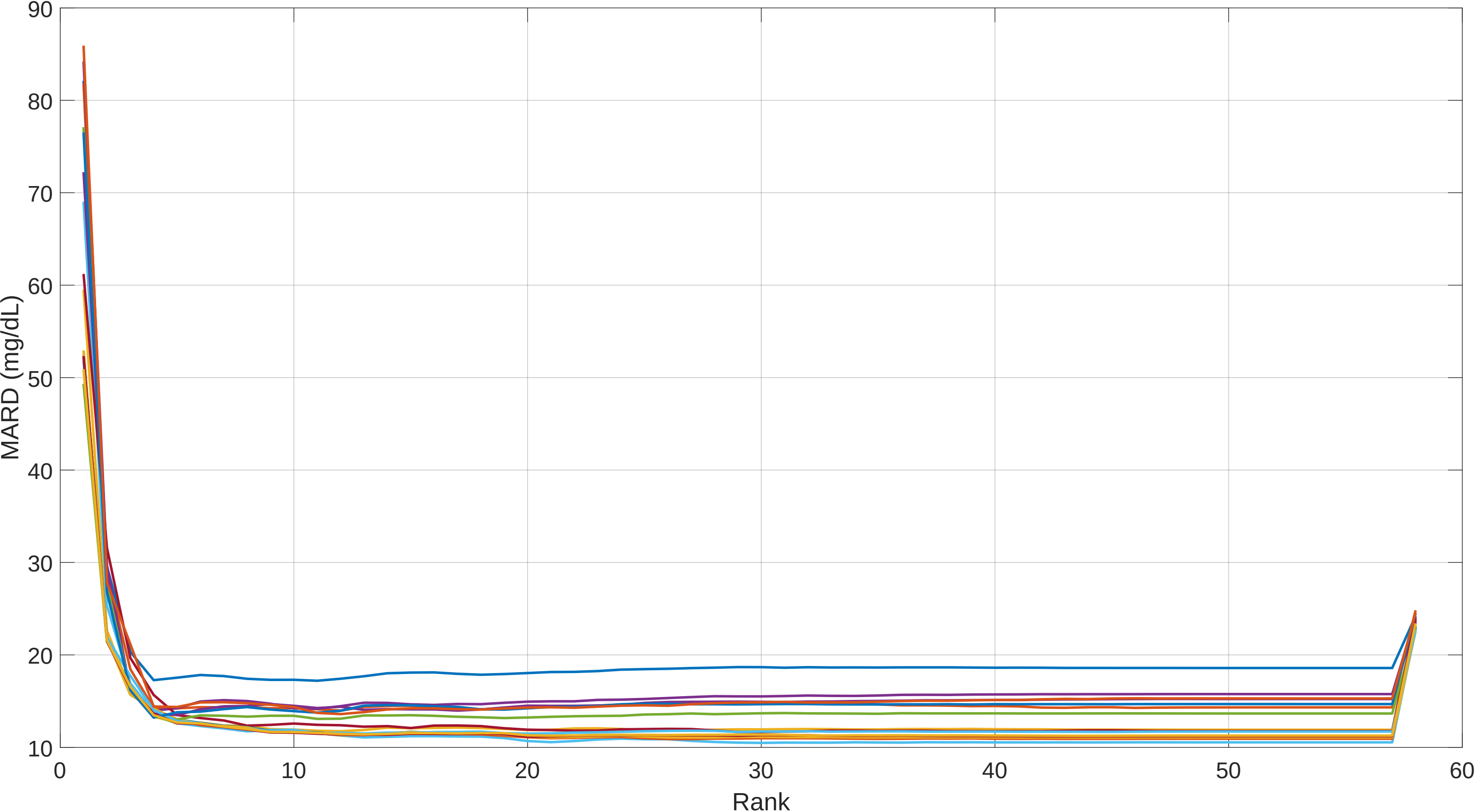
Post Outlier Removed LOOP MARD vs PLS Rank: Session 3 CGM OLRank 20 PredRank 28
