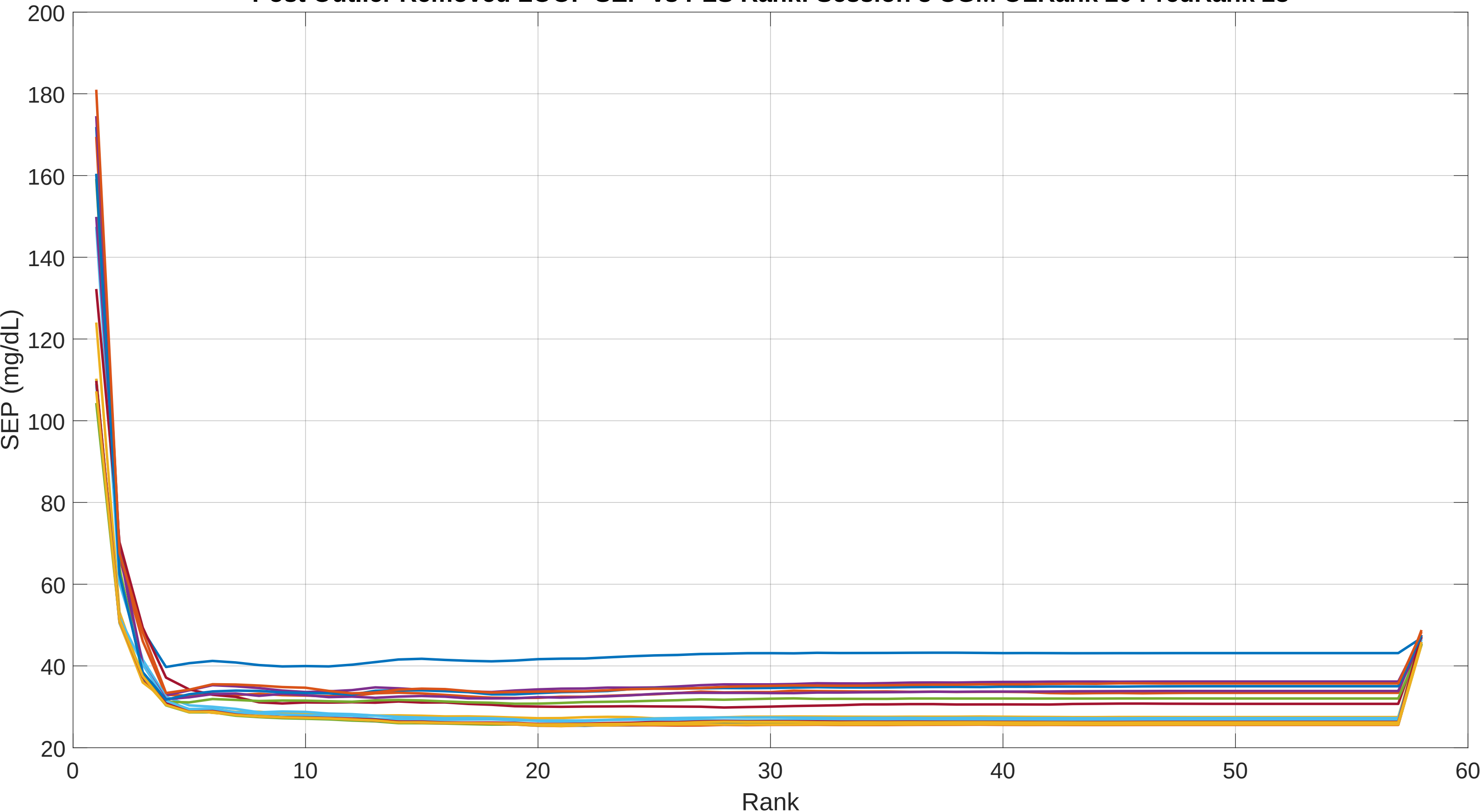
Post Outlier Removed LOOP SEP vs PLS Rank: Session 3 CGM OLRank 20 PredRank 28
