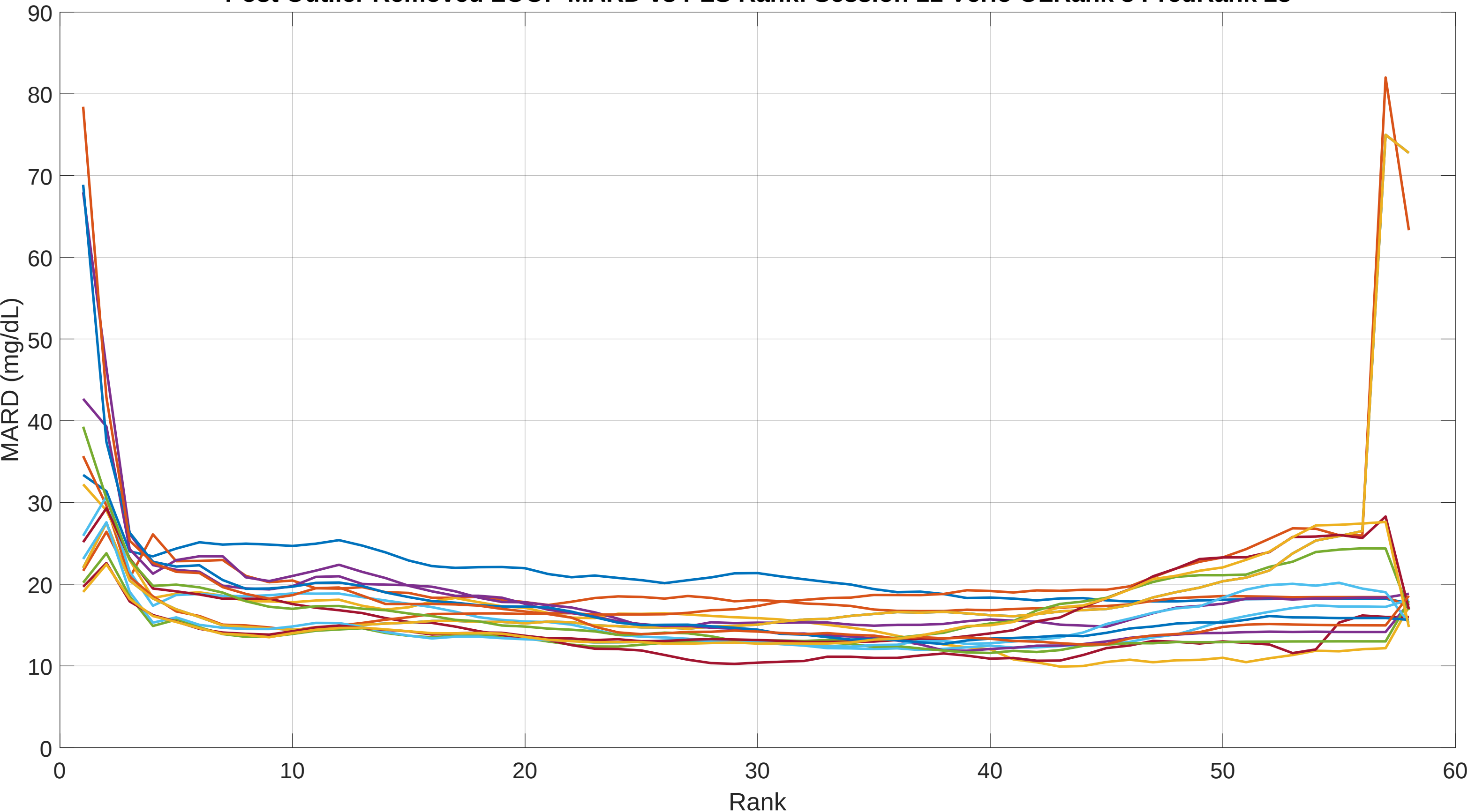
Post Outlier Removed LOOP MARD vs PLS Rank: Session 11 Verio OLRank 8 PredRank 28
