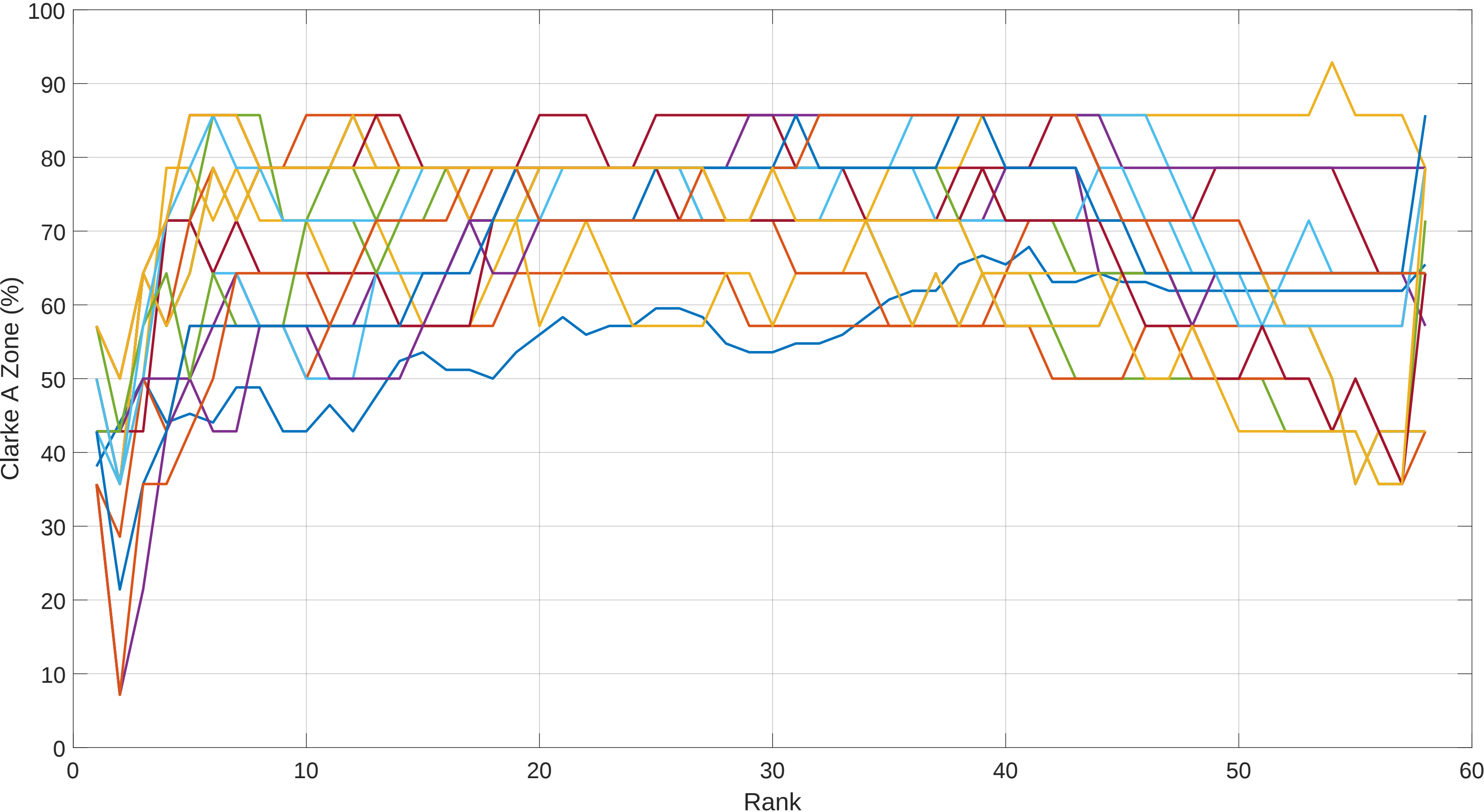
Post Outlier Removed LOOP Clarke A-Zone vs PLS Rank: Session 11 Verio OLRank 8 PredRank 28
