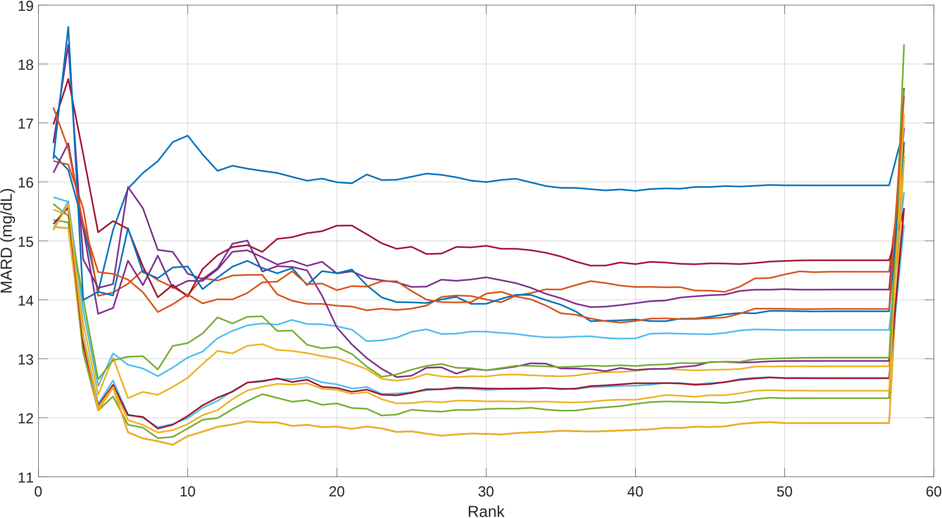
Post Outlier Removed LOOP MARD vs PLSRank: Session 10 Oxi OLRank 8 PredRank 28
