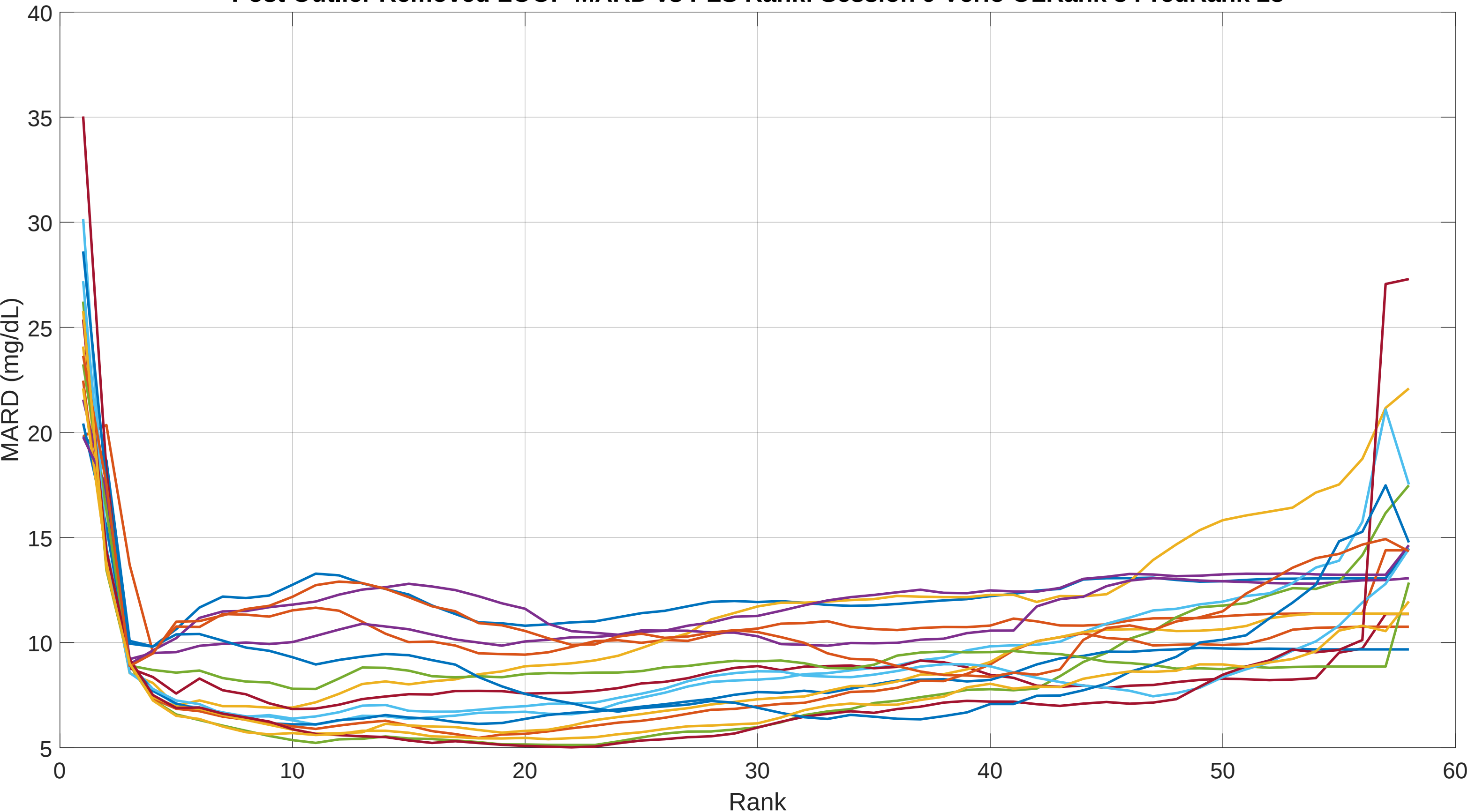
Post Outlier Removed LOOP MARD vs PLS Rank: Session 9 Verio OLRank 8 PredRank 28
