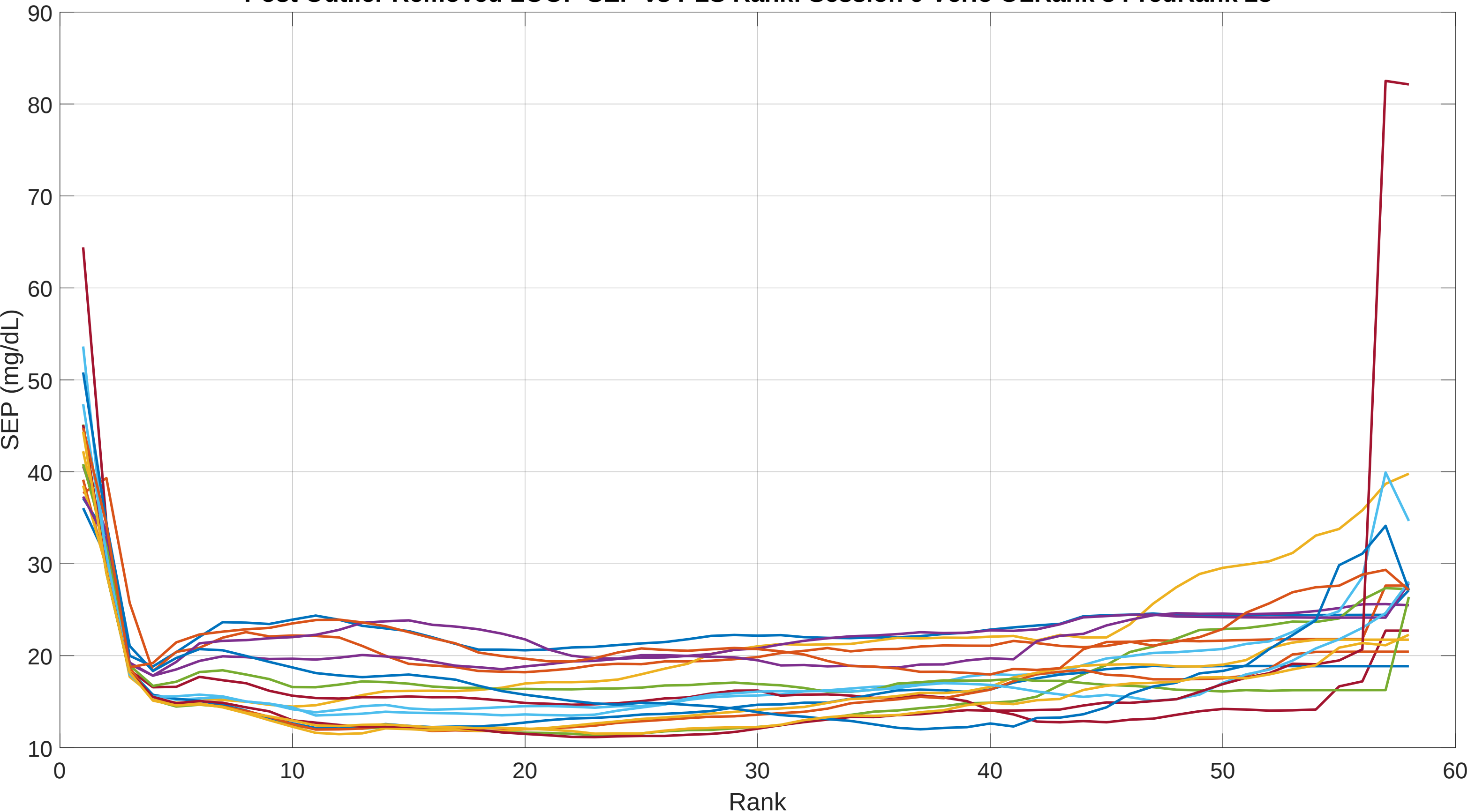
Post Outlier Removed LOOP SEP vs PLS Rank: Session 9 Verio OLRank 8 PredRank 28
