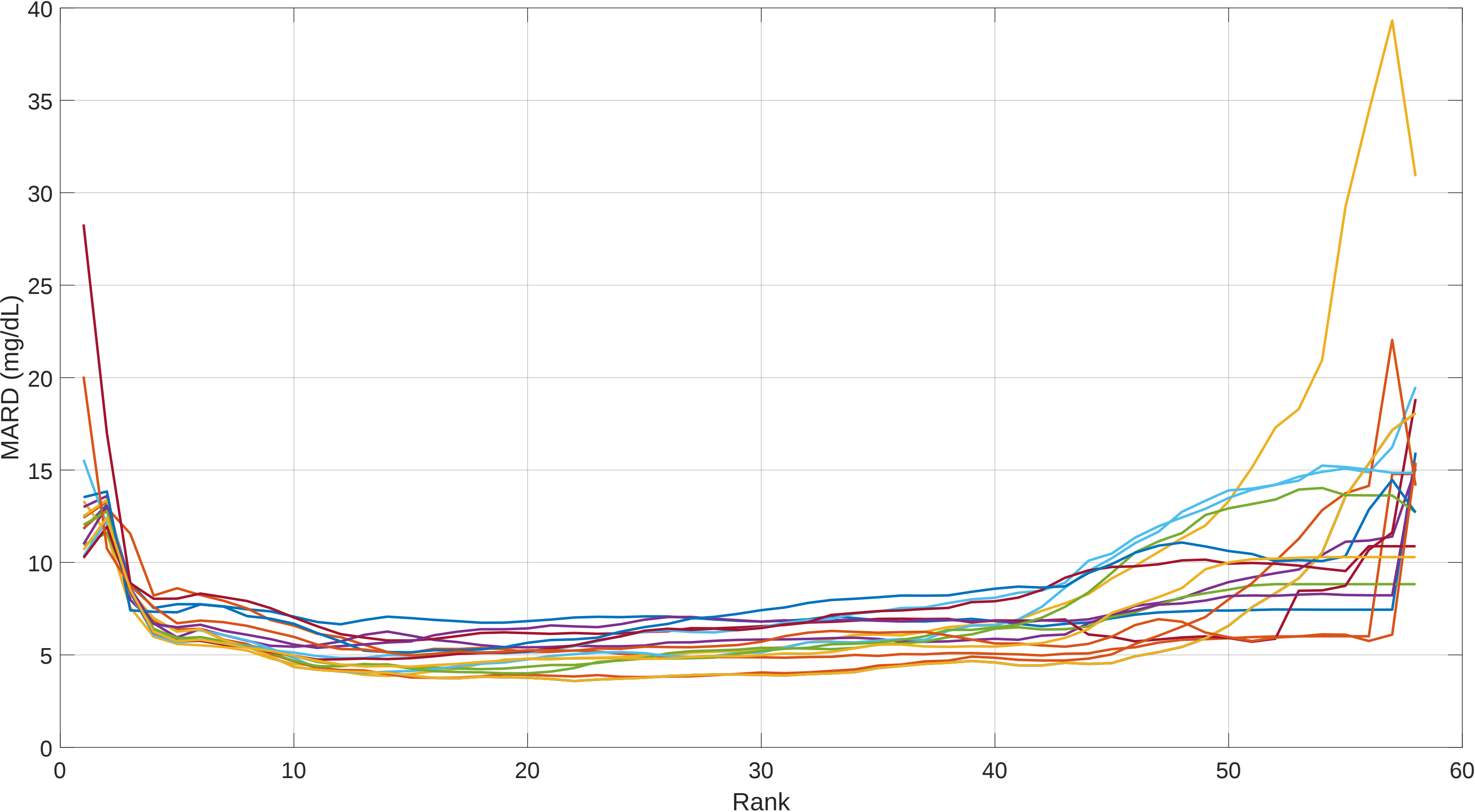
Post Outlier Removed LOOP MARD vs PLS Rank: Session 9 Oxi OLRank 8 PredRank 28
