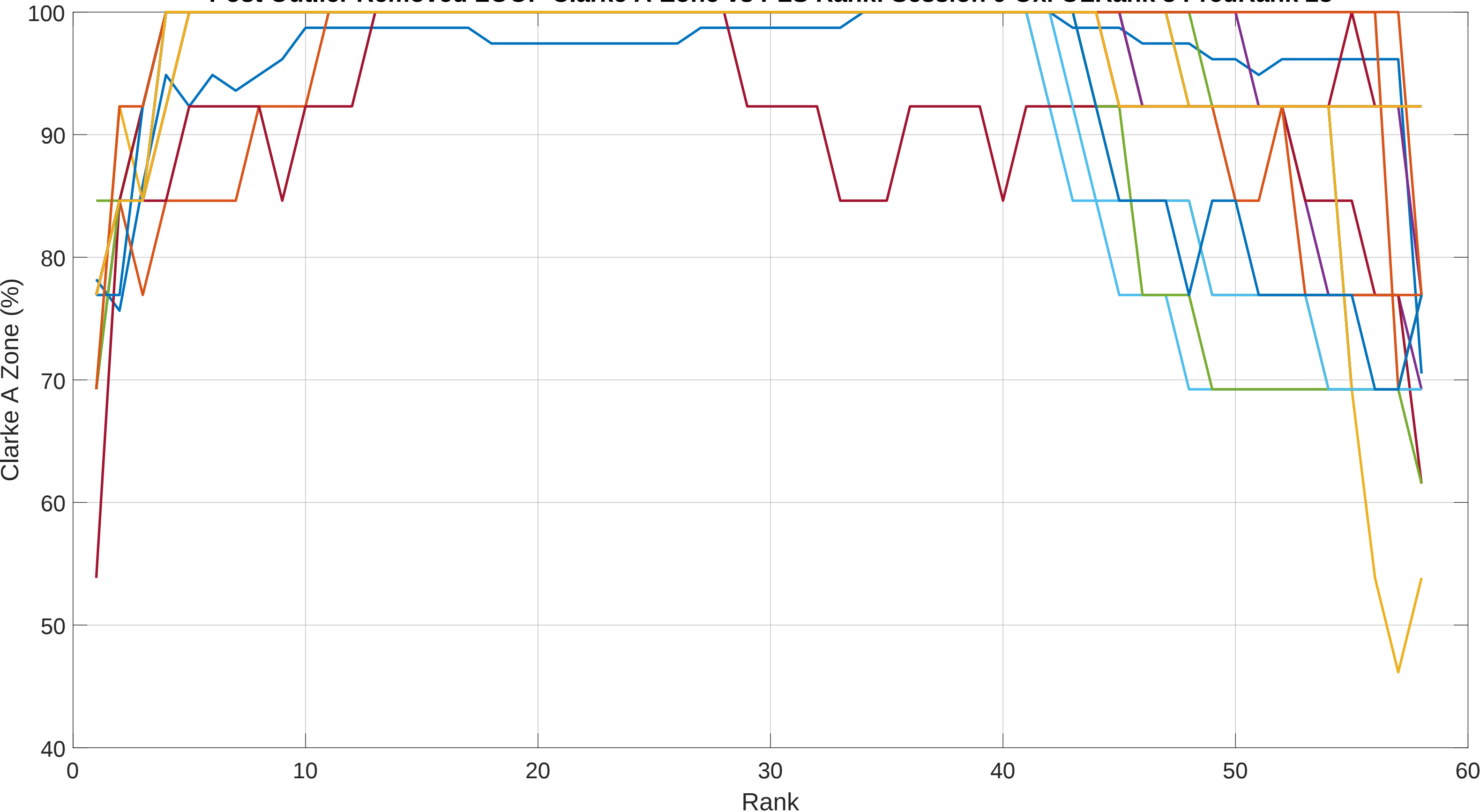
Post Outlier Removed LOOP Clarke A-Zone vs PLS Rank: Session 9 Oxi OLRank 8 PredRank 28
