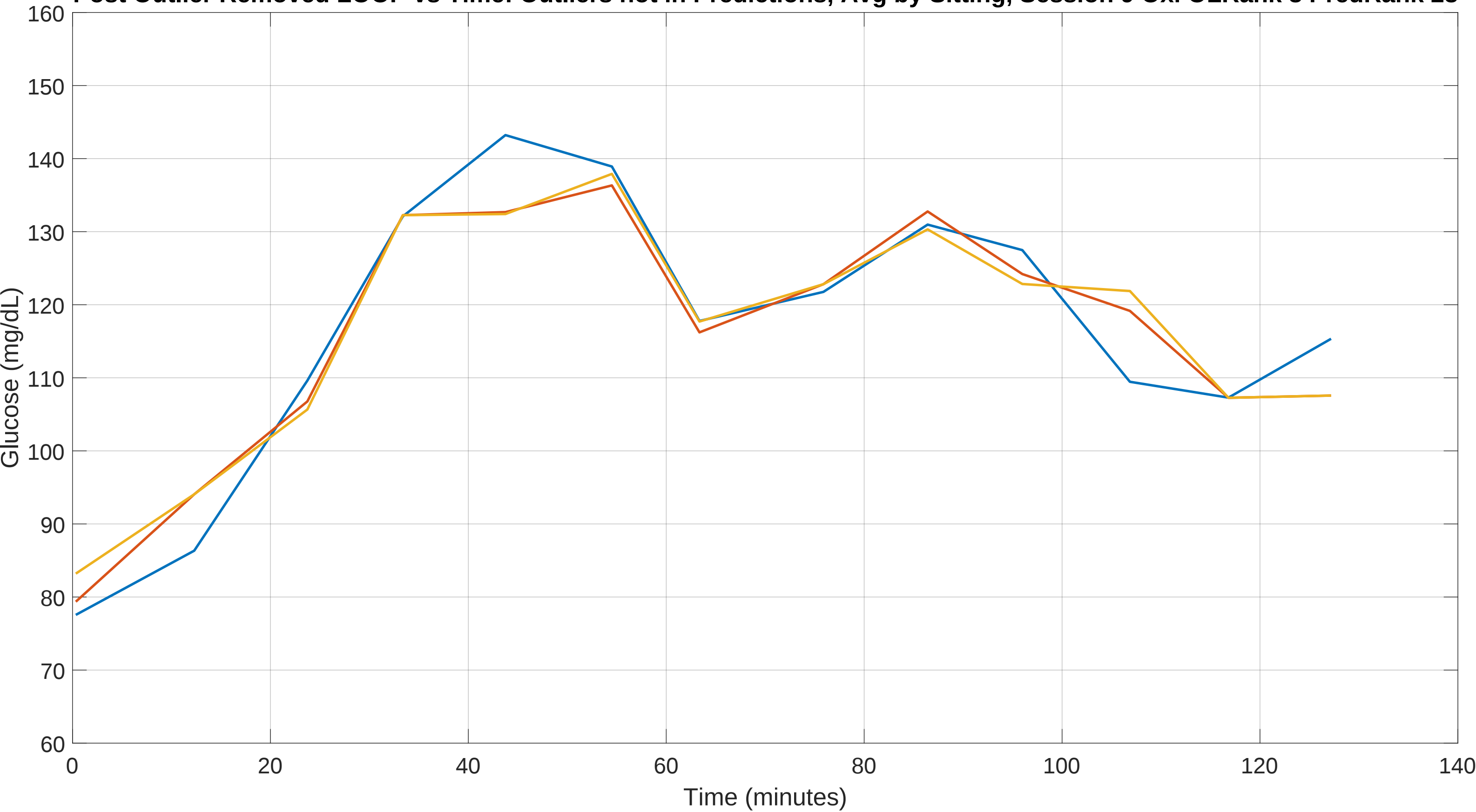
Post Outlier Removed LOOP vs Time: Outliers not in Predictions, Avg by Sitting, Session 9 Oxi OLRank 8 PredRank 28
