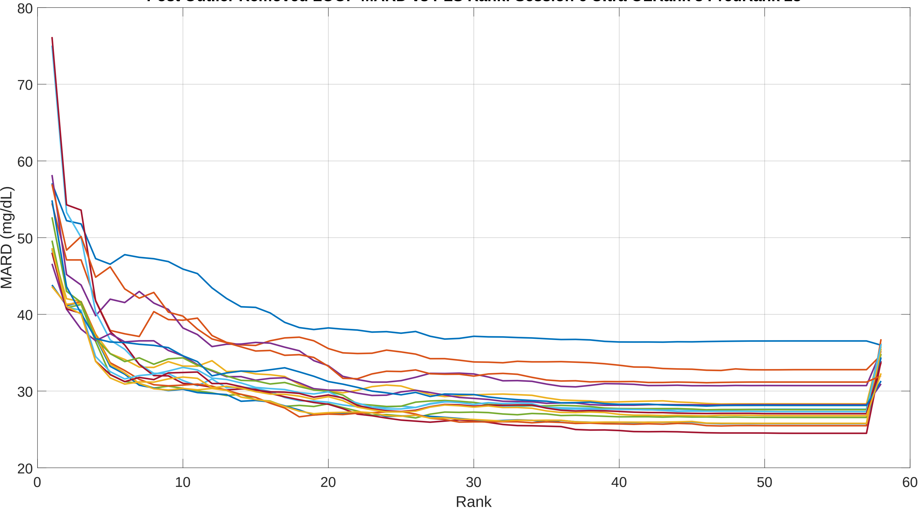
Post Outlier Removed LOOP MARD vs PLS Rank: Session 6 Ultra OLRank 8 PredRank 28
