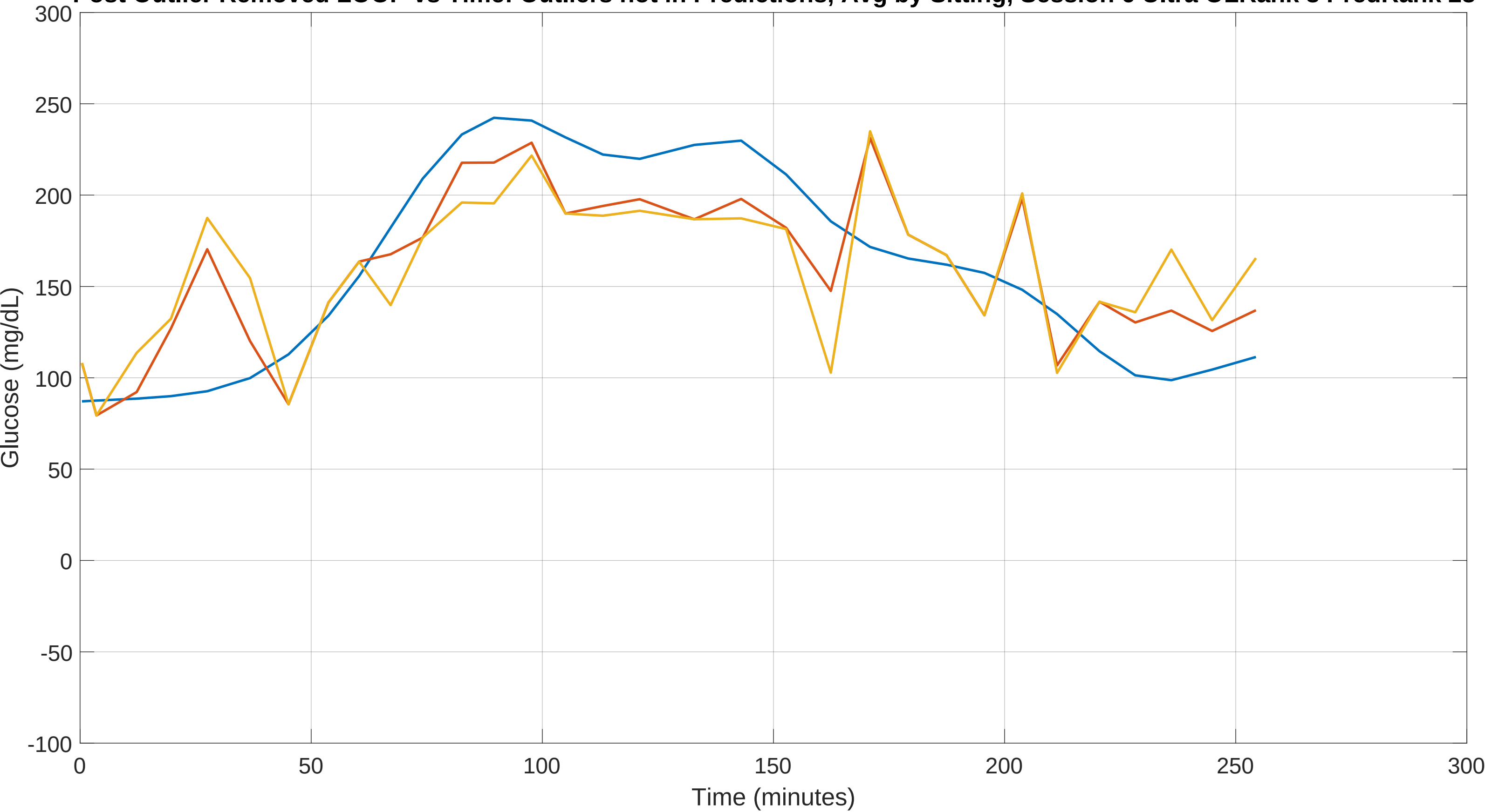
Post Outlier Removed LOOP vs Time: Outliers not in Predictions, Avg by Sitting, Session 6 Ultra OLRank 8 PredRank 28
