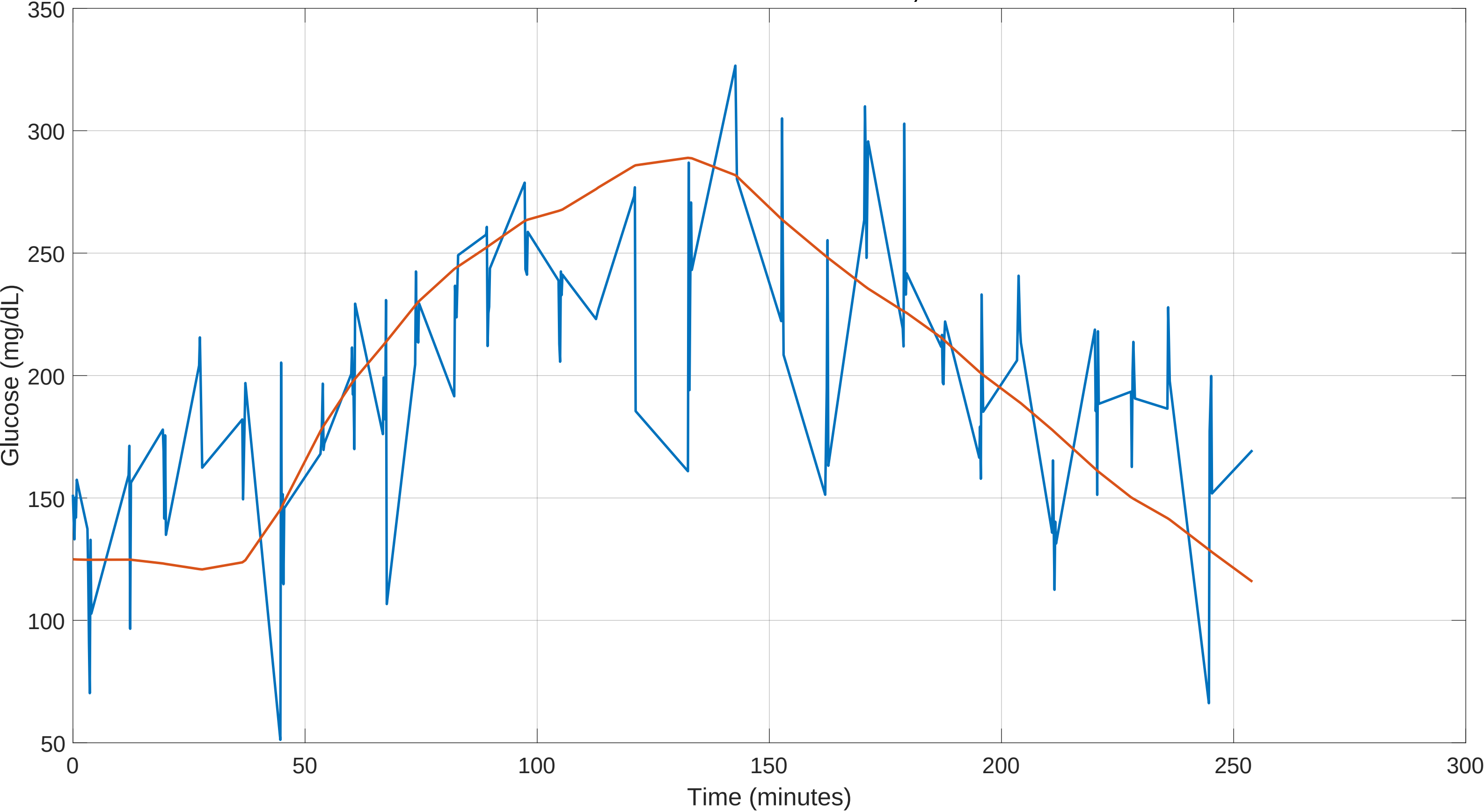
Post Outlier Removed LOOP vs Time: Outliers not in Predictions, Session 6 CGM OLRank 8 PredRank 28
