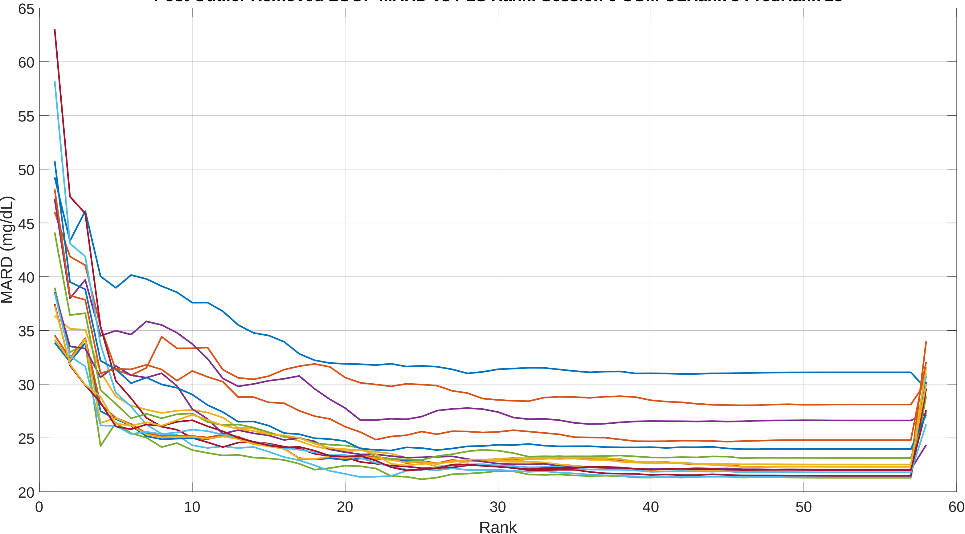
Post Outlier Removed LOOP MARD vs PLS Rank: Session 6 CGM OLRank 8 PredRank 28
