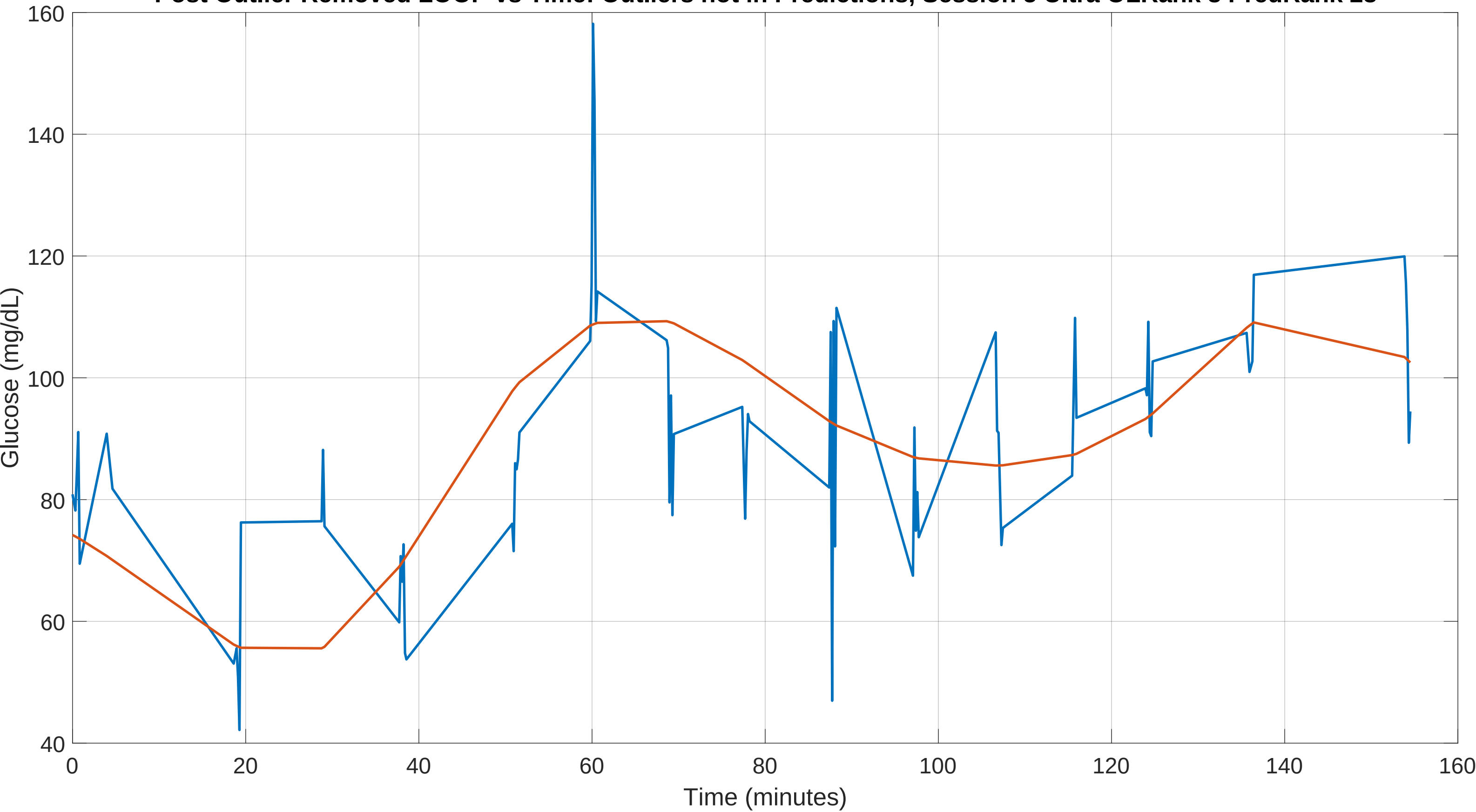
Post Outlier Removed LOOP vs Time: Outliers not in Predictions, Session 5 Ultra OLRank 8 PredRank 28
