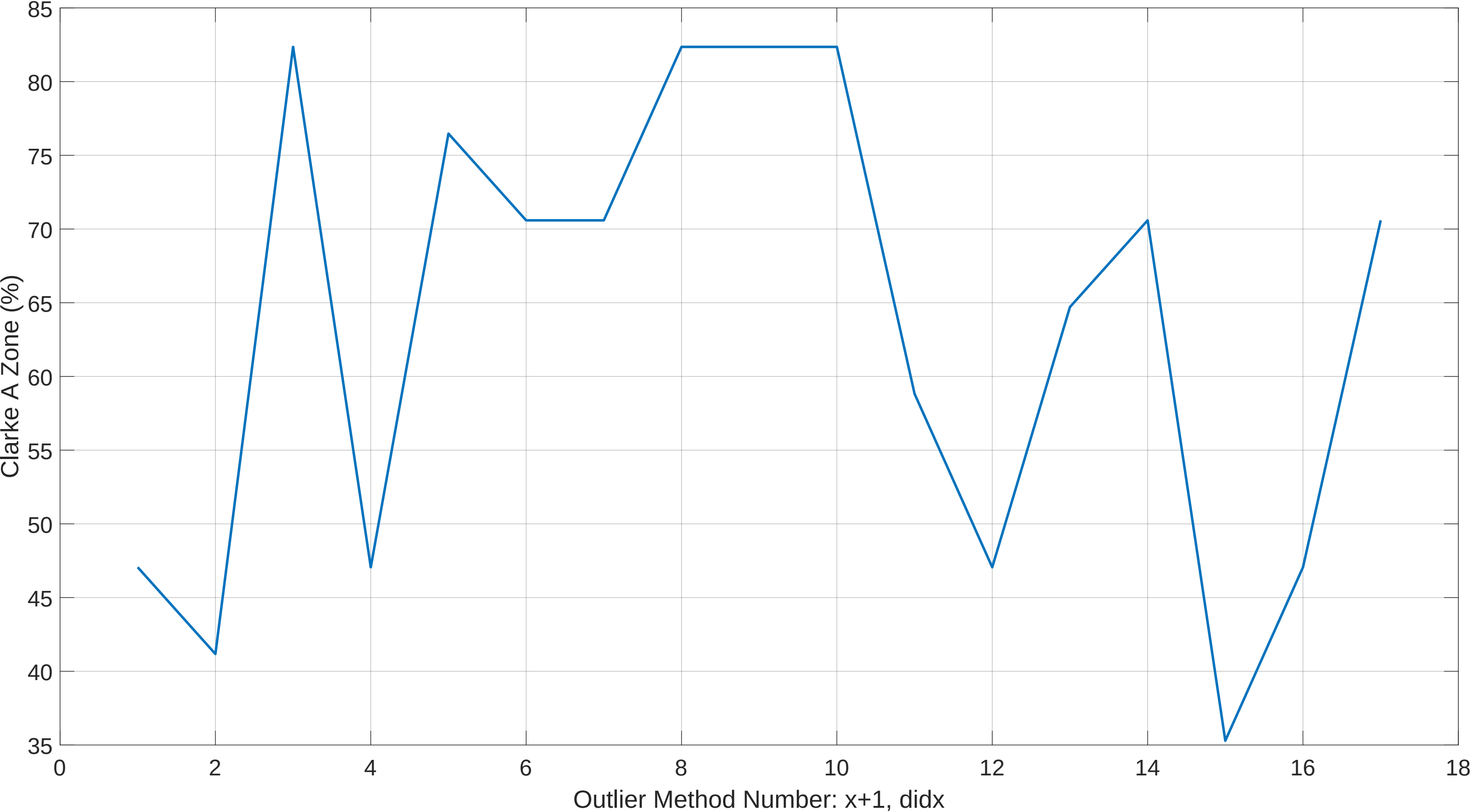
Post Outlier Removed LOOP Clarke A-Zone vs Outlier Method #: Session 5 Ultra OLRank 8 PredRank 28
