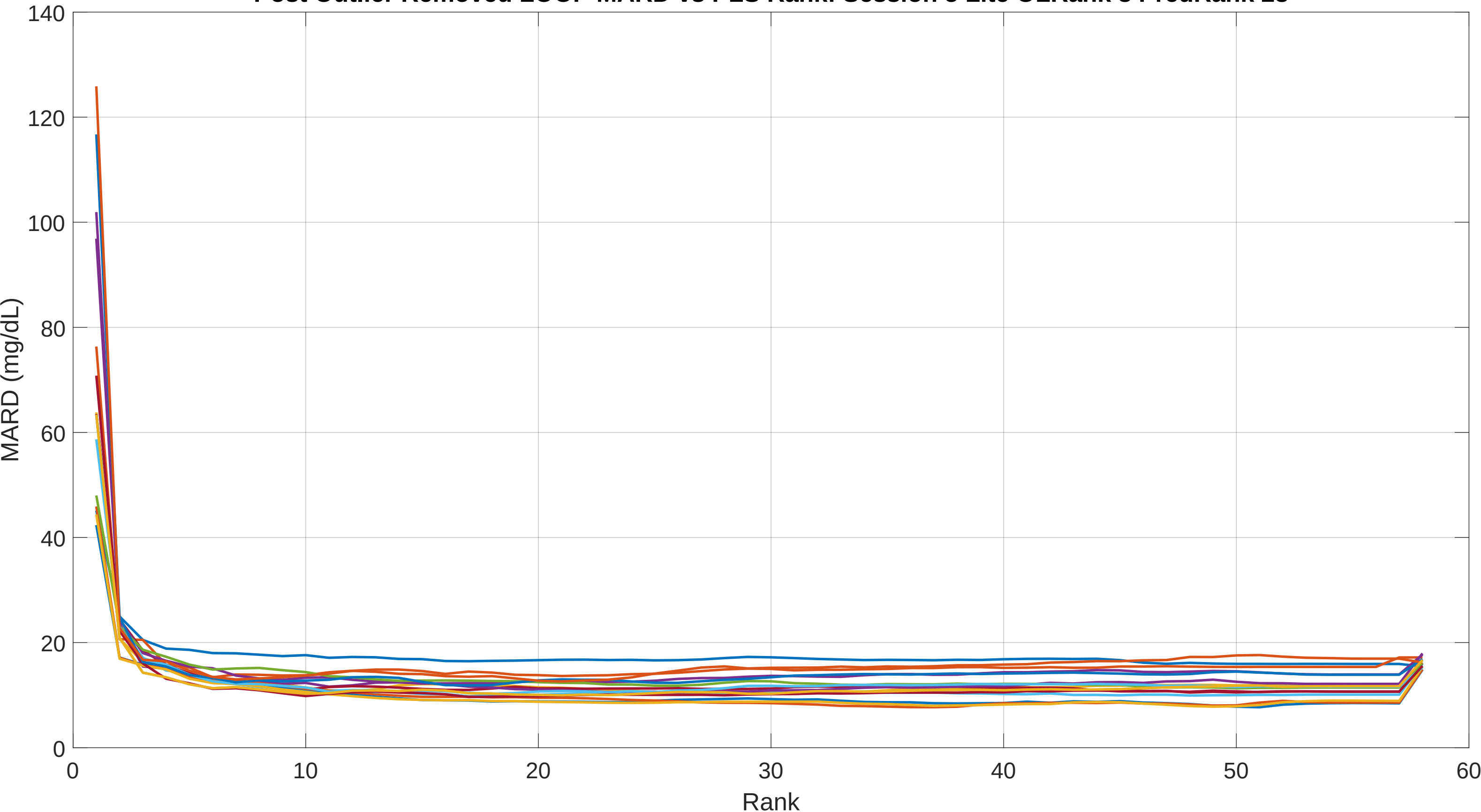
Post Outlier Removed LOOP MARD vs PLS Rank: Session 5 Lite OLRank 8 PredRank 28
