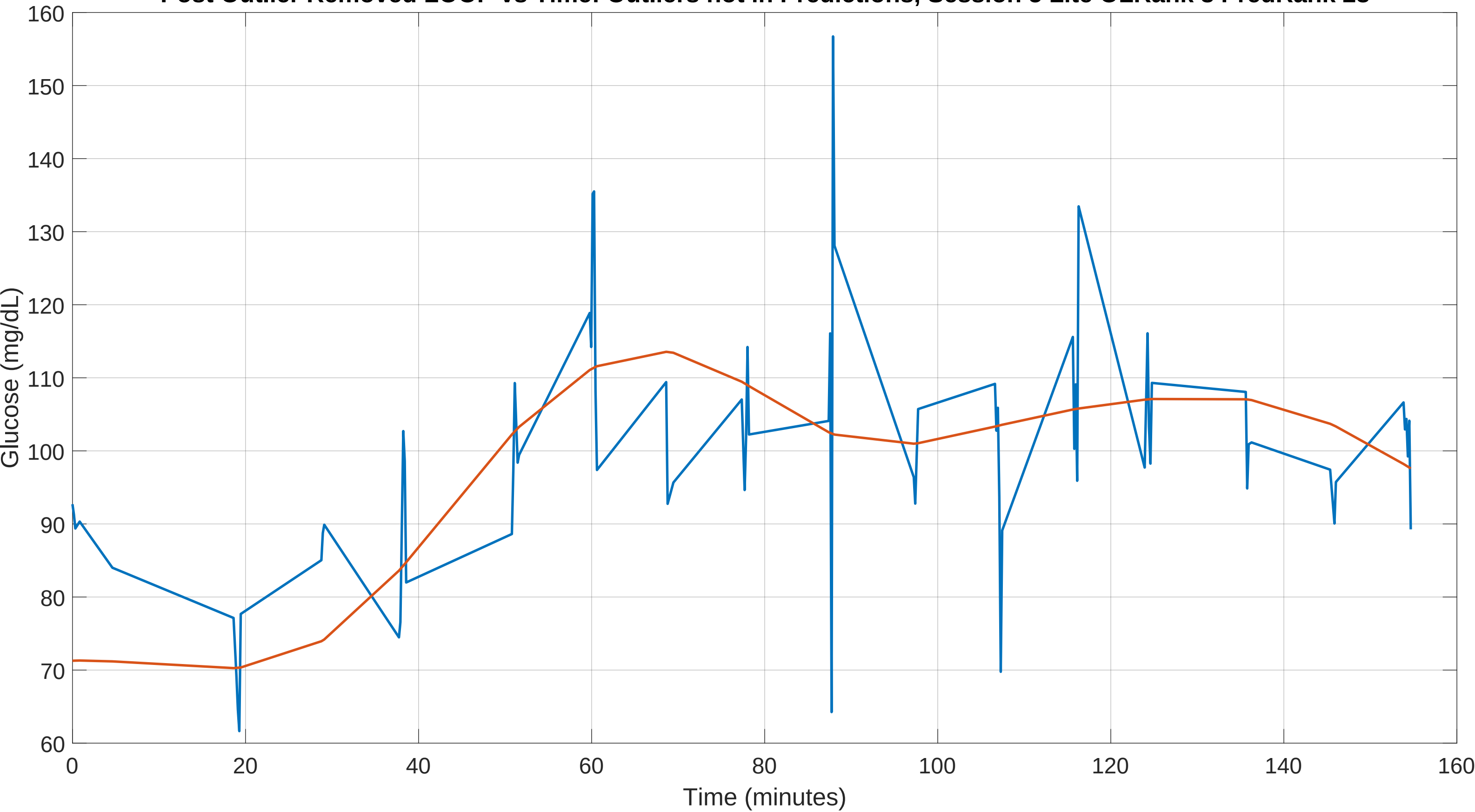
Post Outlier Removed LOOP vs Time: Outliers not in Predictions, Session 5 Lite OLRank 8PredRank 28
