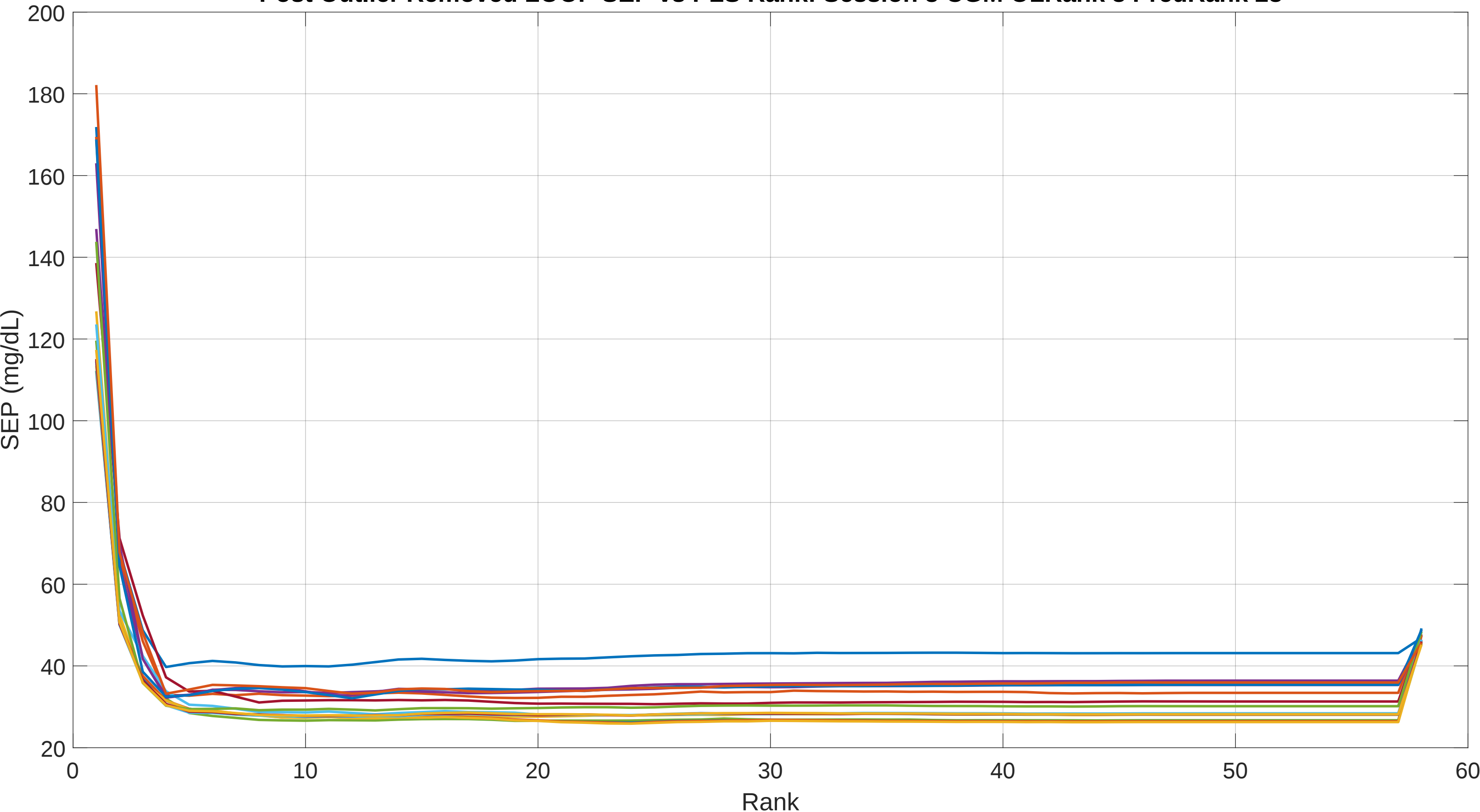
Post Outlier Removed LOOP SEP vs PLS Rank: Session 3 CGM OLRank 8 PredRank 28
