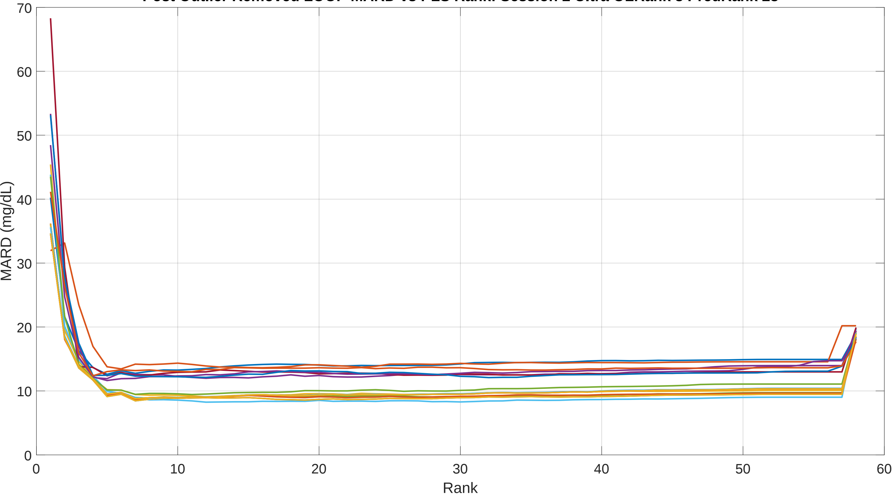
Post Outlier Removed LOOP MARD vs PLS Rank: Session 2 Ultra OLRank 8 PredRank 28
