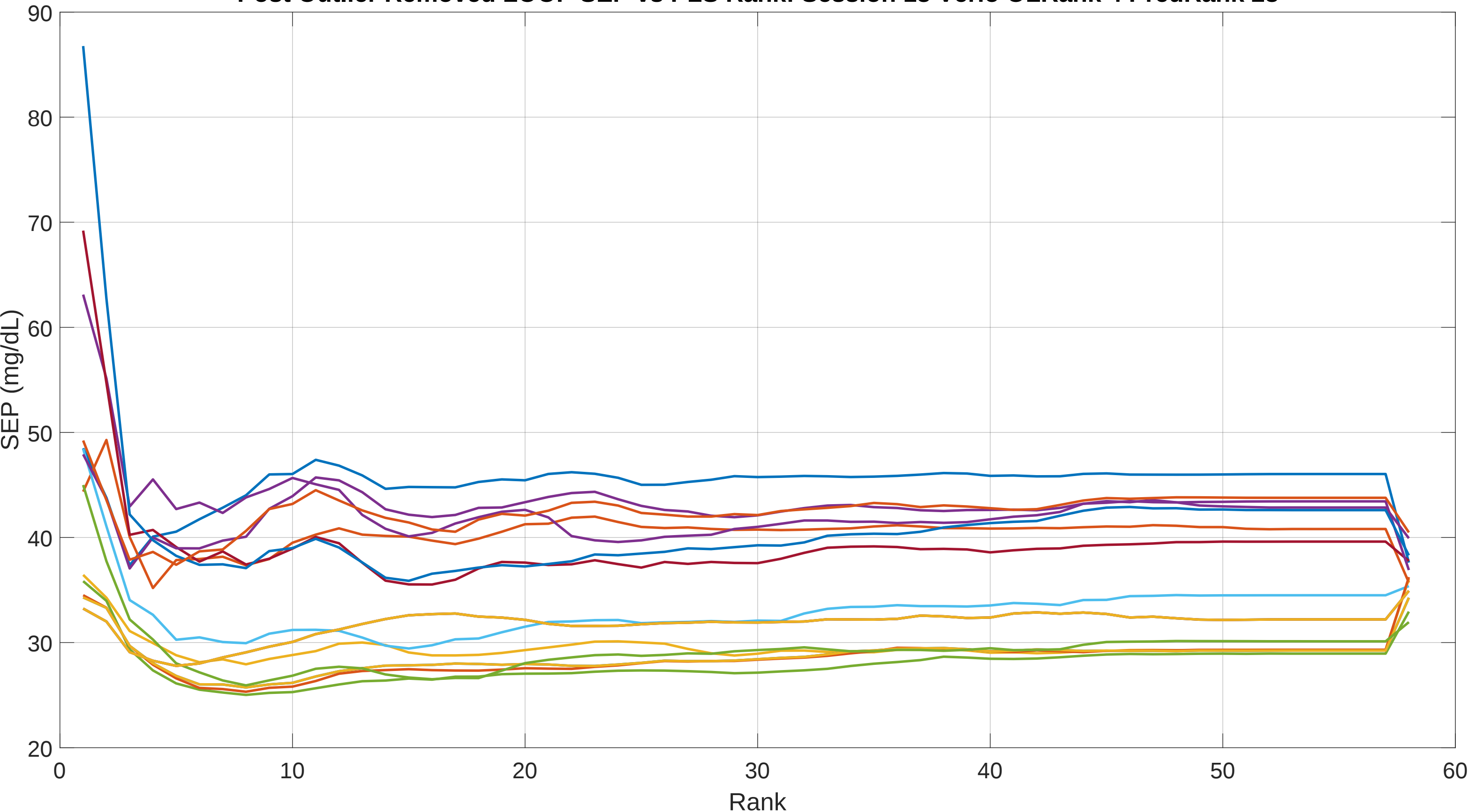
Post Outlier Removed LOOP SEP vs PLS Rank: Session 13 Verio OLRank 4 PredRank 28
