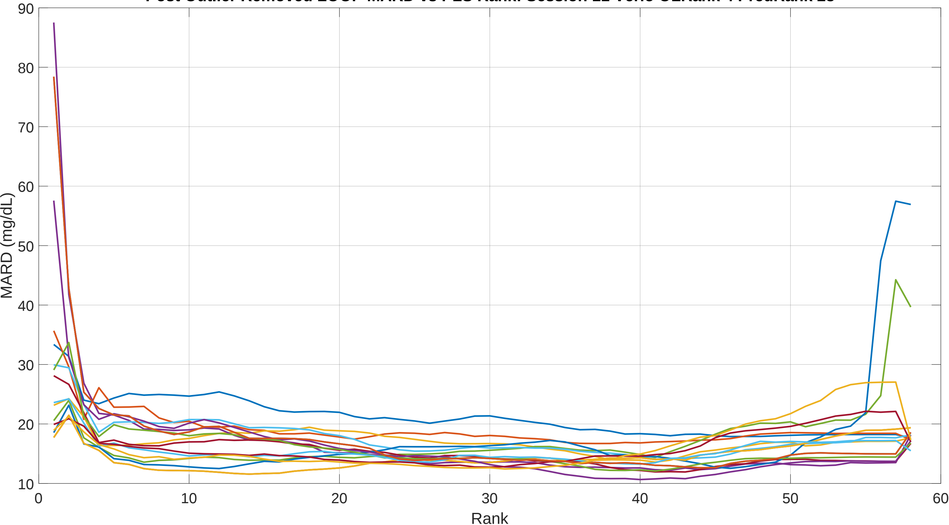
Post Outlier Removed LOOP MARD vs PLS Rank: Session 11 Verio OLRank 4 PredRank 28
