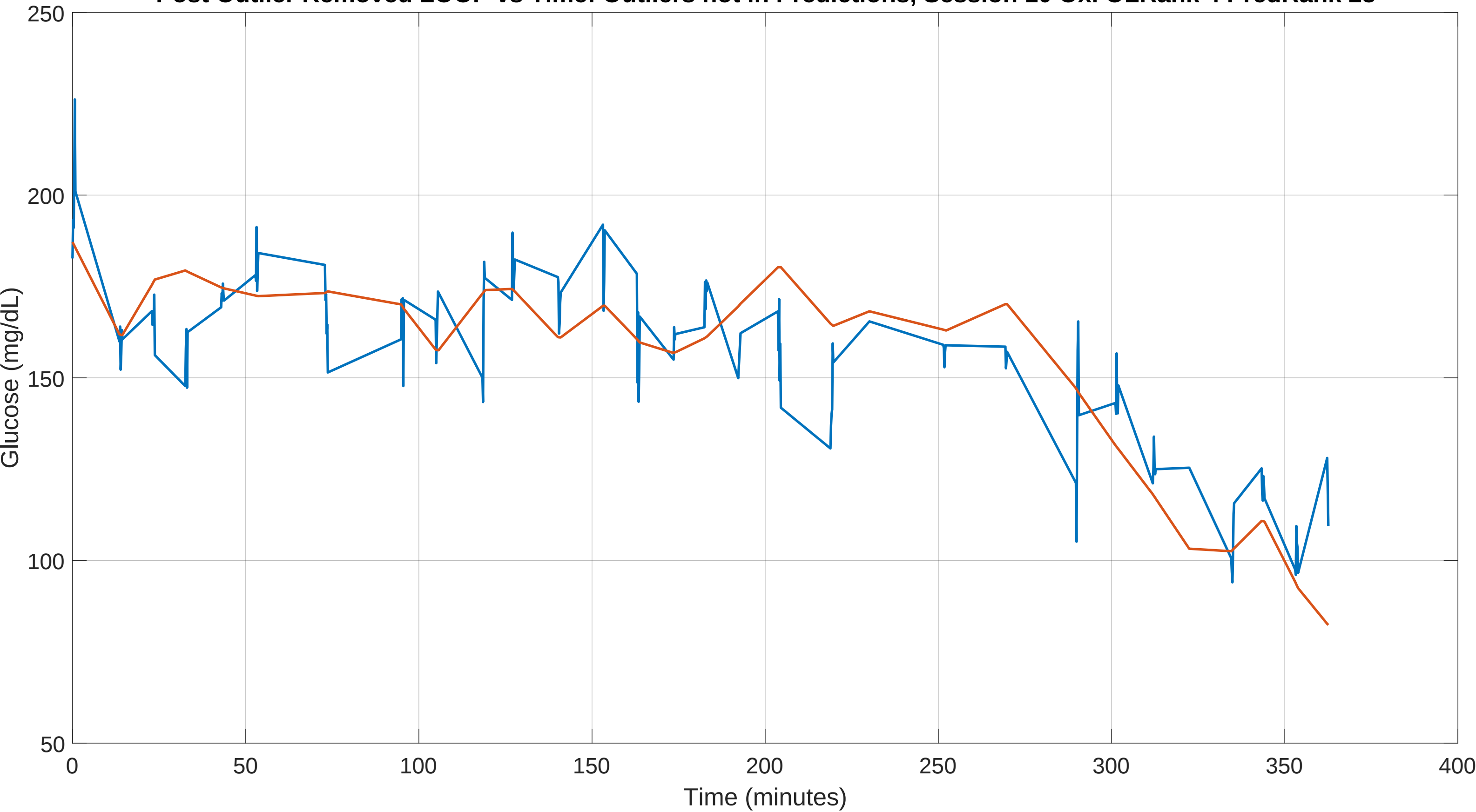
Post Outlier Removed LOOP vs Time: Outliers not in Predictions, Session 10 Oxi OLRank 4 PredRank 28
