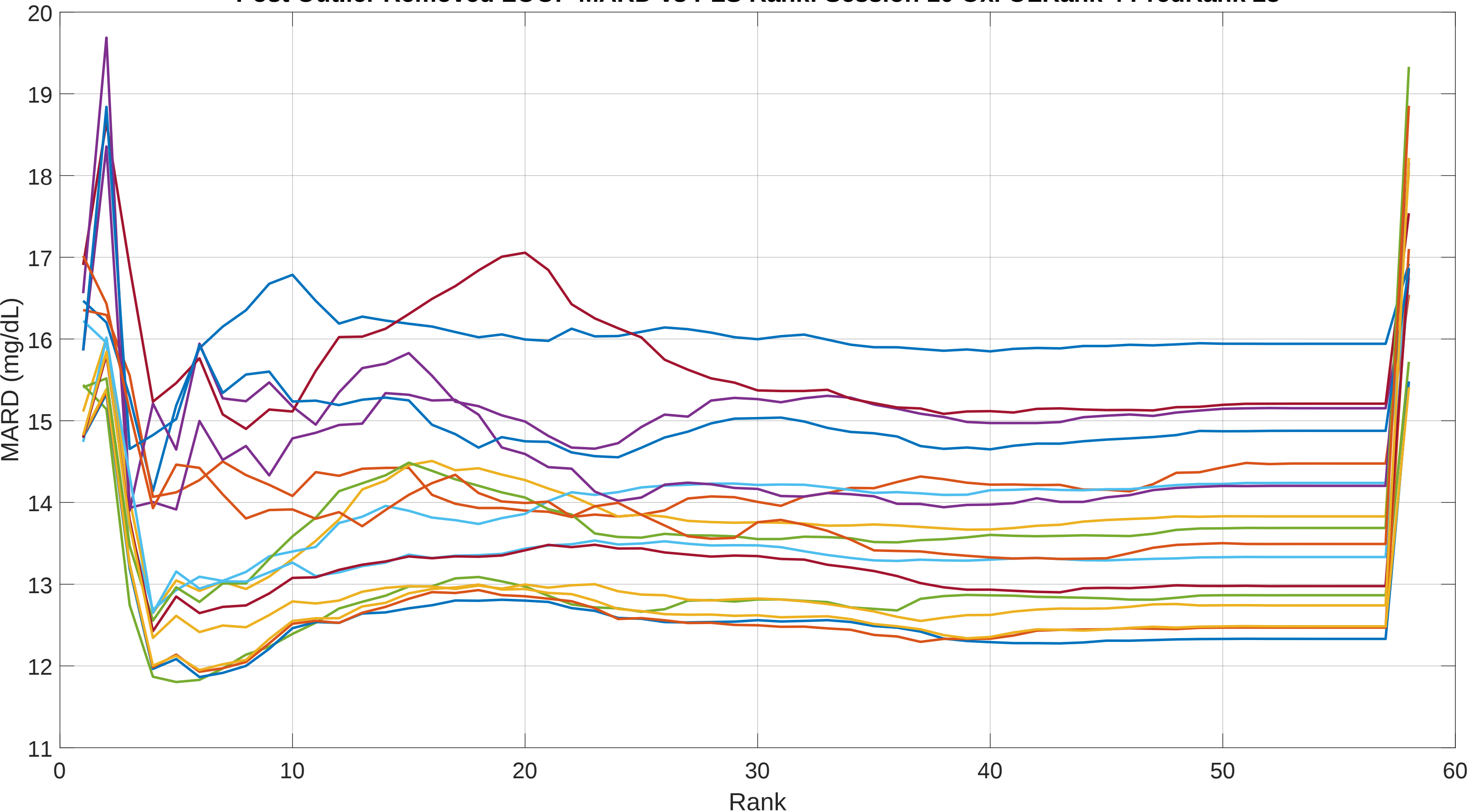
Post Outlier Removed LOOP MARD vs PLSRank: Session 10 Oxi OLRank 4 PredRank 28
