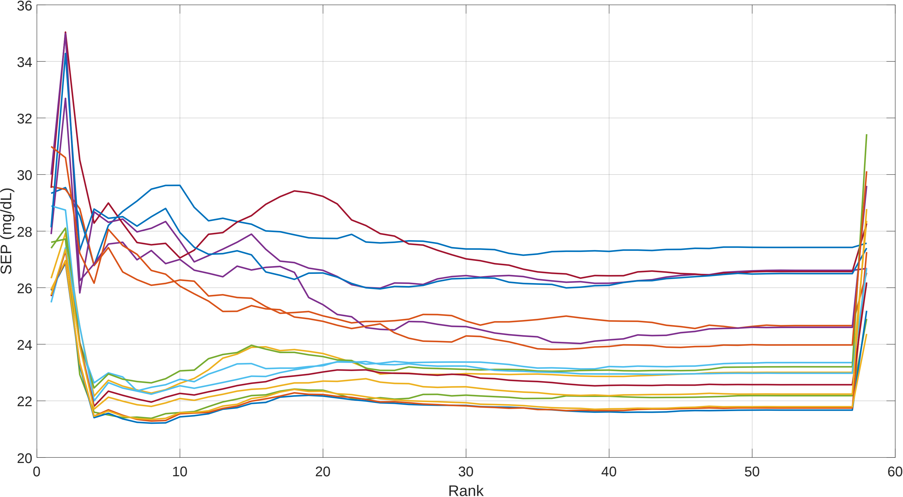
Post Outlier Removed LOOP SEP vs PLS Rank: Session 10 Oxi OLRank 4 PredRank 28
