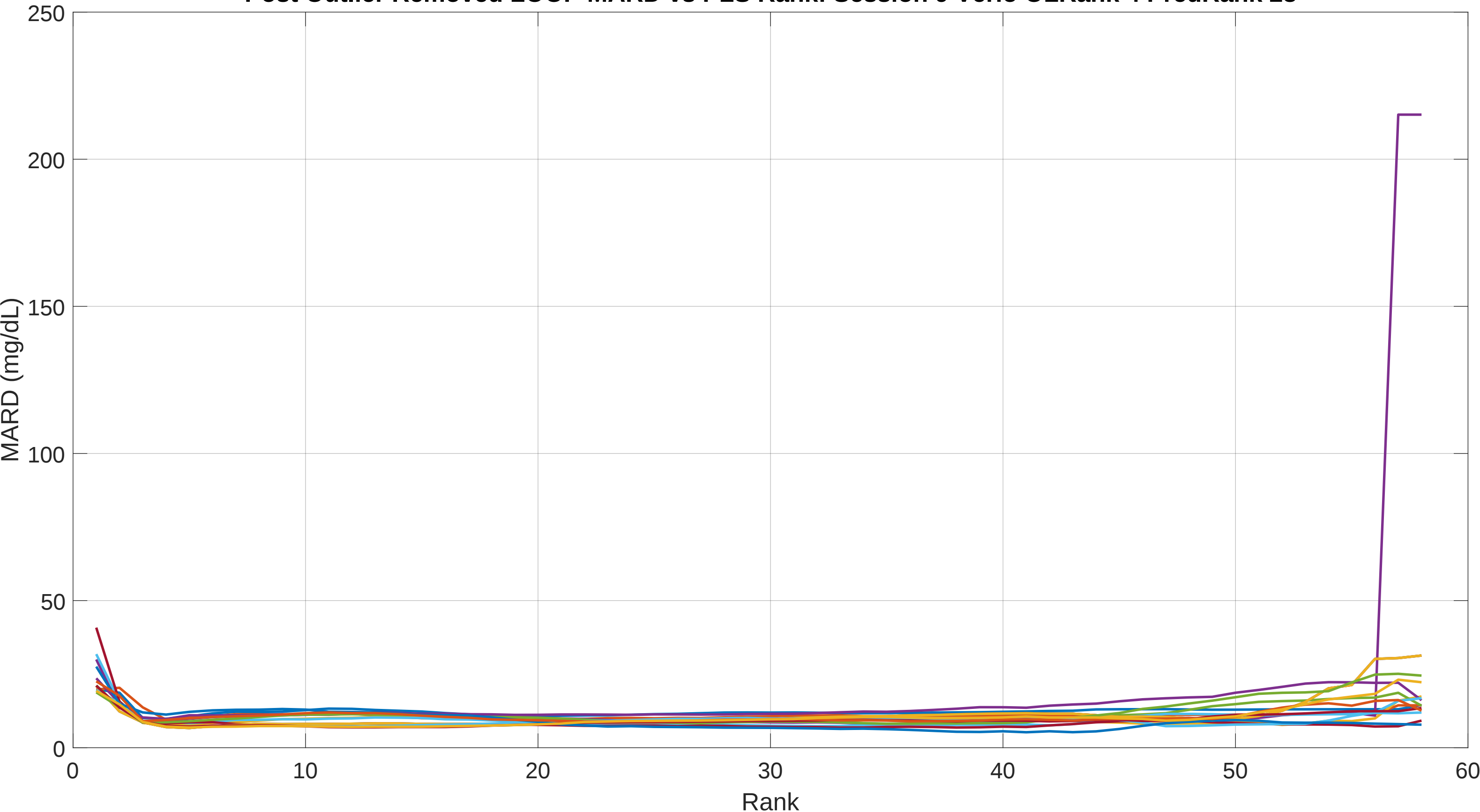
Post Outlier Removed LOOP MARD vs PLS Rank: Session 9 Verio OLRank 4 PredRank 28
